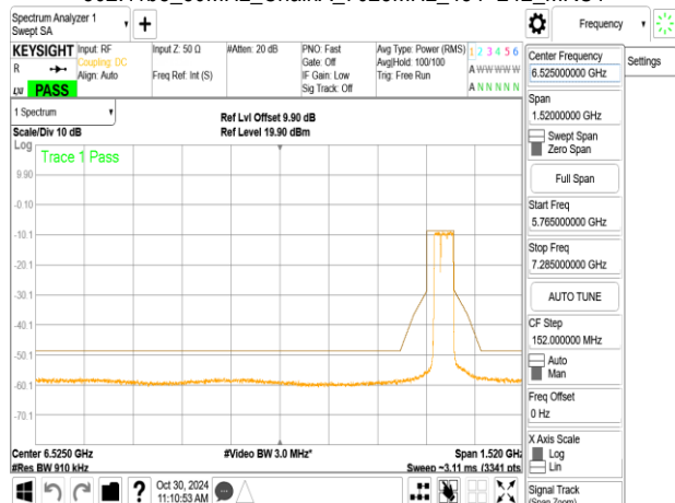
802.11be_80MHz_ChainA_7025MHz_484+242_MR1
