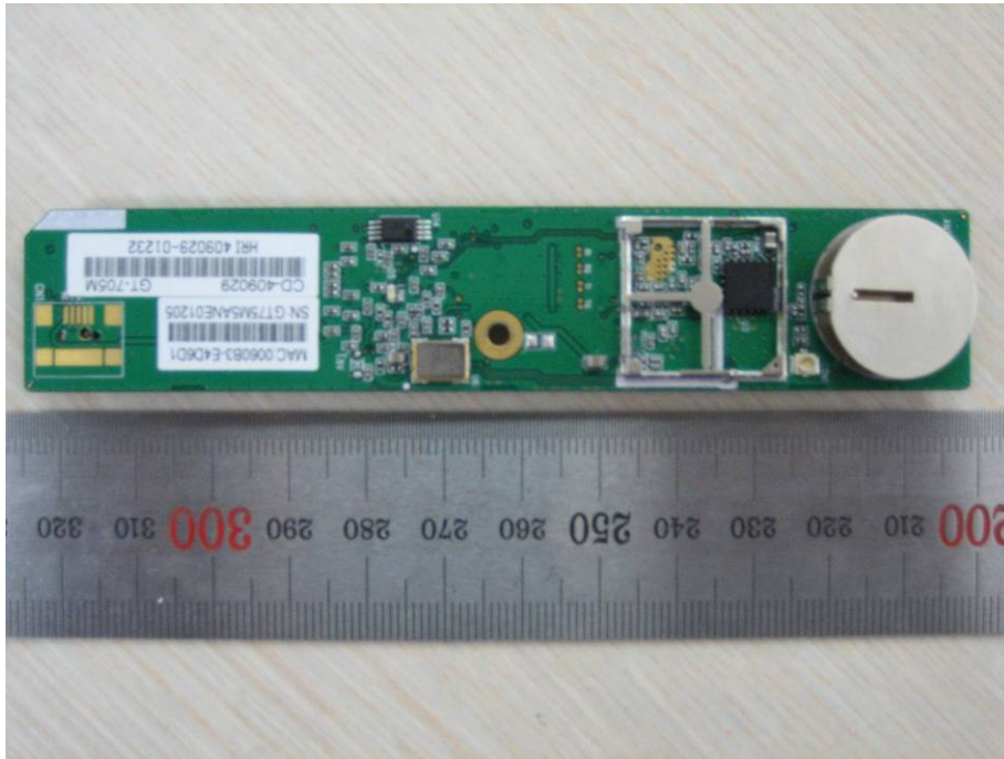
EUT- Taiwan RF module Top View
