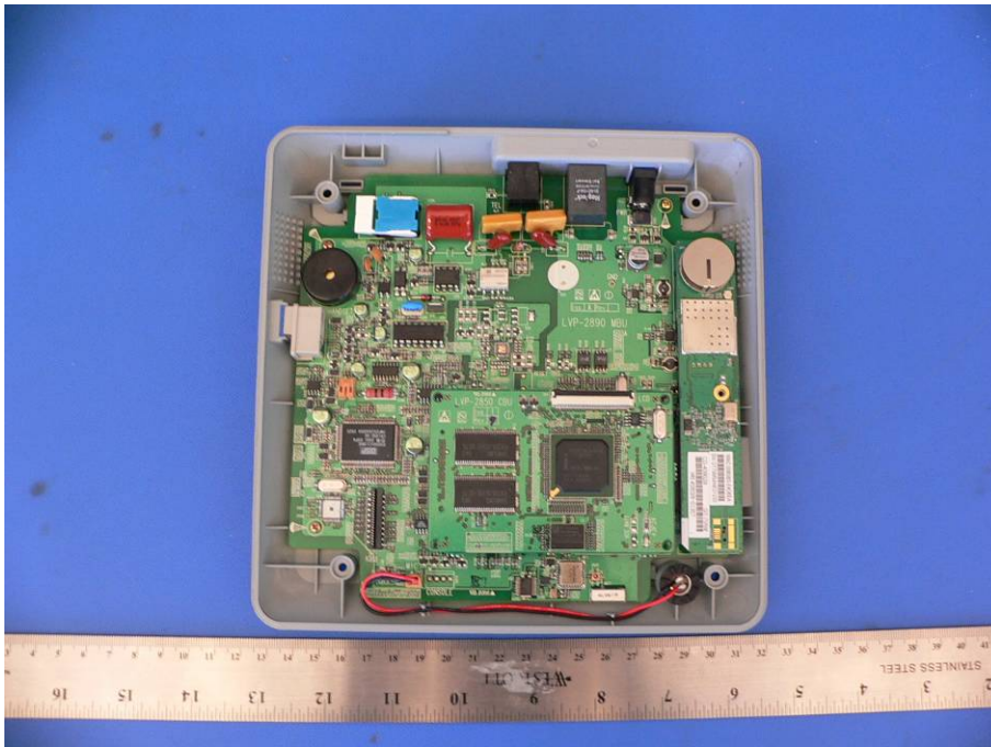
EUT- Chassis off with Taiwan RF Module View
