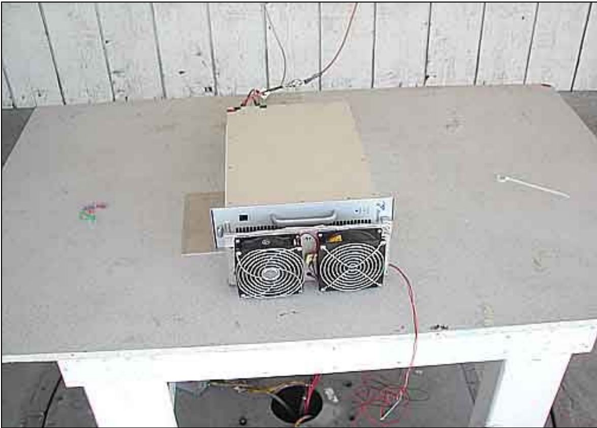
Radiated Emissions - Front View
