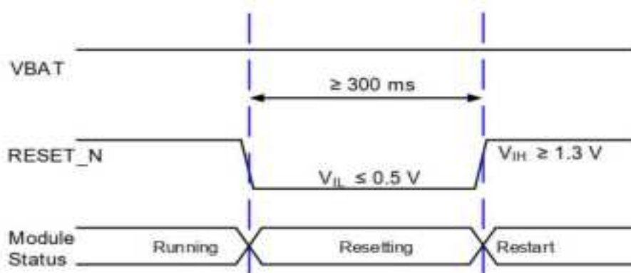
Figure 3-10: Reset Timing
