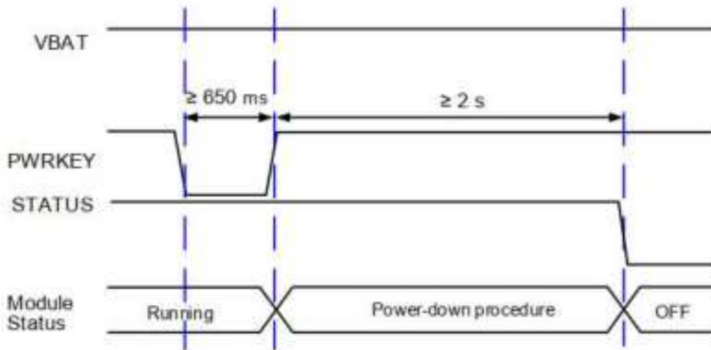
Figure 3-7: Power-down Timing
