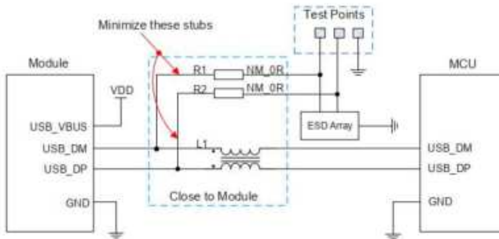
Figure 4-1: Reference Circuit of USB Application
