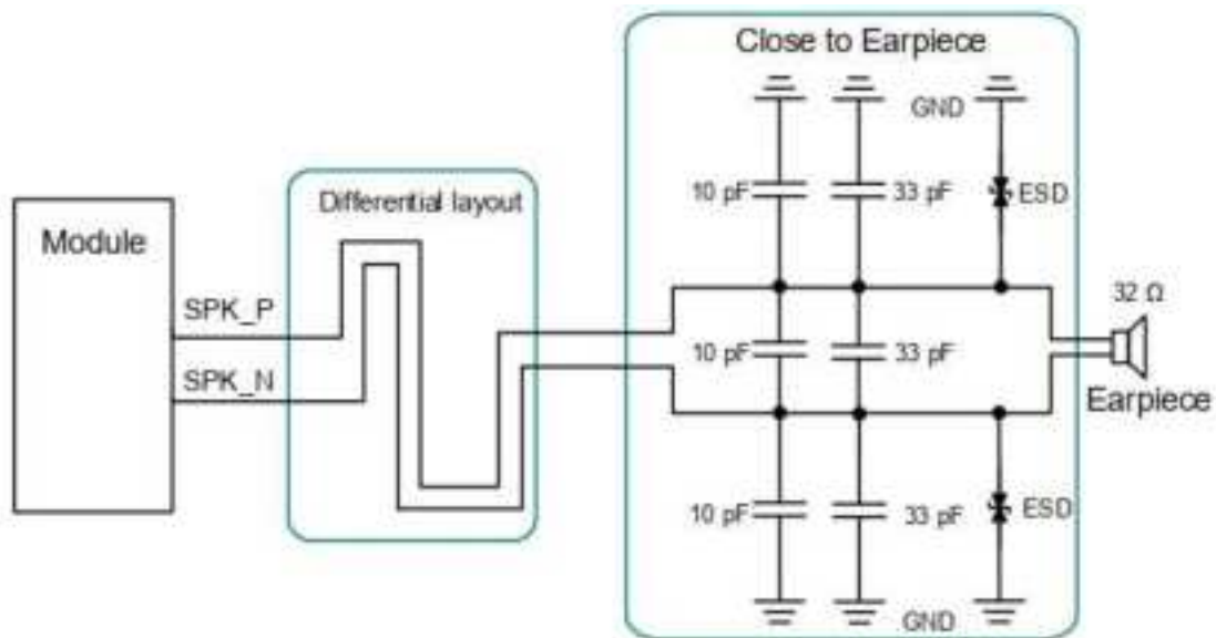
Figure 4-8: Reference Design for Loudspeaker Interface
