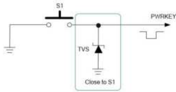
Figure 3-5: Turing on the Module Using Button
