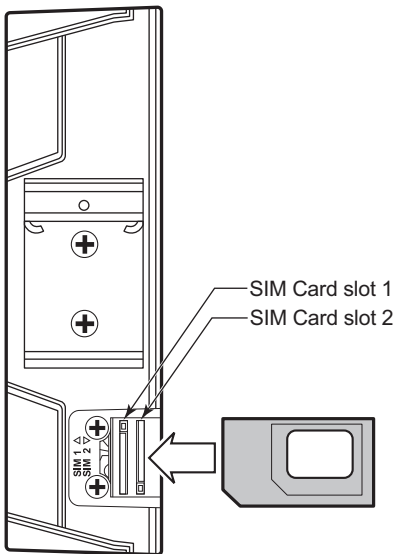
Figure 13 SIM Slots and Orientation on a 7705 SAR-Hmc
