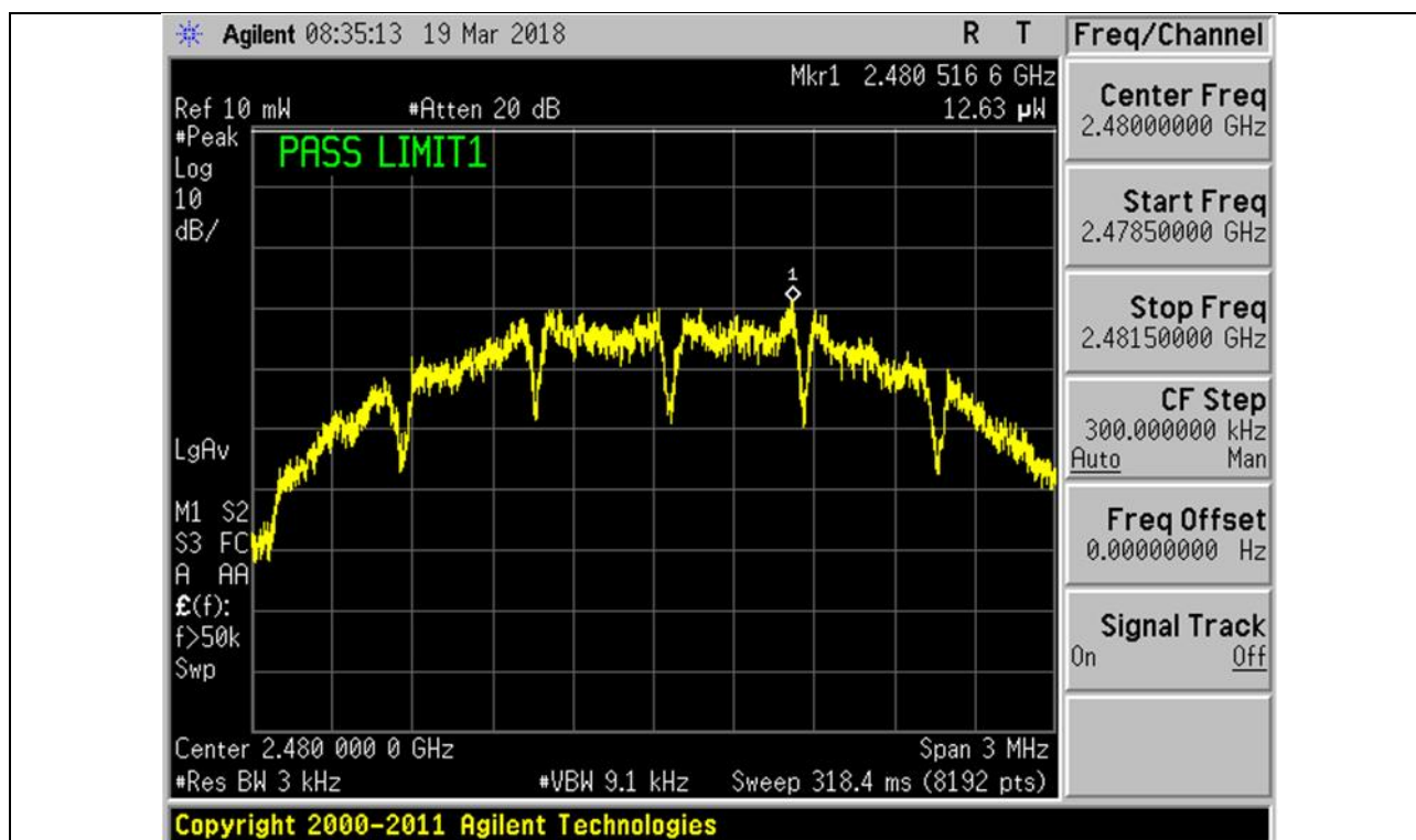
Plot 50 – Upper Channel
