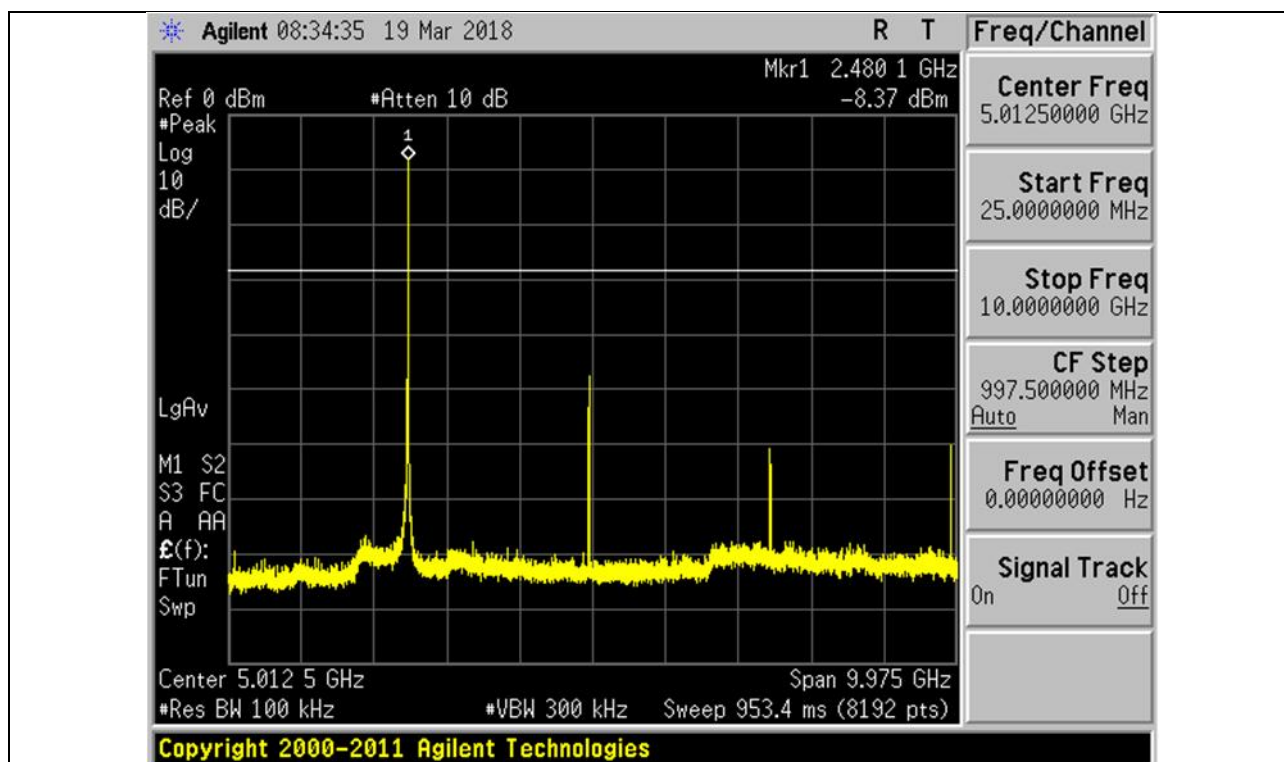
Plot 11 – Upper Channel
