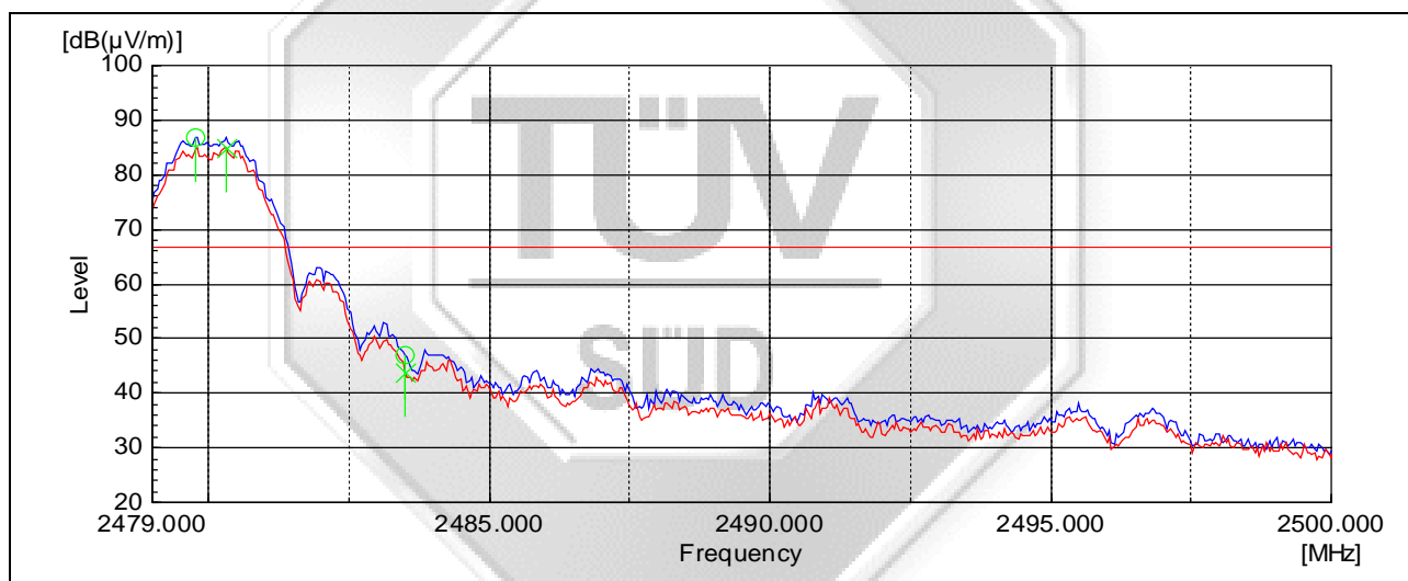
Plot 43 – Upper Band Edge at 2.4835GHz
