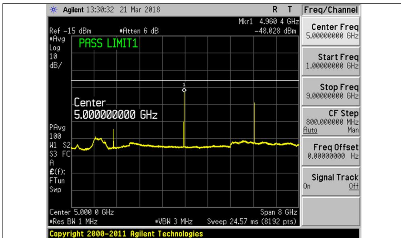
Plot 37 – Upper Channel
