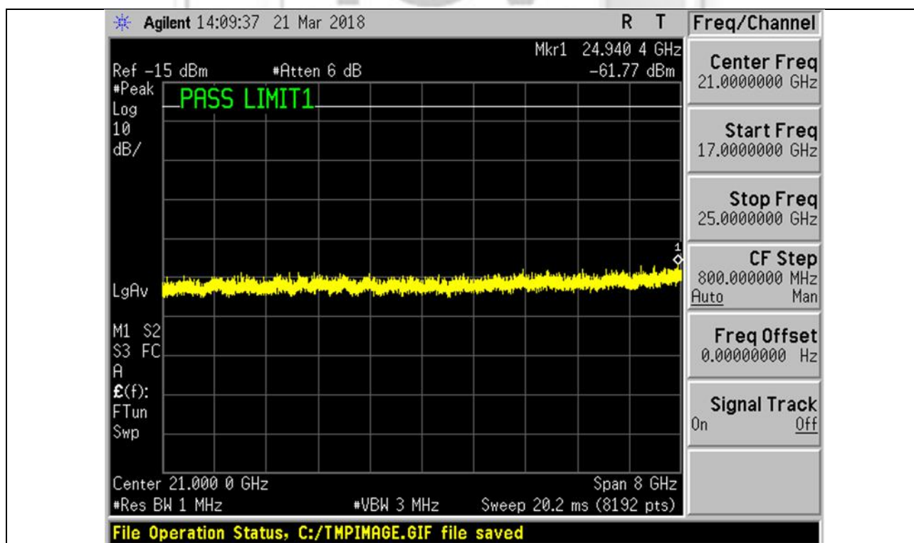
Plot 18 – Lower Channel
