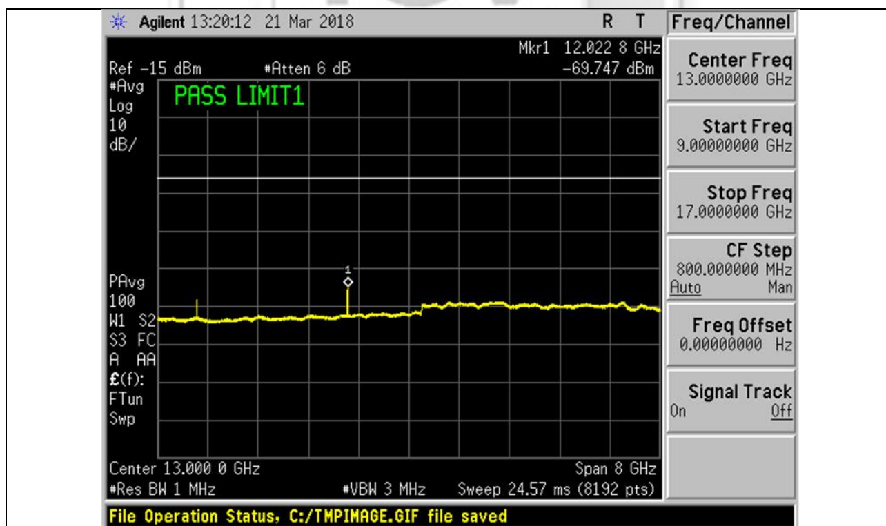
Plot 32 – Lower Channel
