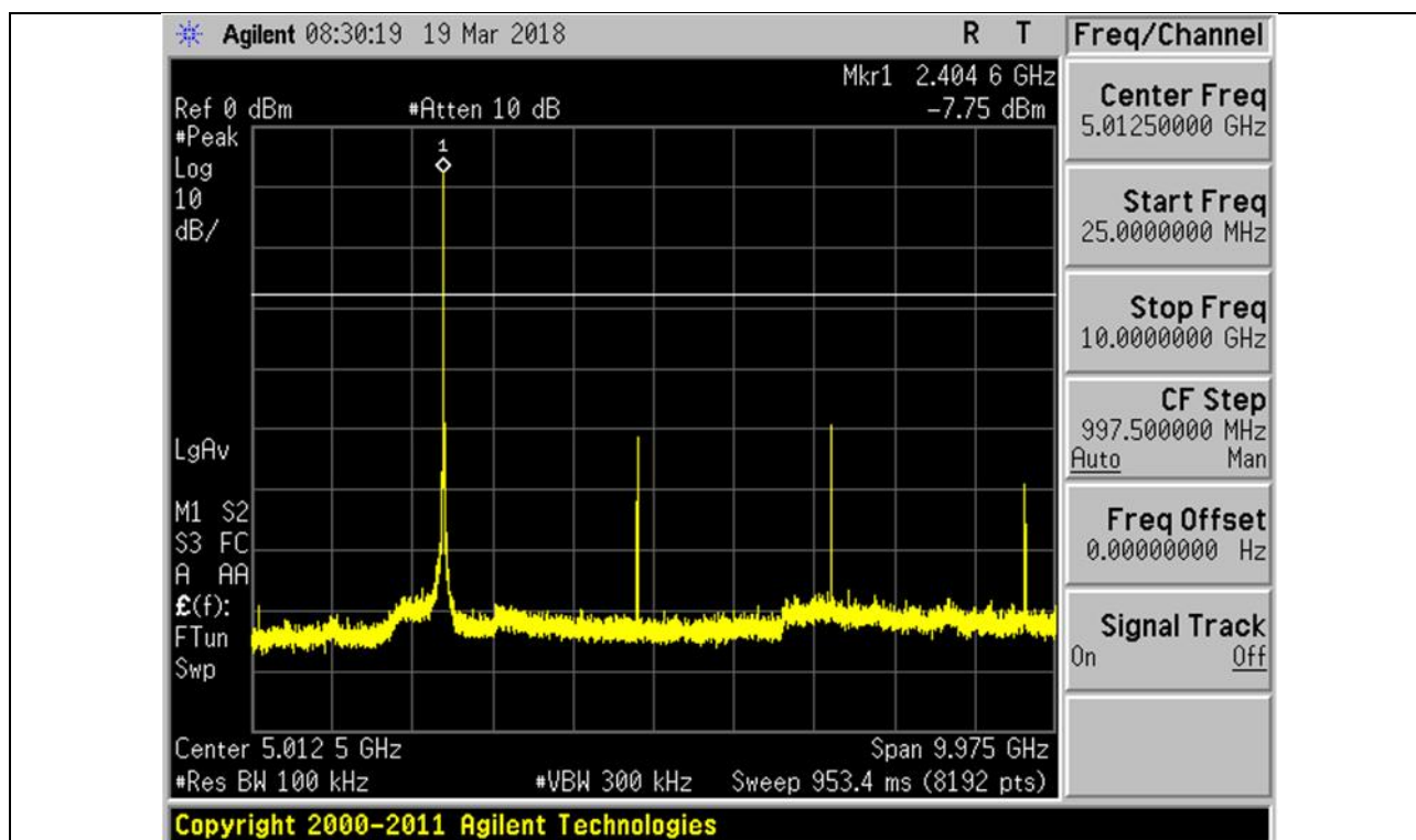
Plot 7 – Lower Channel
