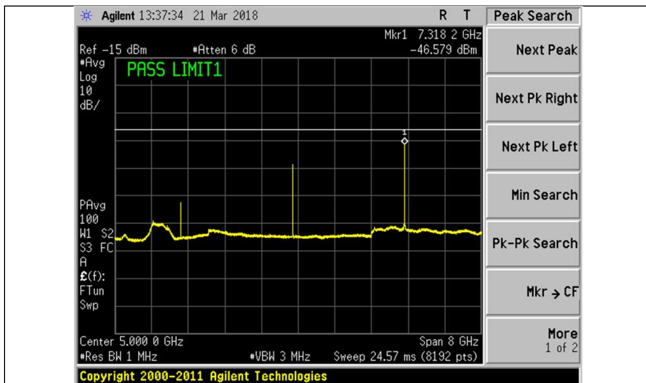
Plot 34 – Middle Channel
