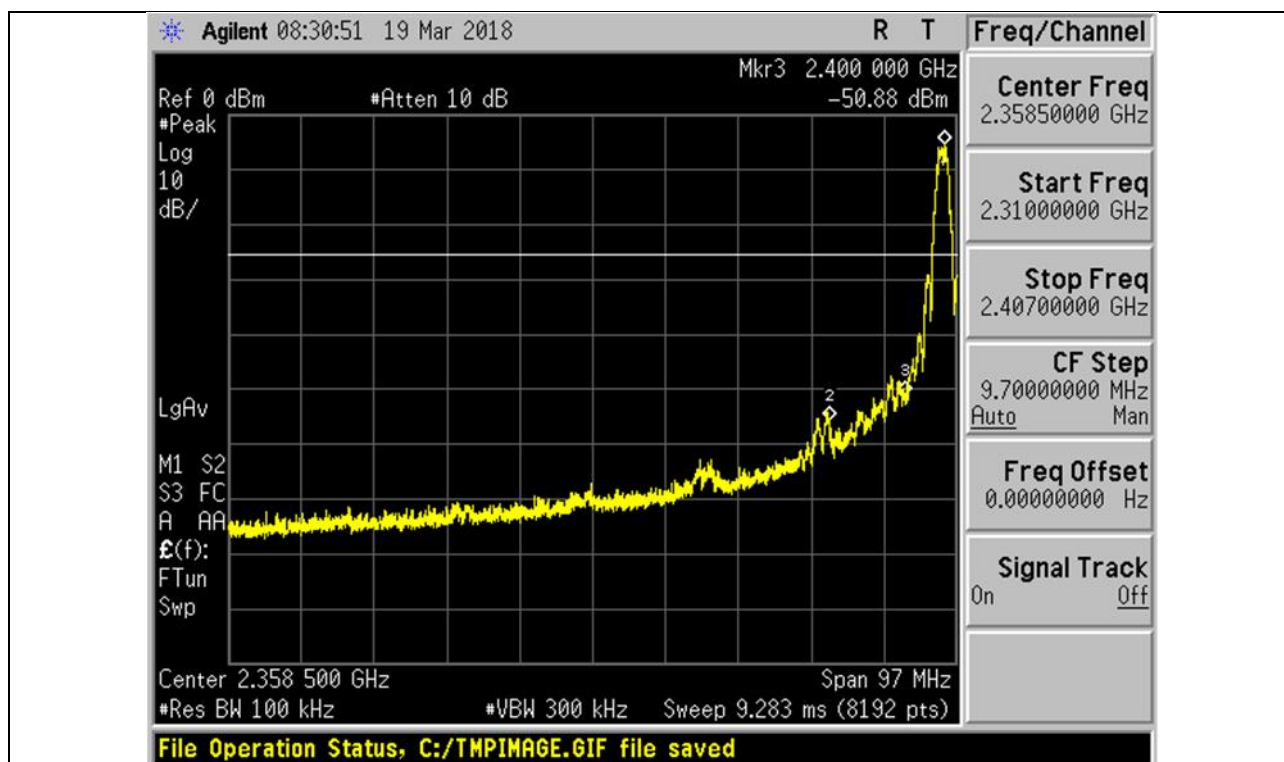
Plot 40 – Lower Band Edge at 2.4000GHz
