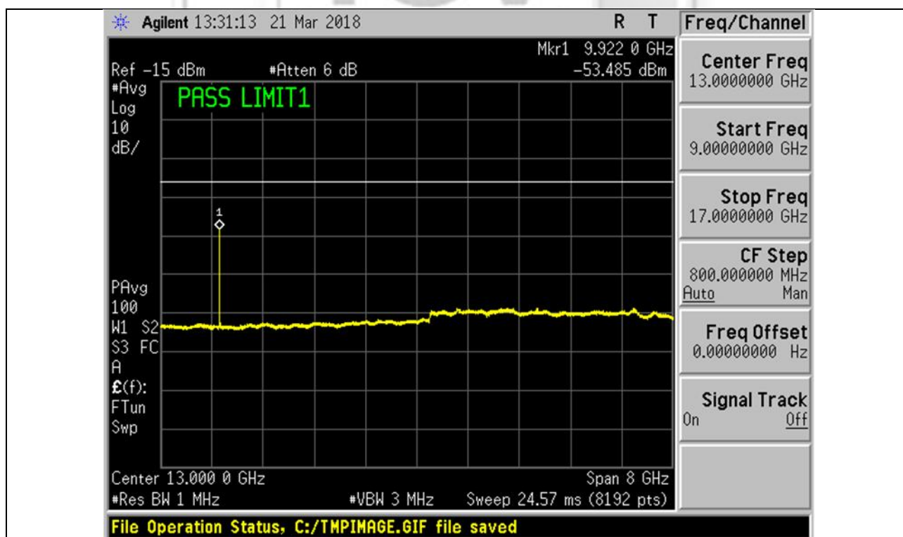
Plot 38 – Upper Channel
