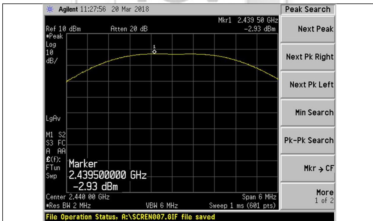
Plot 5 – Middle Channel
