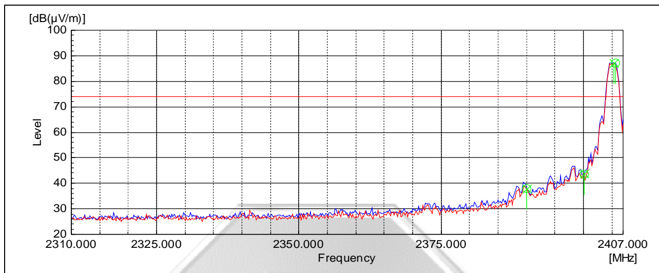
Plot 42 – Lower Band Edge at 2.4000GHz
