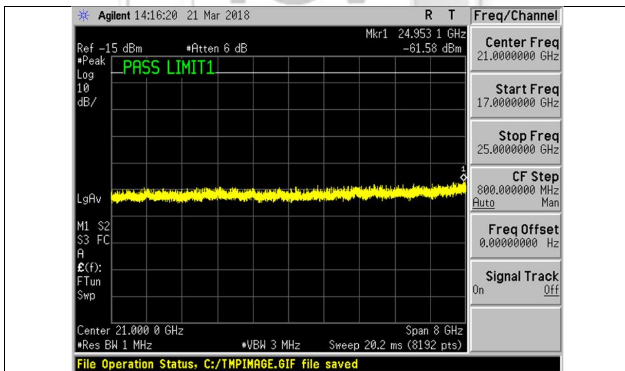
Plot 24 – Middle Channel
