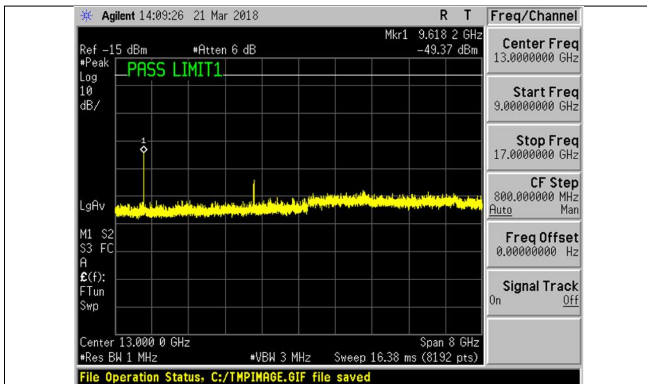
Plot 17 – Lower Channel
