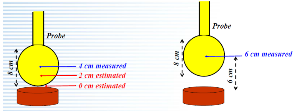
Example of probe measurements in points close to the device surface: estimates compared with measurements at 4 and 6 cm provide validation
