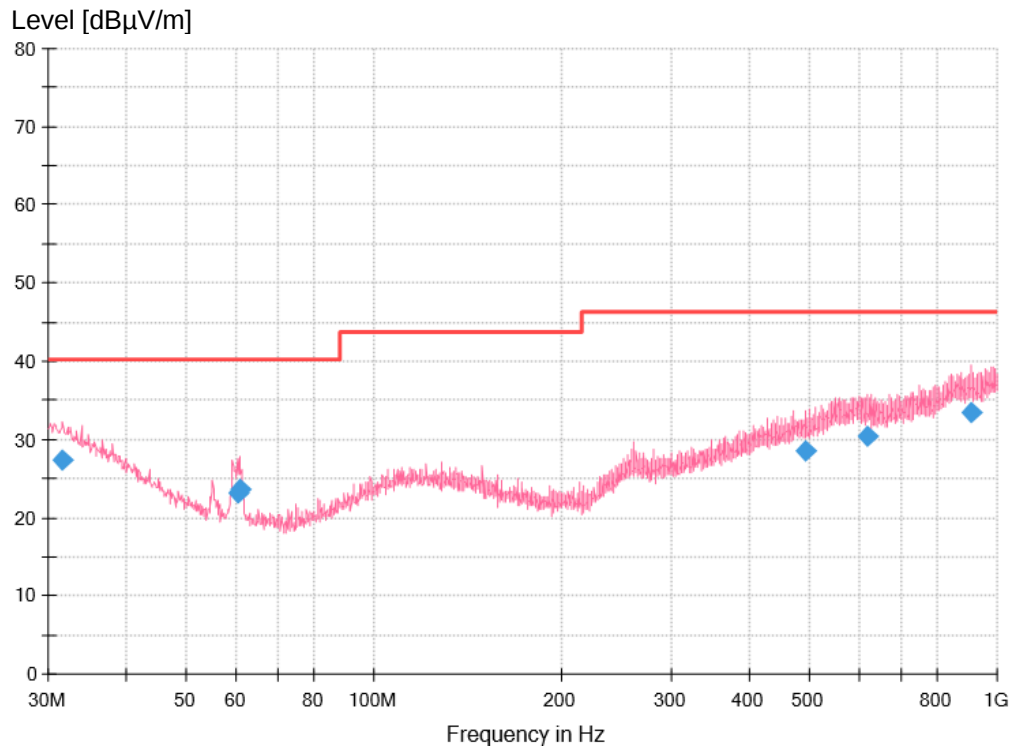
Figure 6: Spectral Diagrams, Radiated Emission, 30 MHz – 1000 MHz, Vertical polarization, Mode 2
