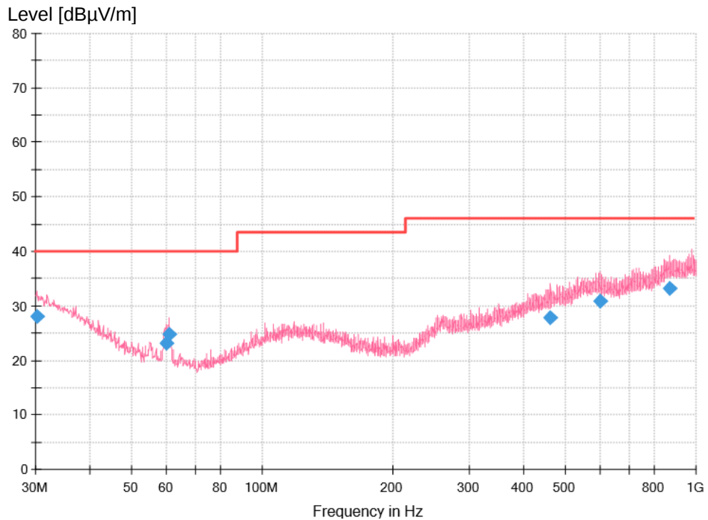
Figure 4: Spectral Diagrams, Radiated Emission, 30 MHz – 1000 MHz, Vertical polarization, Mode 1
