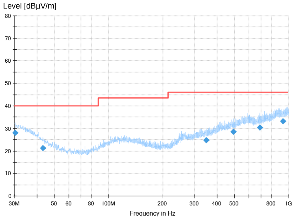
Figure 5: Spectral Diagrams, Radiated Emission, 30 MHz – 1000 MHz, Horizontal polarization, Mode 2
