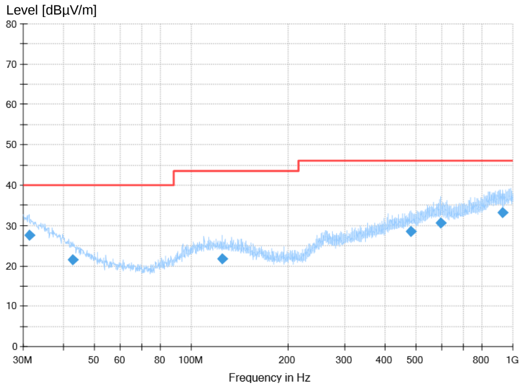
Figure 3: Spectral Diagrams, Radiated Emission, 30 MHz – 1000 MHz, Horizontal polarization, Mode 1
