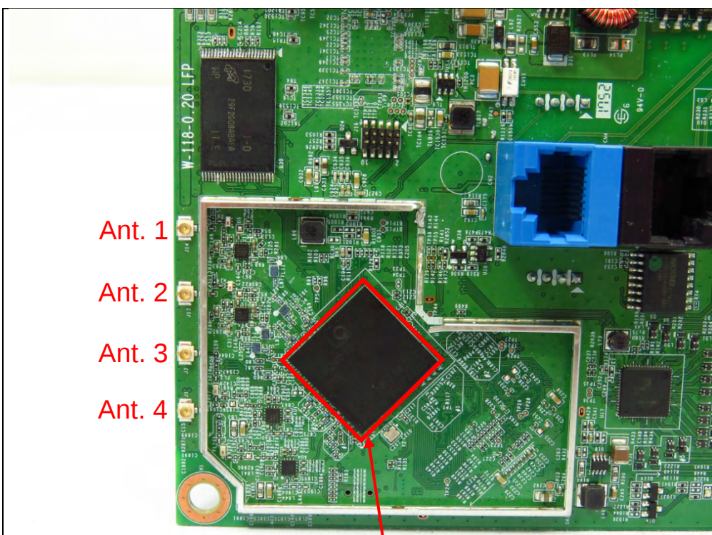
Radio 1, 2 Chip
