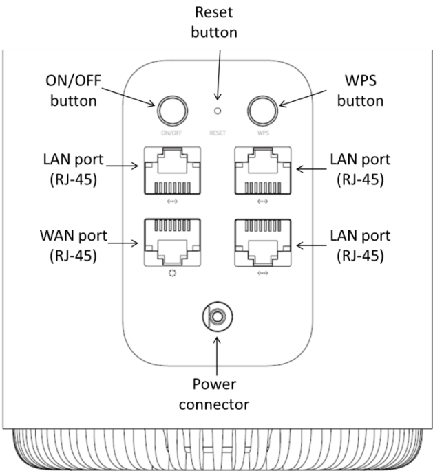
Figure 7 HA-030W-B CPE physical connections
