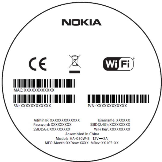
Figure 10 HA-030W-B CPE European (EU) safety label
