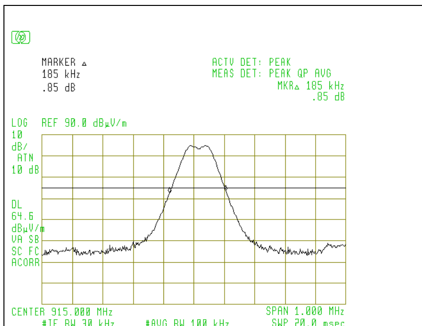
20dB Bandwidth 915 MHz Plot
