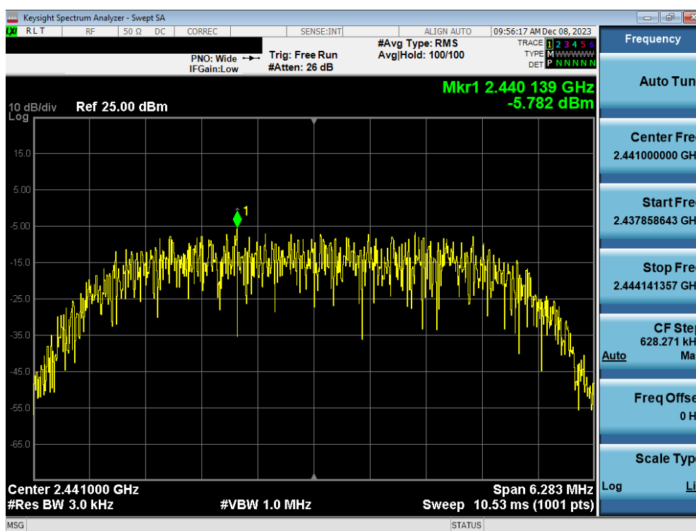
Plot 7-52. Power Spectral Density Plot Tx BF Antenna WF2b (Bluetooth (HDR8), 8Mbps, ePA – Ch. 38)
