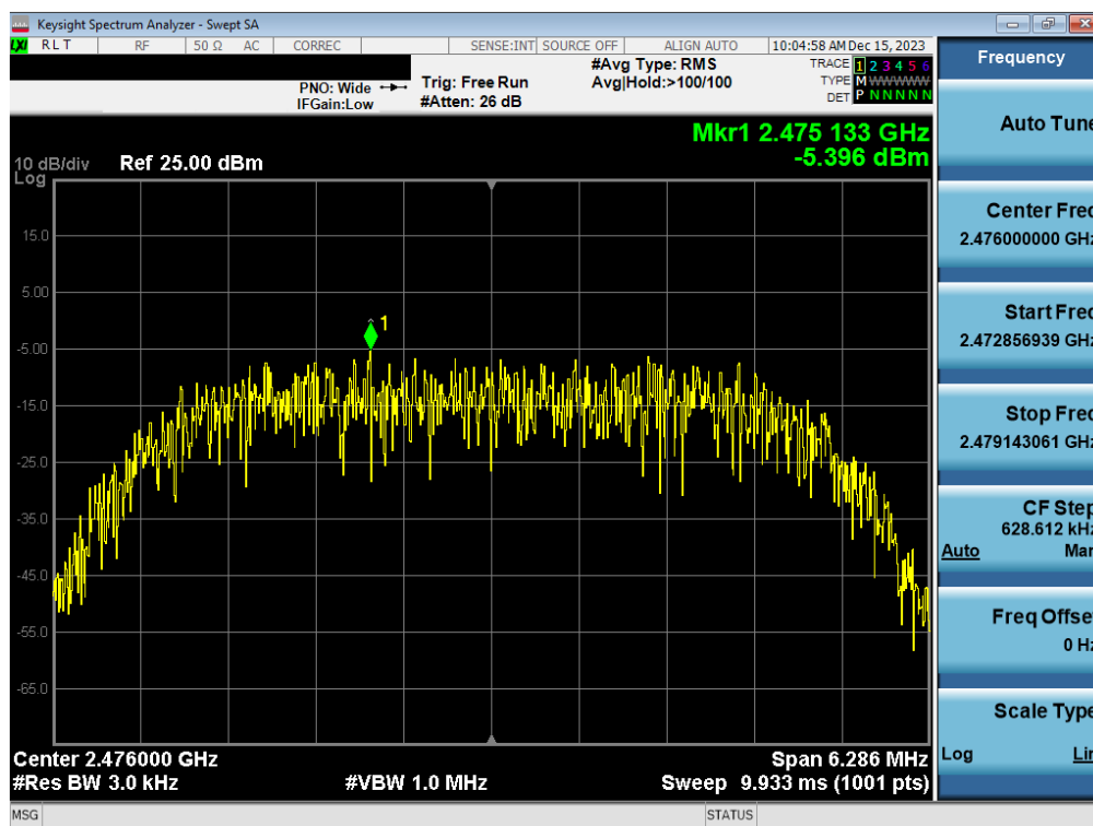
Plot 7-54. Power Spectral Density Plot TxBF Antenna WF2b (Bluetooth (HDR8), 8Mbps, ePA – Ch. 73)
