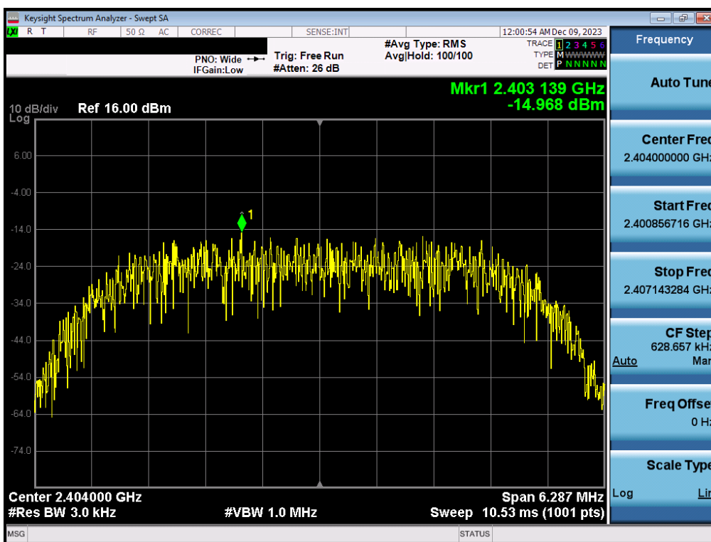
Plot 7-34. Power Spectral Density Plot Antenna WF2b (Bluetooth (HDR8), 8Mbps, iPA – Ch. 1)
