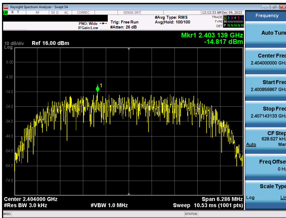
Plot 7-55. Power Spectral Density Plot TxBF Antenna WF7b (Bluetooth (HDR8), 8Mbps, iPA – Ch. 1)
