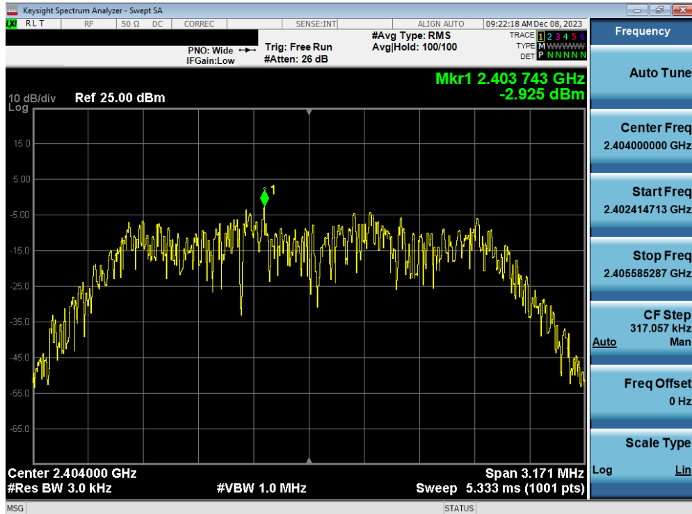
Plot 7-37. Power Spectral Density Plot TxBF Antenna WF7b (Bluetooth (HDR4), 4Mbps, ePA – Ch. 1)
