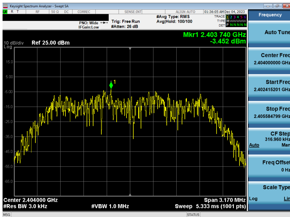
Plot 7-25. Power Spectral Density Plot Antenna WF2b (Bluetooth (HDR4), 4Mbps, ePA – Ch. 1)
