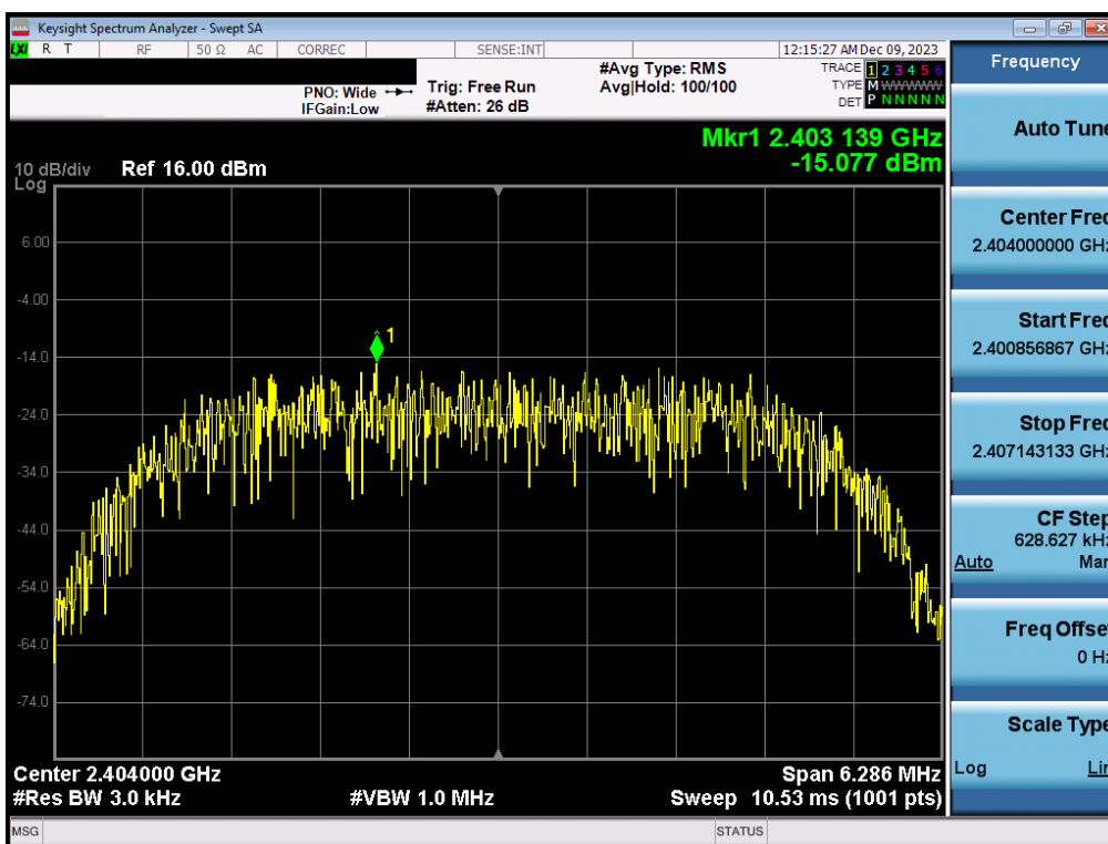
Plot 7-22. Power Spectral Density Plot Antenna WF7b (Bluetooth (HDR8), 8Mbps, iPA – Ch. 1)
