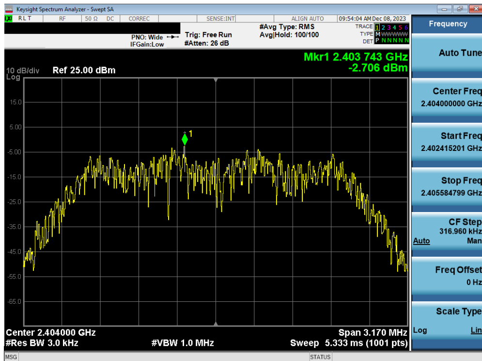
Plot 7-38. Power Spectral Density Plot TxBF Antenna WF2b (Bluetooth (HDR4), 4Mbps, ePA – Ch. 1)
