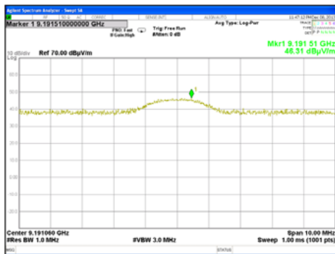
Plot 7.7.72 Radiated emission measurements at the tenth harmonic of high carrier frequency
