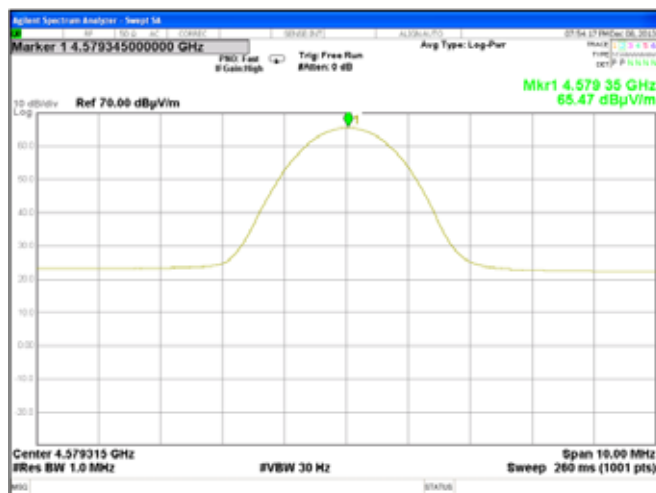
Plot 7.7.40 Radiated emission measurements at the fifth harmonic of mid carrier frequency
