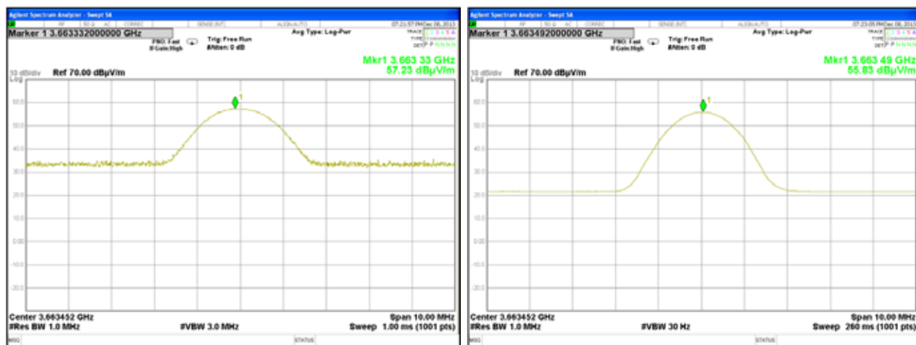
Plot 7.7.34 Radiated emission measurements at the fourth harmonic of mid carrier frequency
