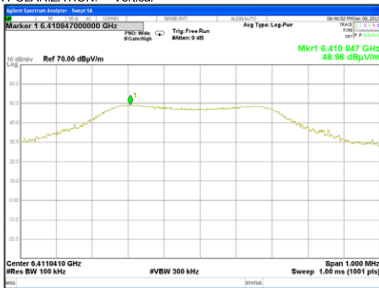
Plot 7.7.52 Radiated emission measurements at the seventh harmonic of mid carrier frequency
