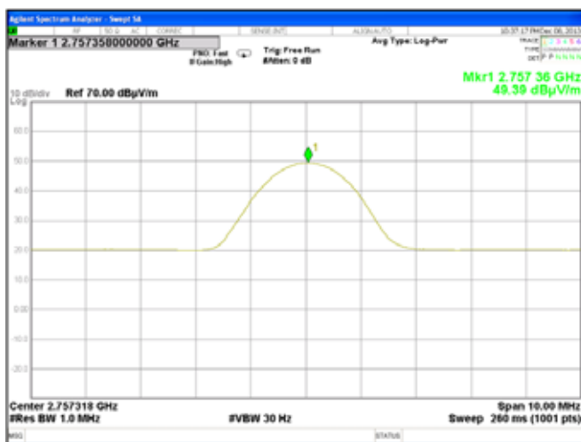
Plot 7.7.30 Radiated emission measurements at the third harmonic of high carrier frequency
