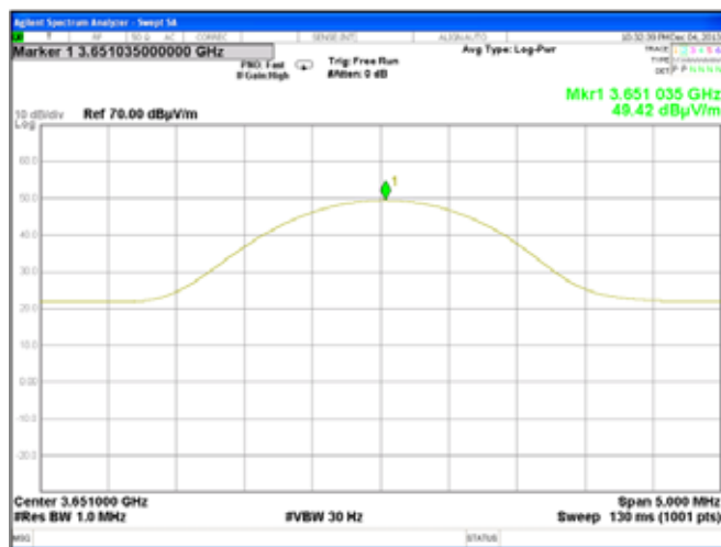
Plot 7.7.32 Radiated emission measurements at the fourth harmonic of low carrier frequency
