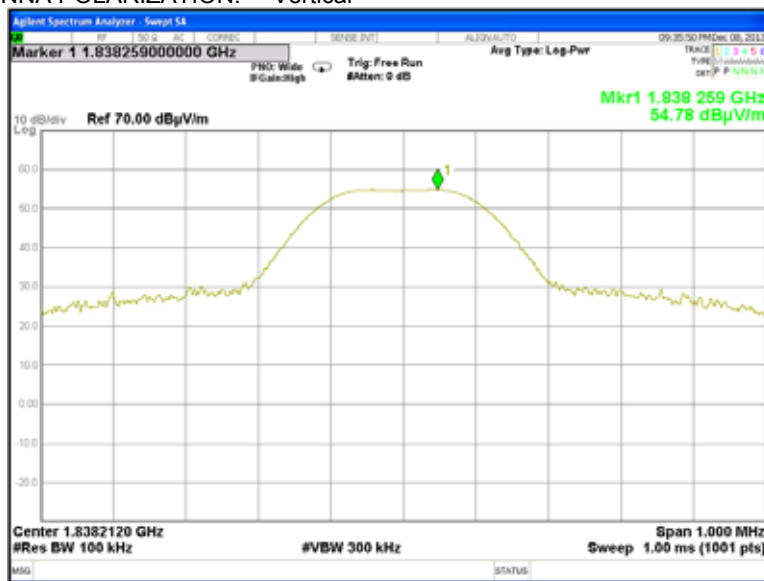
Plot 7.7.24 Radiated emission measurements at the second harmonic of high carrier frequency
