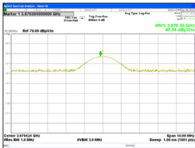
Plot 7.7.36 Radiated emission measurements at the fourth harmonic of high carrier frequency
