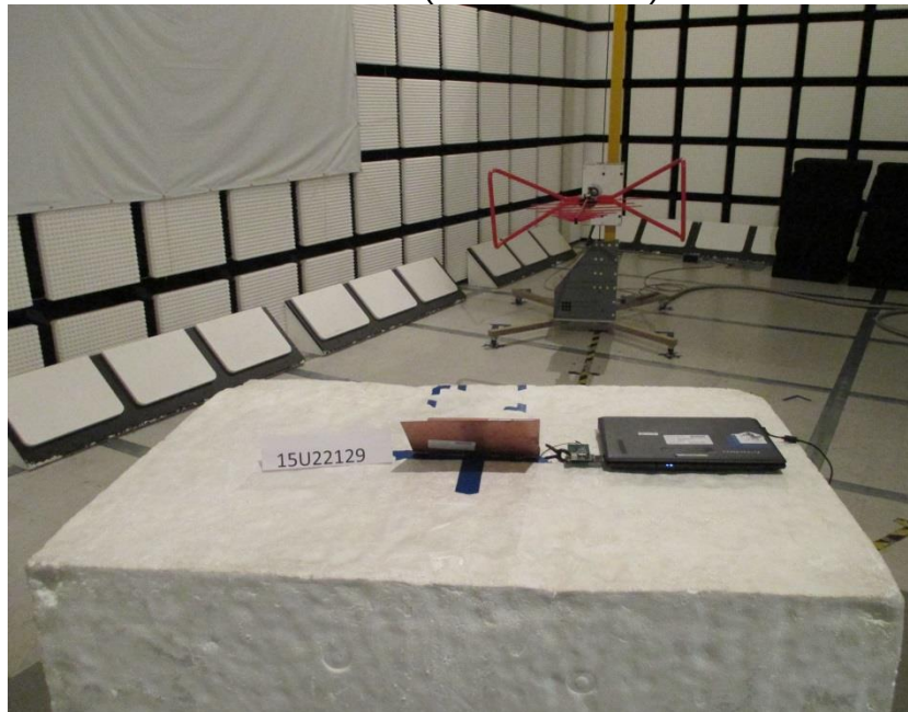
RADIATED FRONT PHOTO (BELOW 1 GHz)
