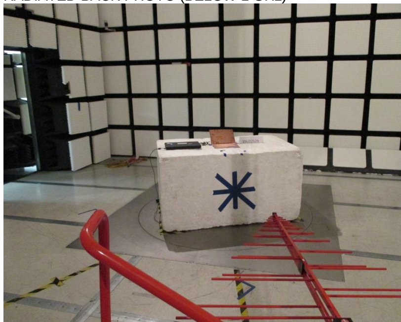
RADIATED BACK PHOTO (BELOW 1 GHz)
