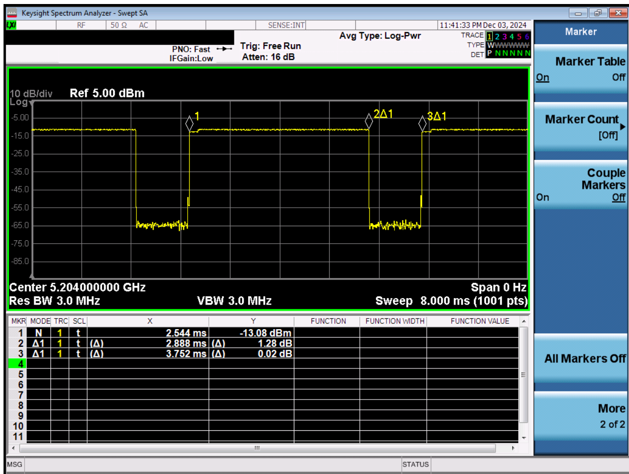
Figure 7-13 NB UNII-1 HDR8 Transmission Plot – Antenna WF2a, Variant 2
