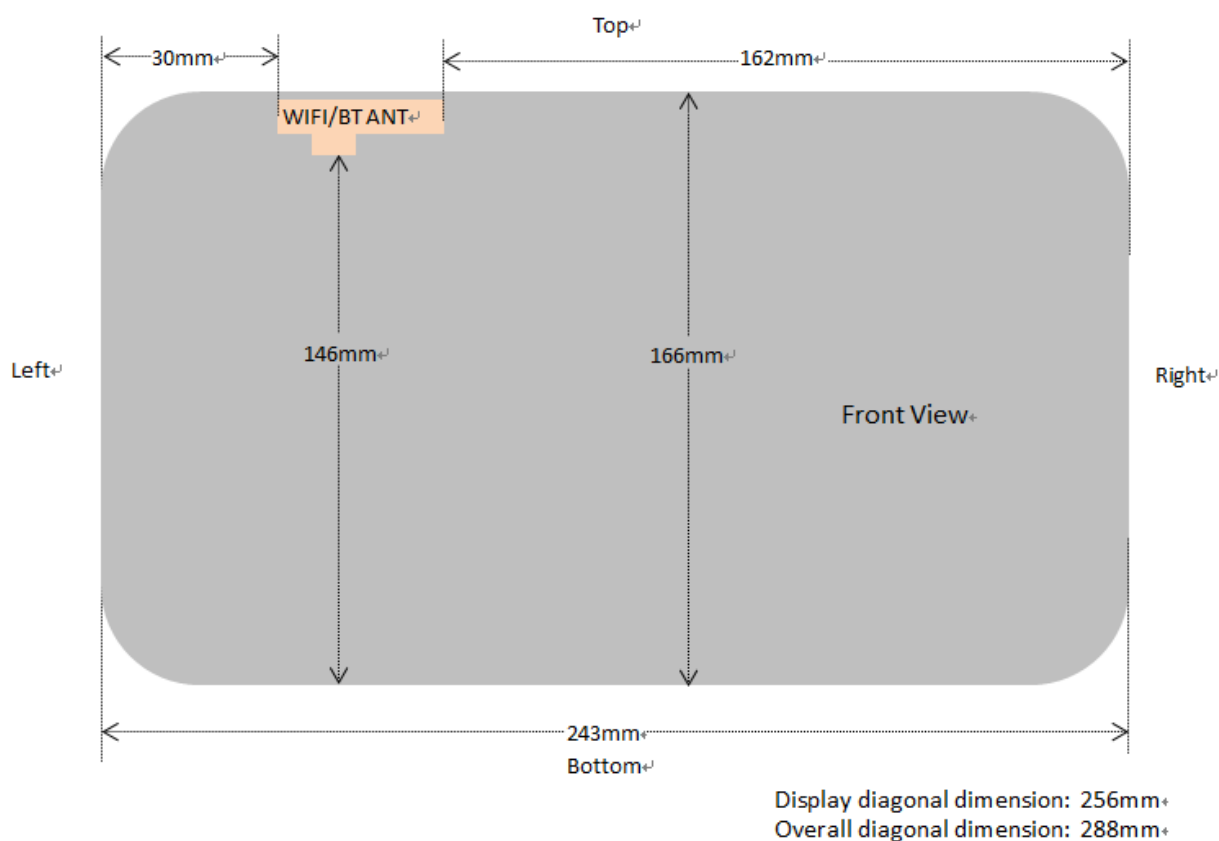
Fig.14.1 EUT Antenna Locations
