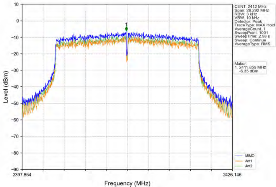
802.11ax(HE20)_LCH_2412MHz_RU242_Left_MIMO_NTNV
