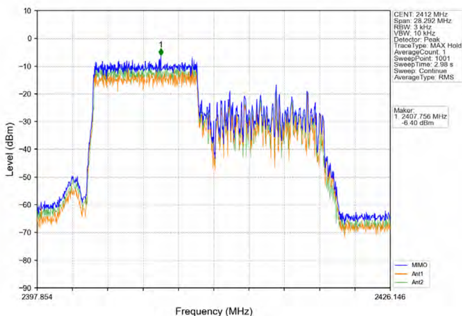
802.11ax(HE20) LCH_2412MHz_RU106 Left_MIMO_NTNV
