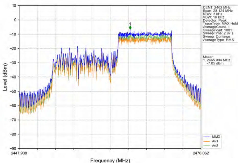
802.11ax(HE20)_HCH_2462MHz_RU106_Right_MIMO_NTNV
