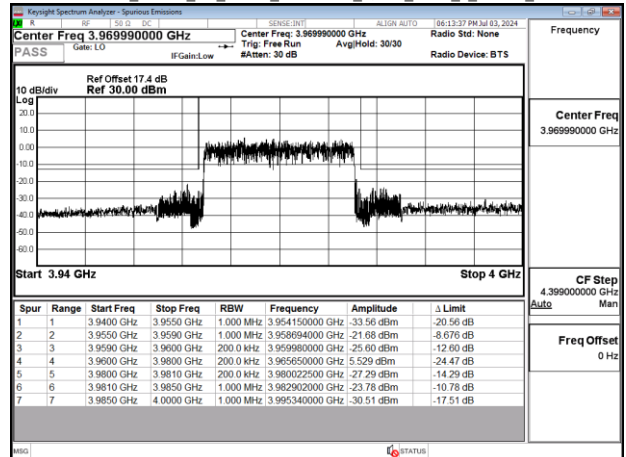
Band77-Part27_20MHz_CP_OFDM_SCS30kHz_QPSK_RB51_0_Chain0_CH664666
