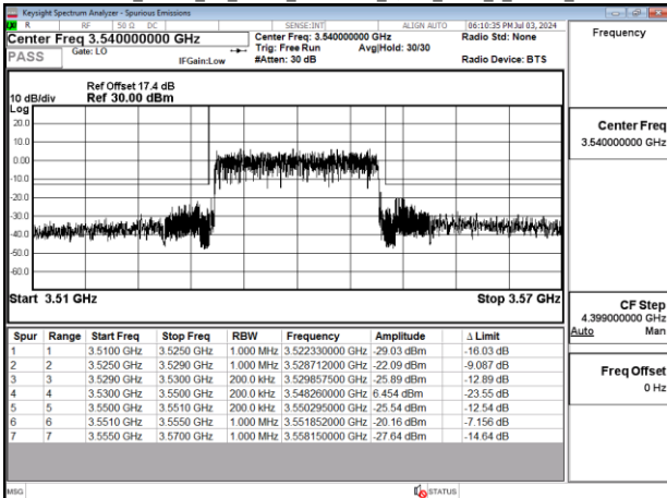
Band77-Part27_20MHz_CP_OFDM_SCS30kHz_QPSK_RB51_0_Chain0_CH636000
