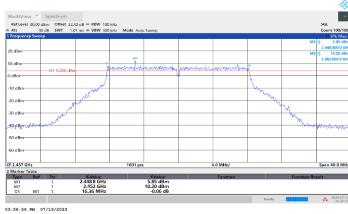
11G-CDD_Ant3_2457
