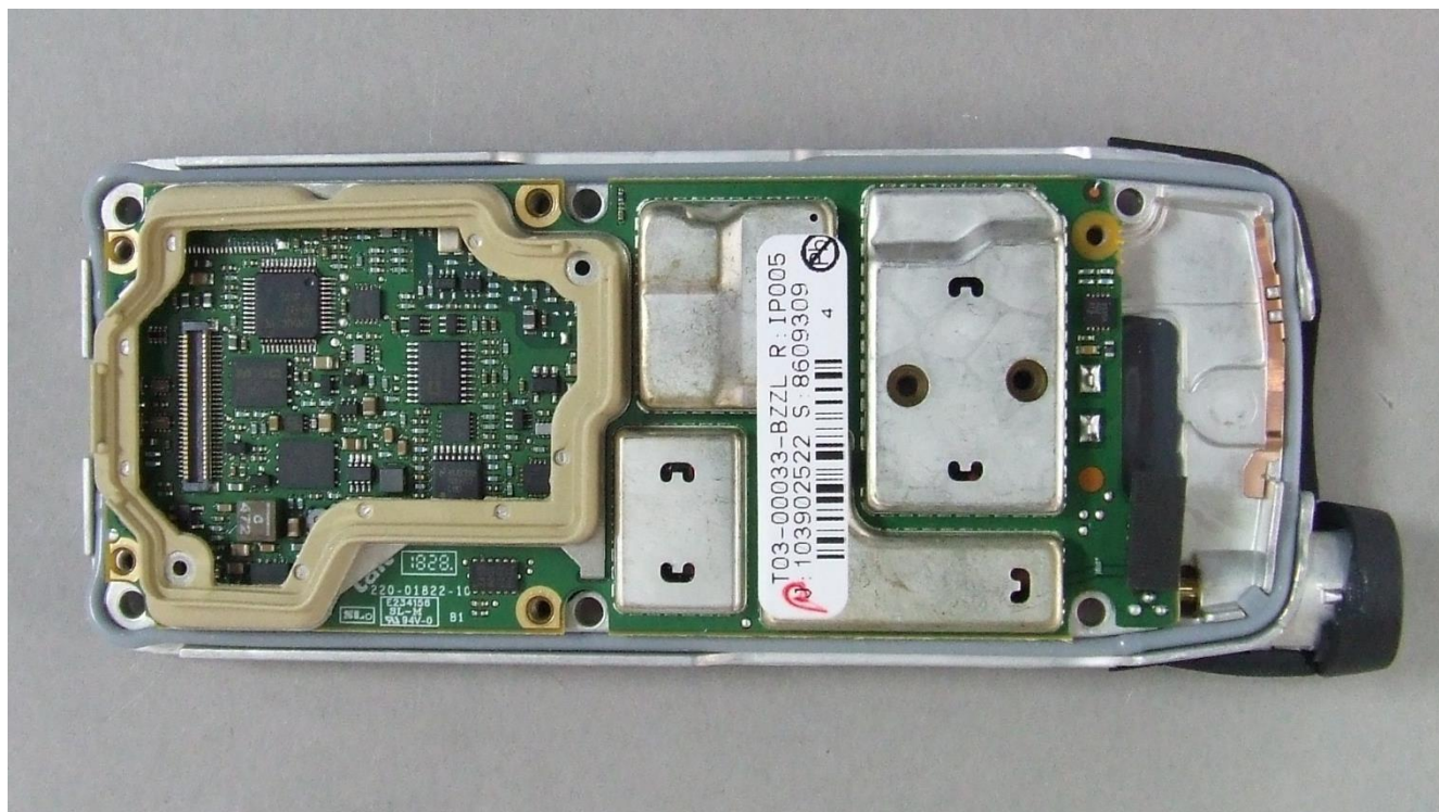
Photograph 02: Rx-Tx PCB - top (with shields)
