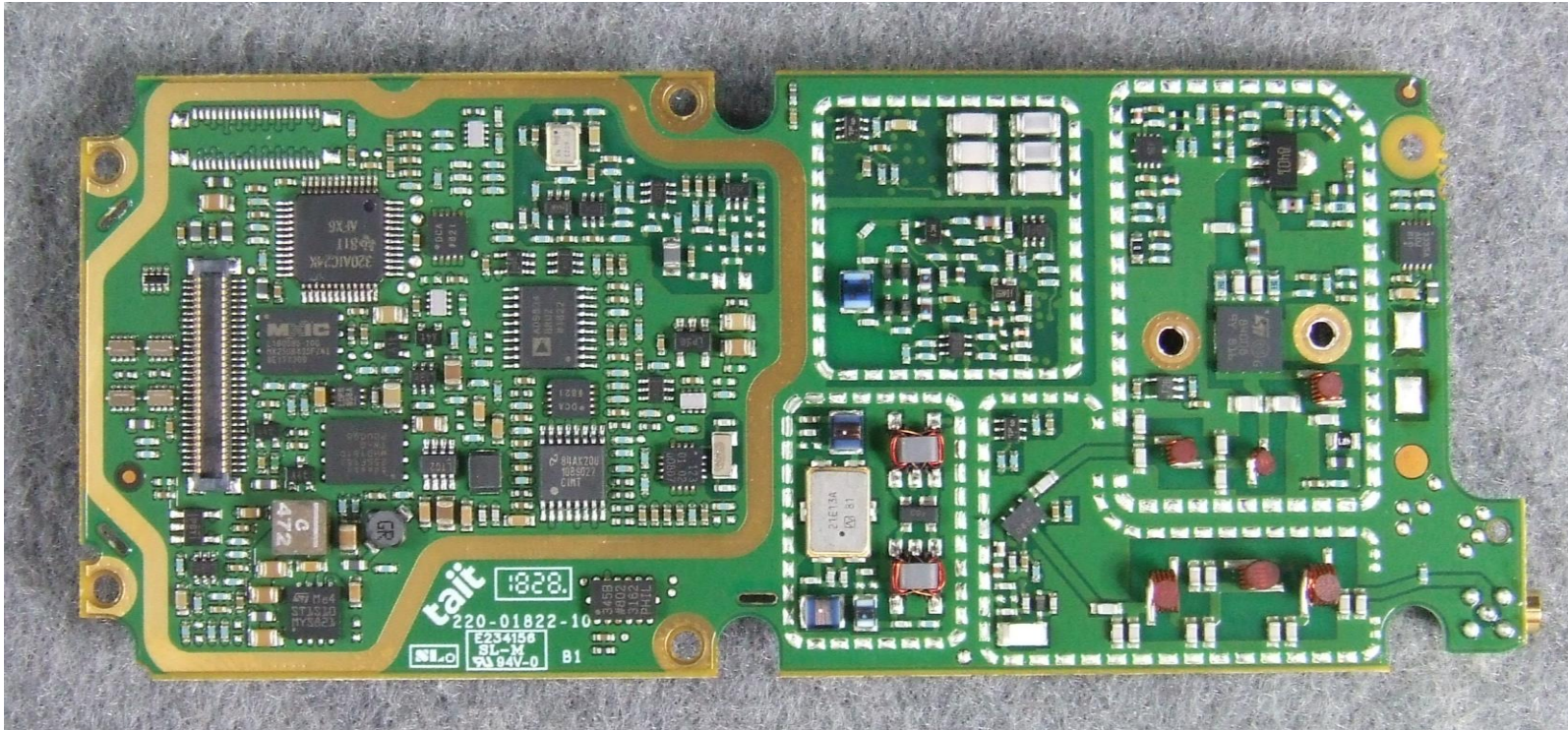
Photograph 03: Rx-Tx PCB - top (without shields)
