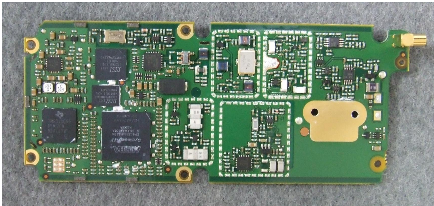
Photograph 05: Rx-Tx PCB - bottom (without shields)
