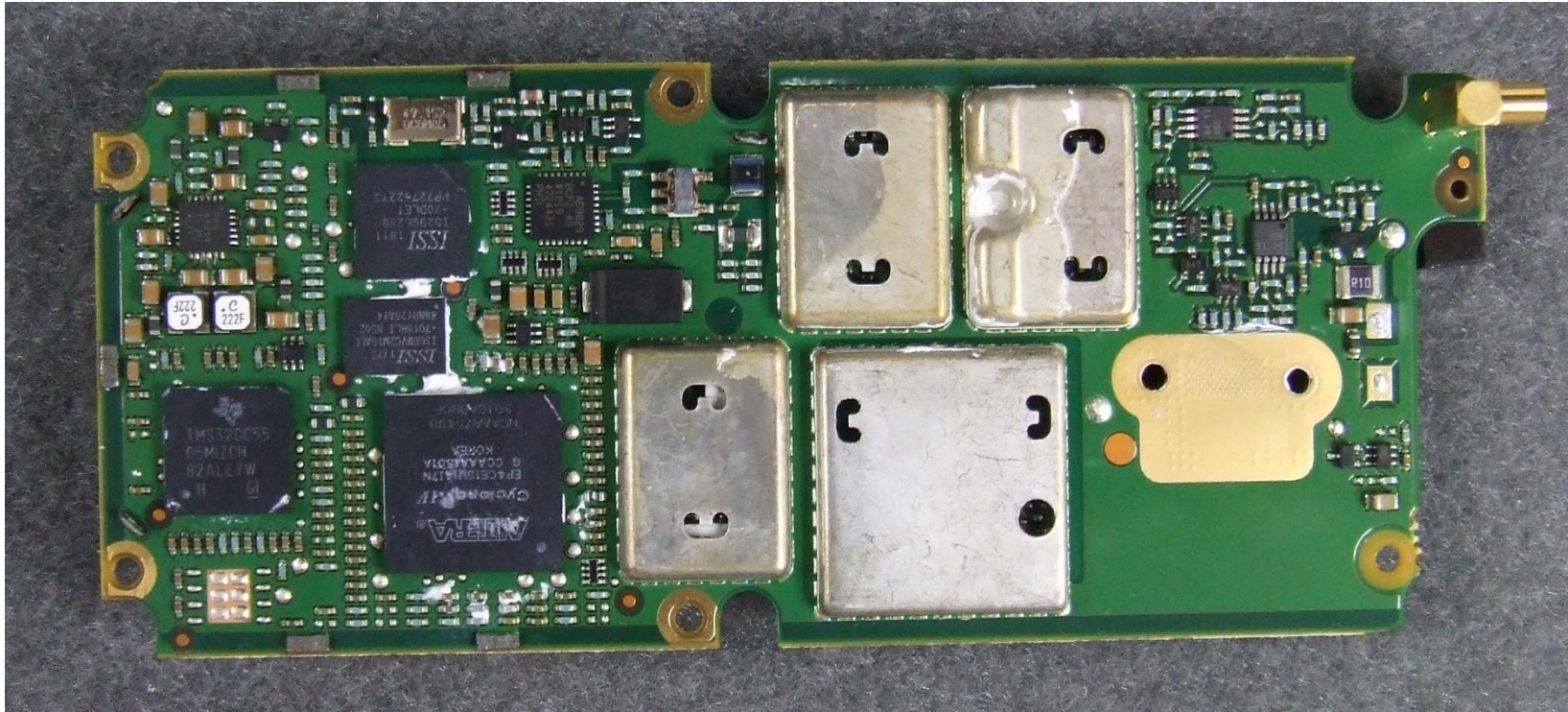
Photograph 04: Rx-Tx PCB - bottom (with shields)
