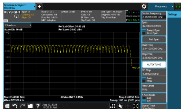
3-DH5(2Mbps)-2441~2483.5MHz
