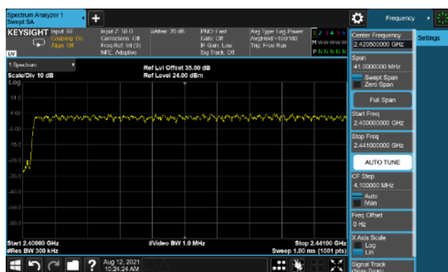
3-DH5(3Mbps)-2400~2441MHz
