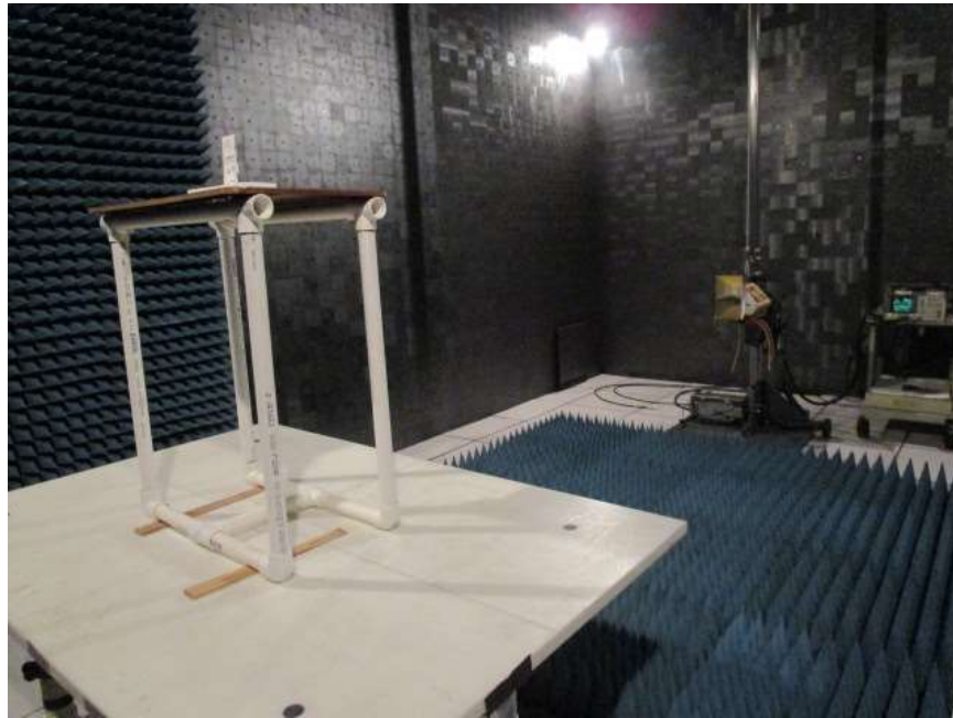
Radiated Emissions Test Setup 1 to 18 GHz
