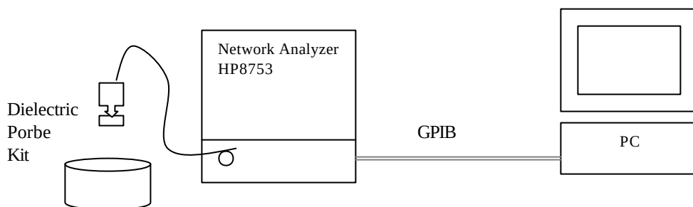
Figure 5: Test configuration
