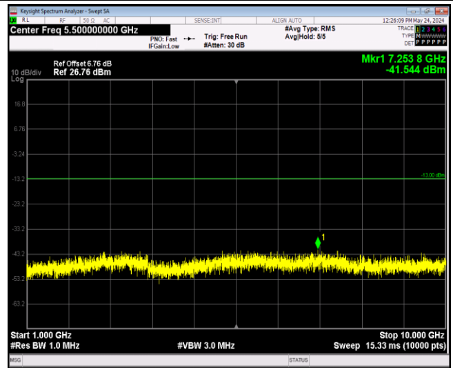
Band13-5MHz-64QAM-23230-1RB#0-Range2:1000~100 00MHz
