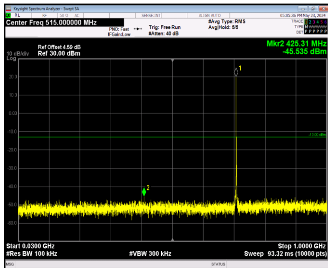
Band12-1.4MHz-16QAM-23017-1RB#0-Range1:30~1 00MHz
