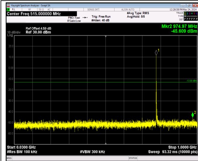
Band13-5MHz-64QAM-23205-1RB#0-Range1:30~100 0MHz
