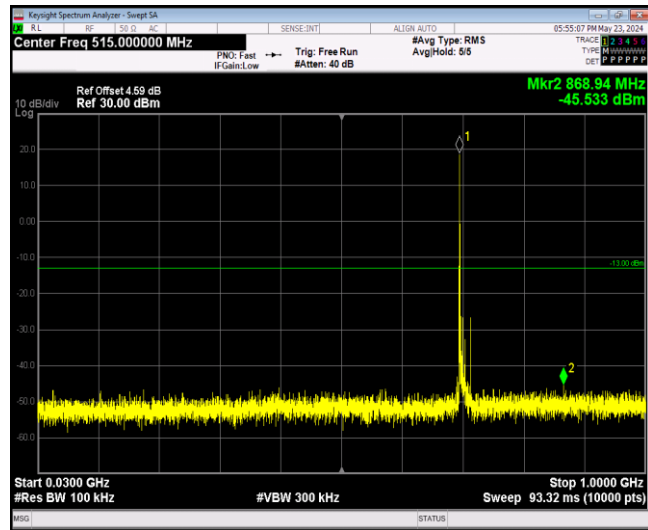
Band12-10MHz-64QAM-23130-1RB#0-Range1:30~10 00MHz
