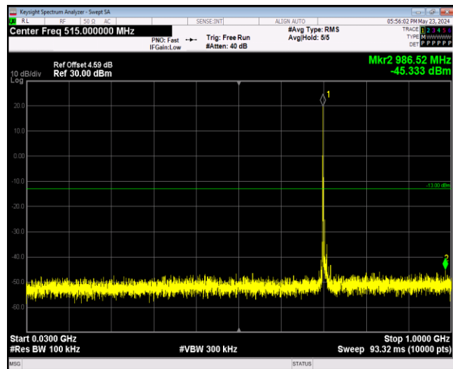
Band13-5MHz-QPSK-23205-1RB#0-Range1:30~1000 MHz
