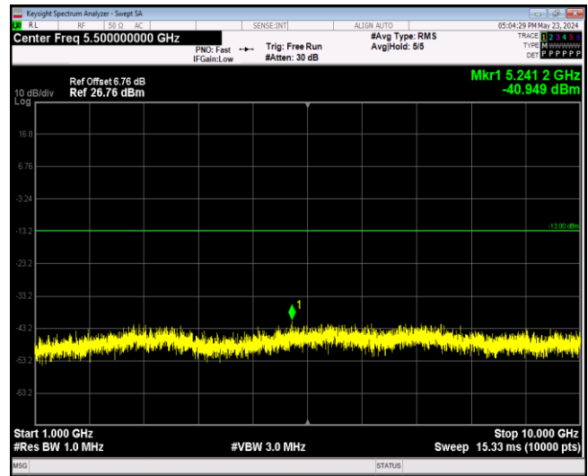
Band12-1.4MHz-64QAM-23095-1RB#0-Range2:1000~10 000MHz
