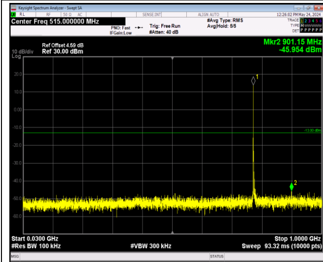
Band13-5MHz-64QAM-23230-1RB#0-Range1:30~100 0MHz
