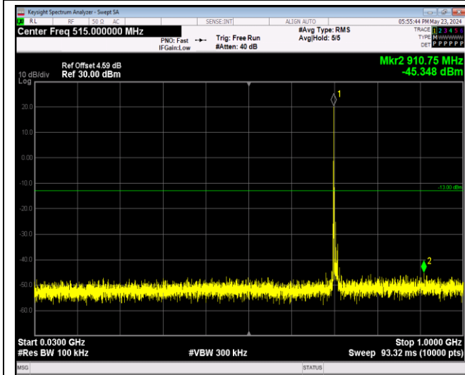
Band12-10MHz-64QAM-23060-1RB#0-Range1:30~1000MHz
