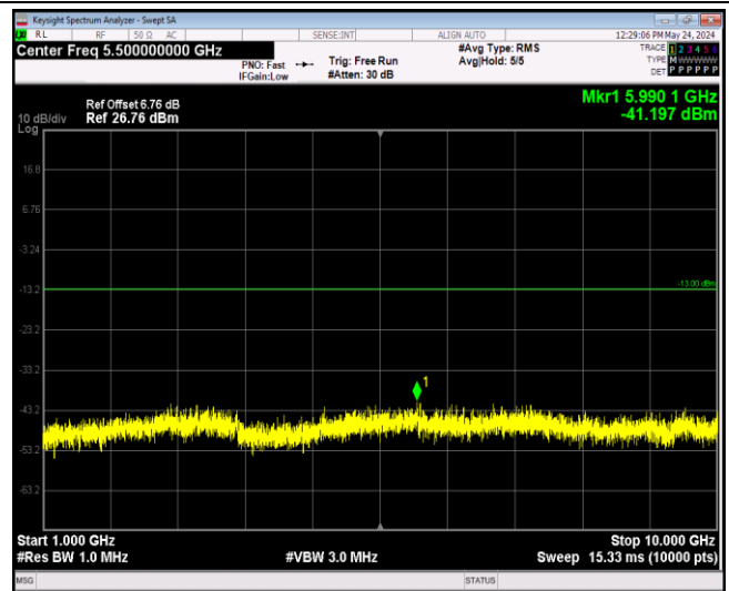
Band13-5MHz-64QAM-23205-1RB#0-Range2:1000~100 00MHz
