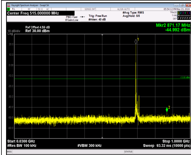
Band12-10MHz-64QAM-23060-1RB#0-Range1:30~1000MHz
