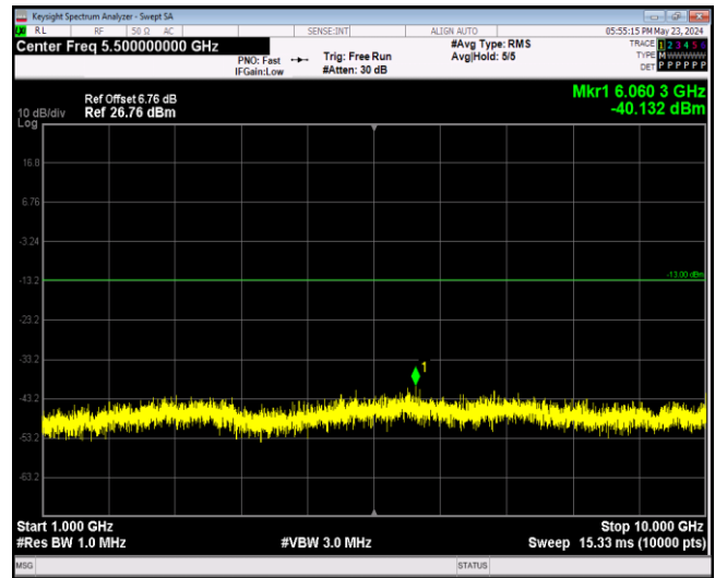
Band12-10MHz-64QAM-23130-1RB#0-Range2:1000~10 00MHz
