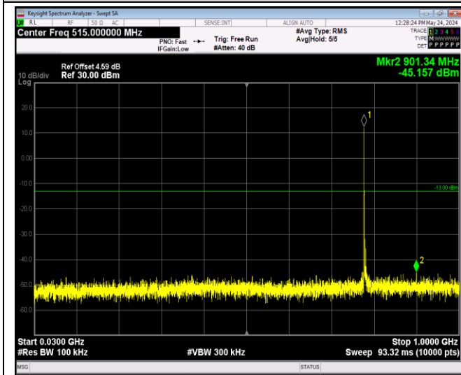
Band13-5MHz-QPSK-23255-1RB#0-Range1:30~1000 MHz
