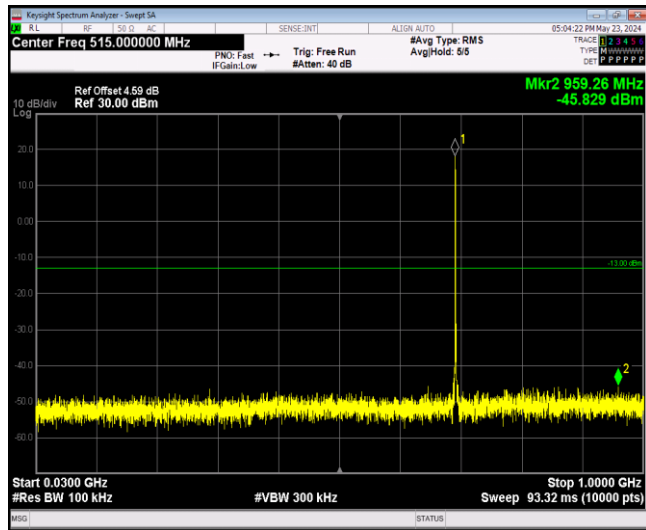
Band12-1.4MHz-64QAM-23095-1RB#0-Range1:30~1 000MHz
