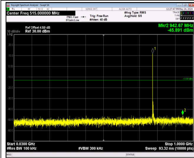
Band13-5MHz-64QAM-23230-1RB#0-Range1:30~100 0MHz
