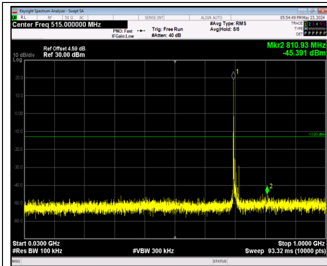
Band12-10MHz-16QAM-23130-1RB#0-Range1:30~1000MHz
