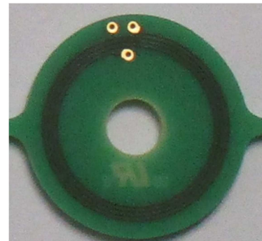
Antenna Type 2 Bottom
