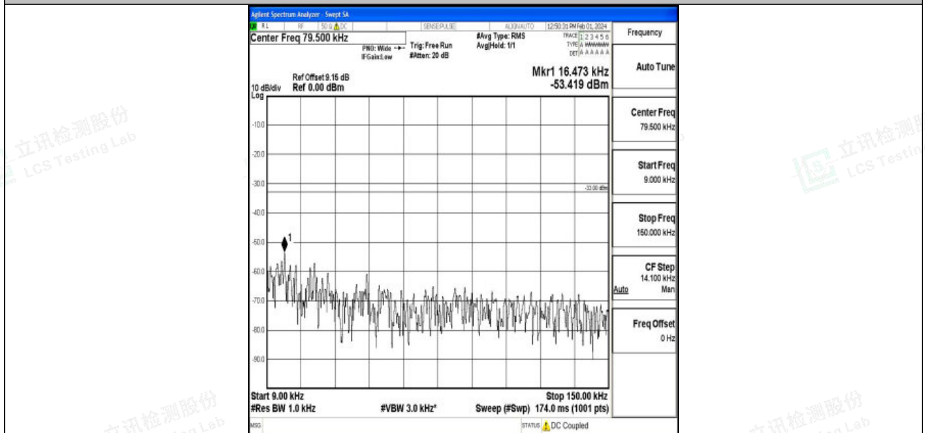
Band5_1.4MHz_16QAM_20525_1RB#0_0.009~0.15_0.009~0.15
