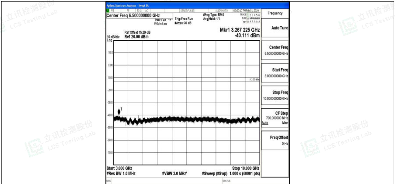
Band5_10MHz_QPSK_20600_1RB#0_3000~10000_3000~10000
