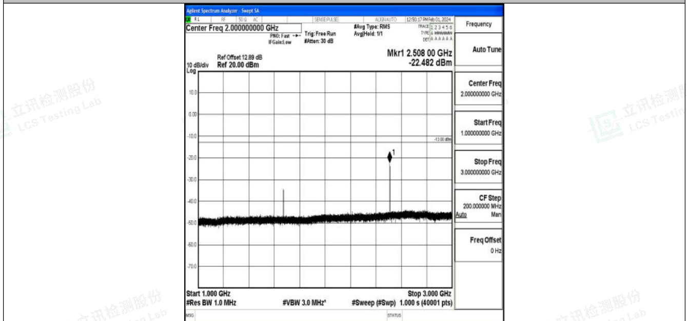
Band5_1.4MHz_QPSK_20525_1RB#0_1000~3000_1000~3000
