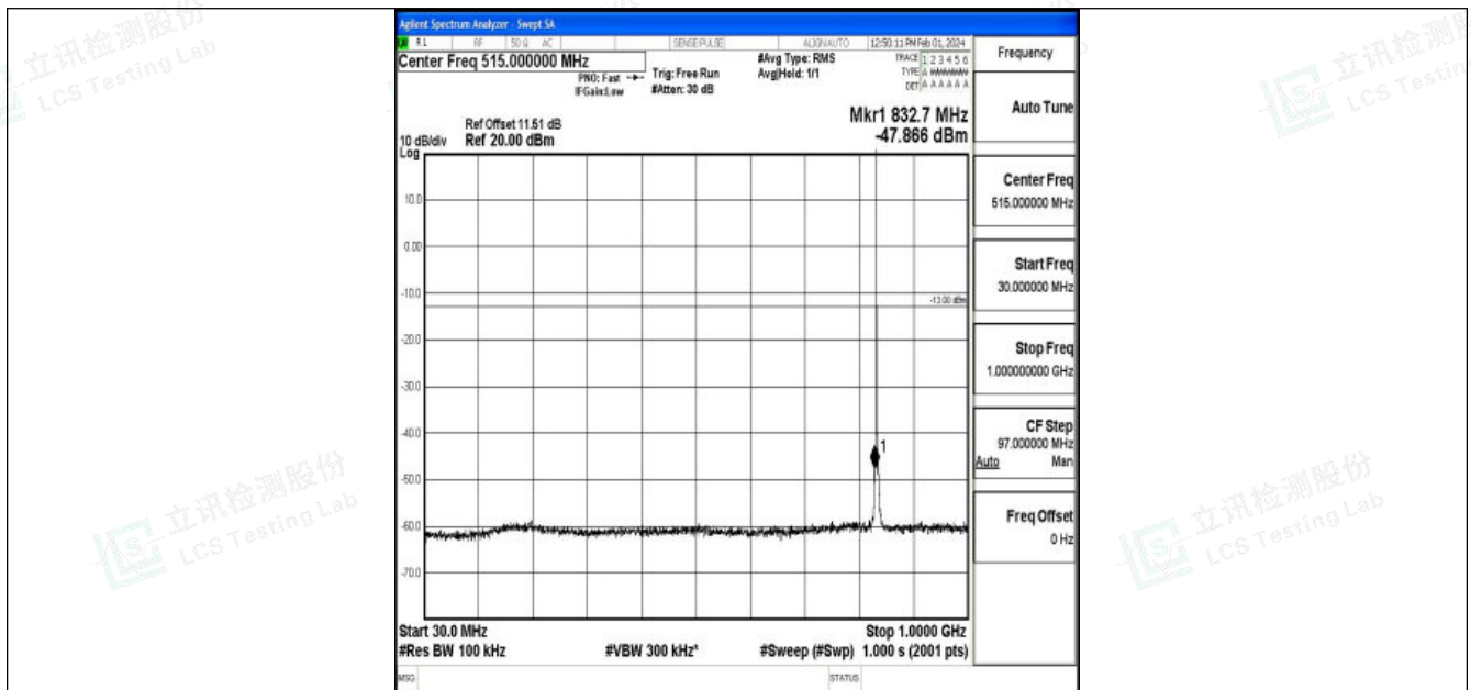
Band5_1.4MHz_QPSK_20525_1RB#0_30~1000_30~1000
