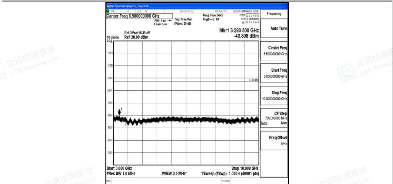
Band5_10MHz_16QAM_20600_1RB#0_3000~10000_3000~10000
