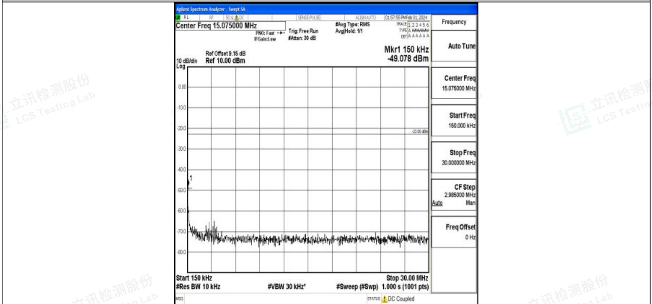
Band5_10MHz_QPSK_20450_1RB#0_0.15~30_0.15~30
