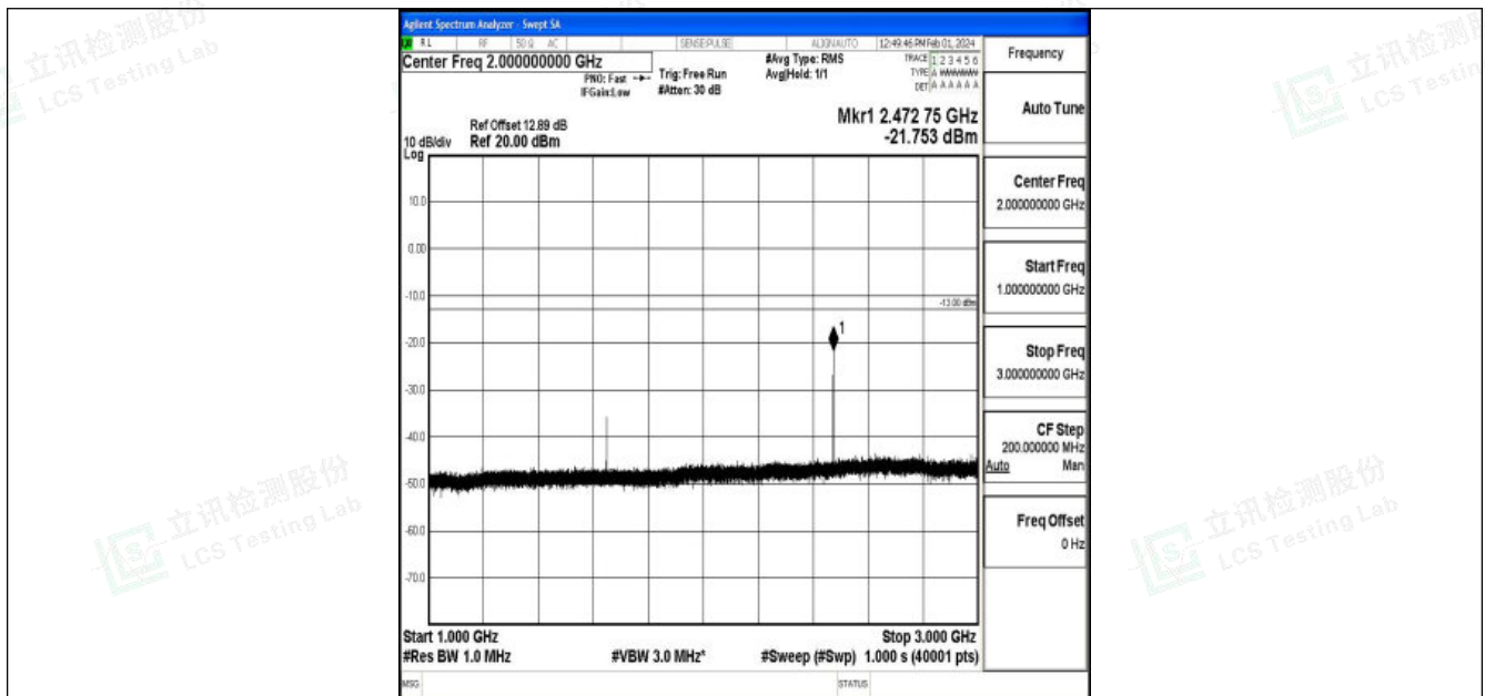
Band5_1.4MHz_16QAM_20407_1RB#0_1000~3000_1000~3000
