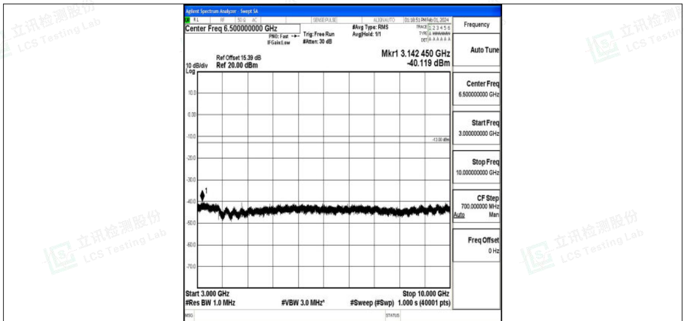
Band5_3MHz_QPSK_20635_1RB#0_3000~10000_3000~10000
