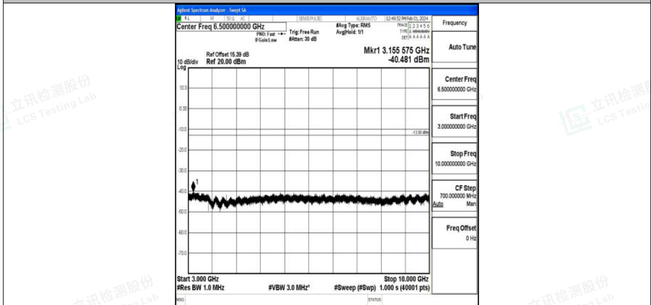
Band5_1.4MHz_16QAM_20407_1RB#0_3000~10000_3000~10000
