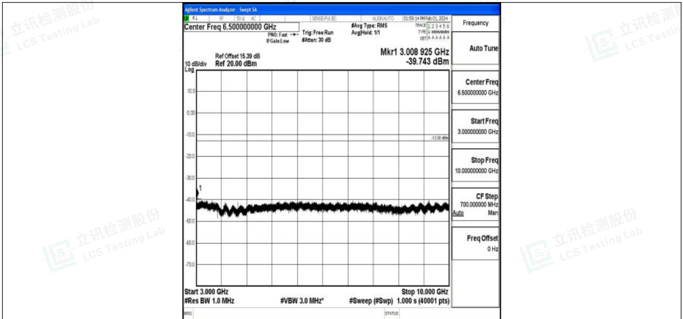
Band5_10MHz_QPSK_20525_1RB#0_3000~10000_3000~10000
