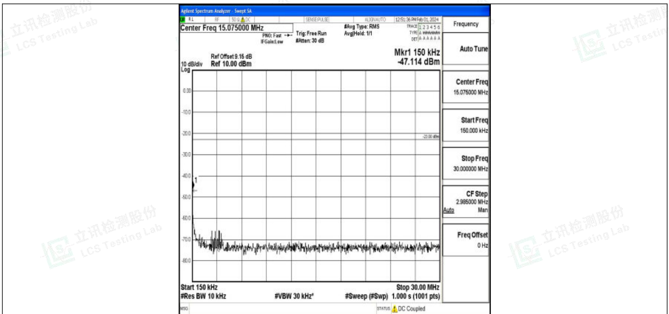
Band5_1.4MHz_16QAM_20643_1RB#0_0.15~30_0.15~30
