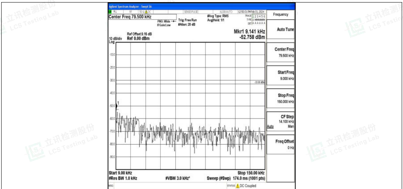
Band5_1.4MHz_QPSK_20525_1RB#0_0.009~0.15_0.009~0.15
