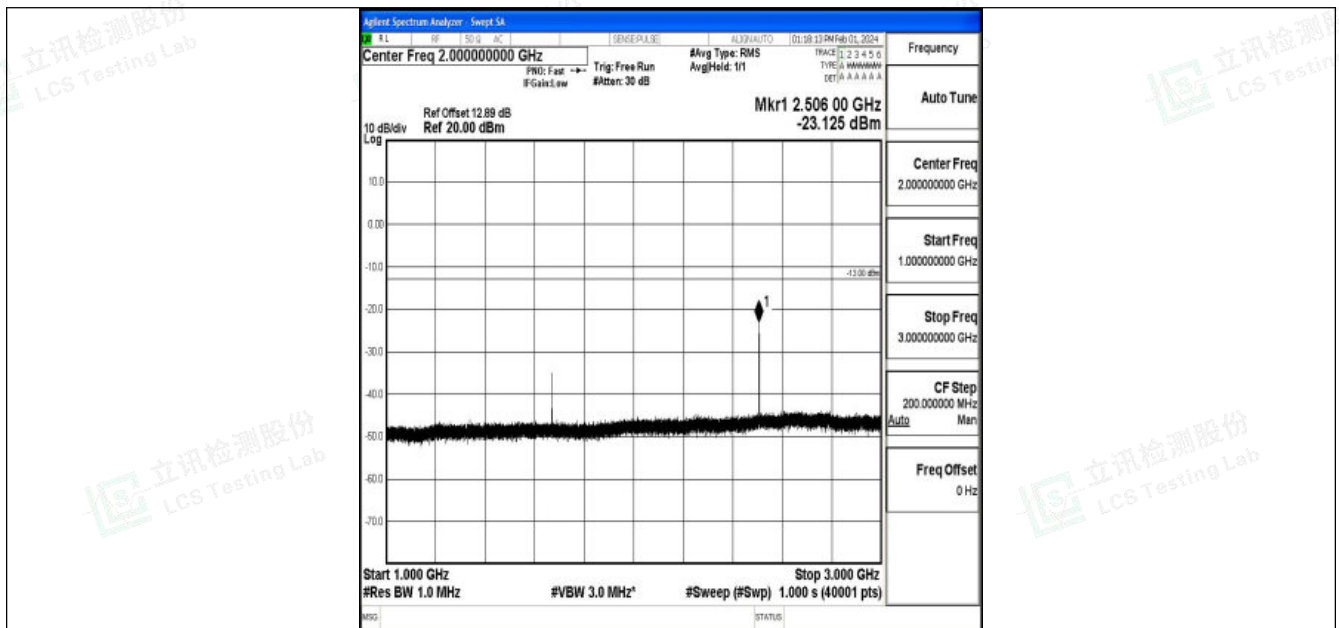
Band5_3MHz_16QAM_20525_1RB#0_1000~3000_1000~3000
