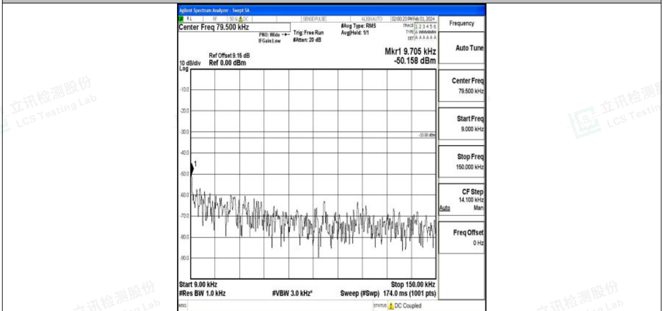
Band5_10MHz_16QAM_20600_1RB#0_0.009~0.15_0.009~0.15
