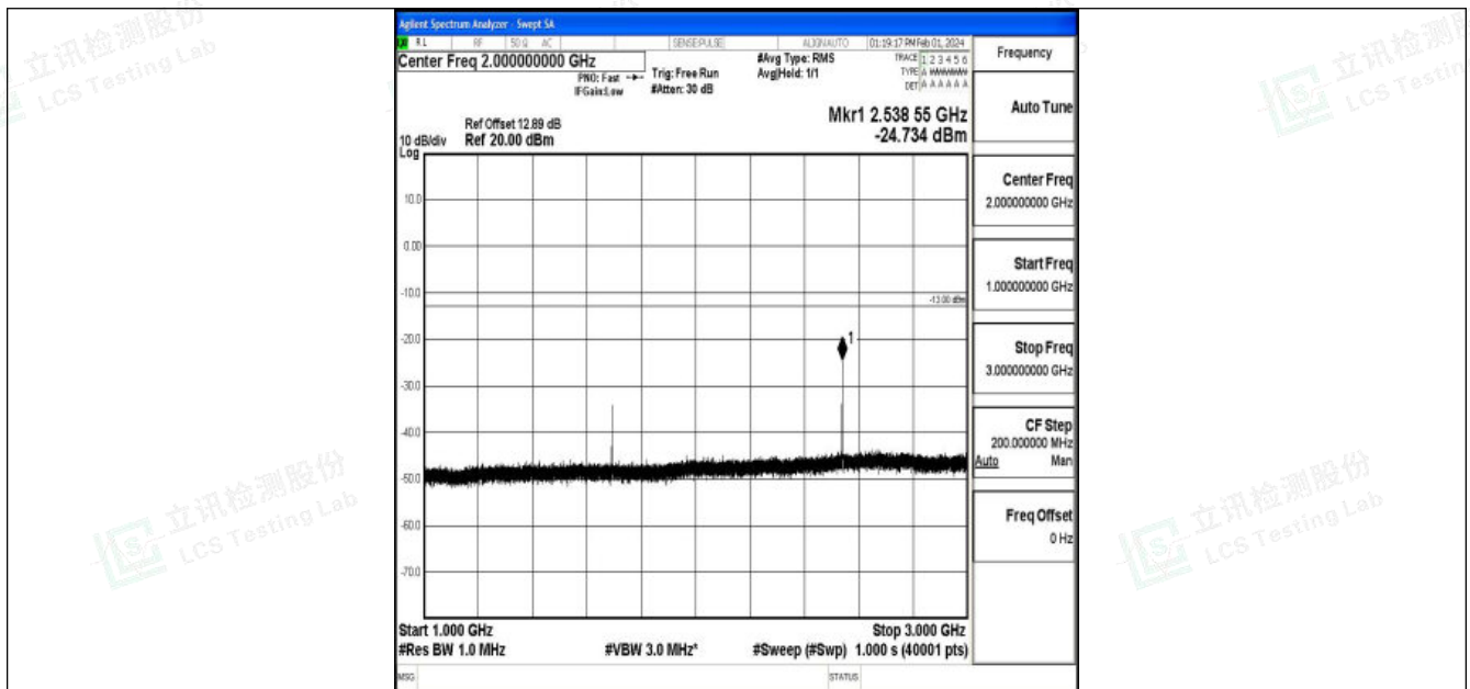
Band5_3MHz_16QAM_20635_1RB#0_1000~3000_1000~3000
