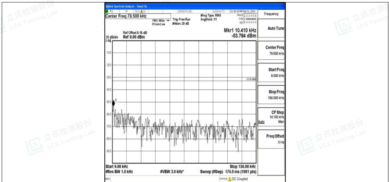
Band5_5MHz_QPSK_20525_1RB#0_0.009~0.15_0.009~0.15
