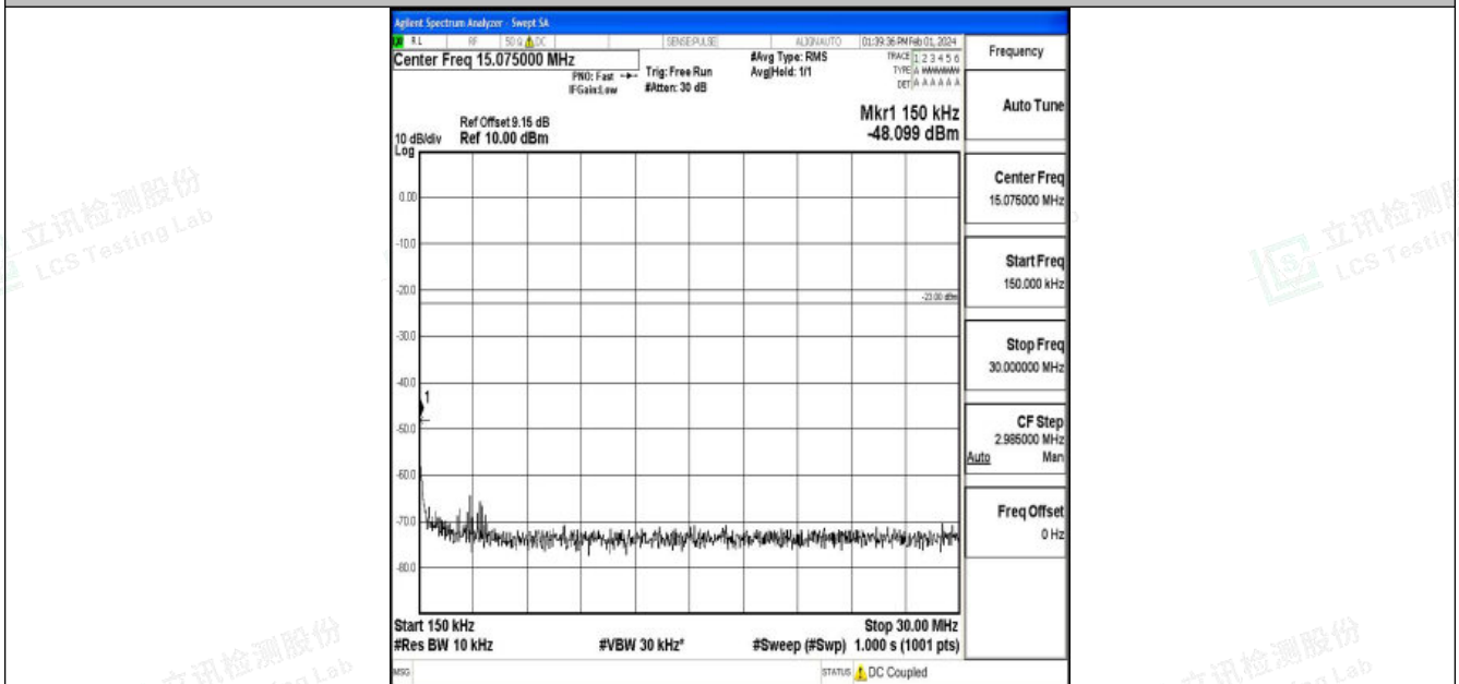
Band5_5MHz_QPSK_20625_1RB#0_0.15~30_0.15~30
