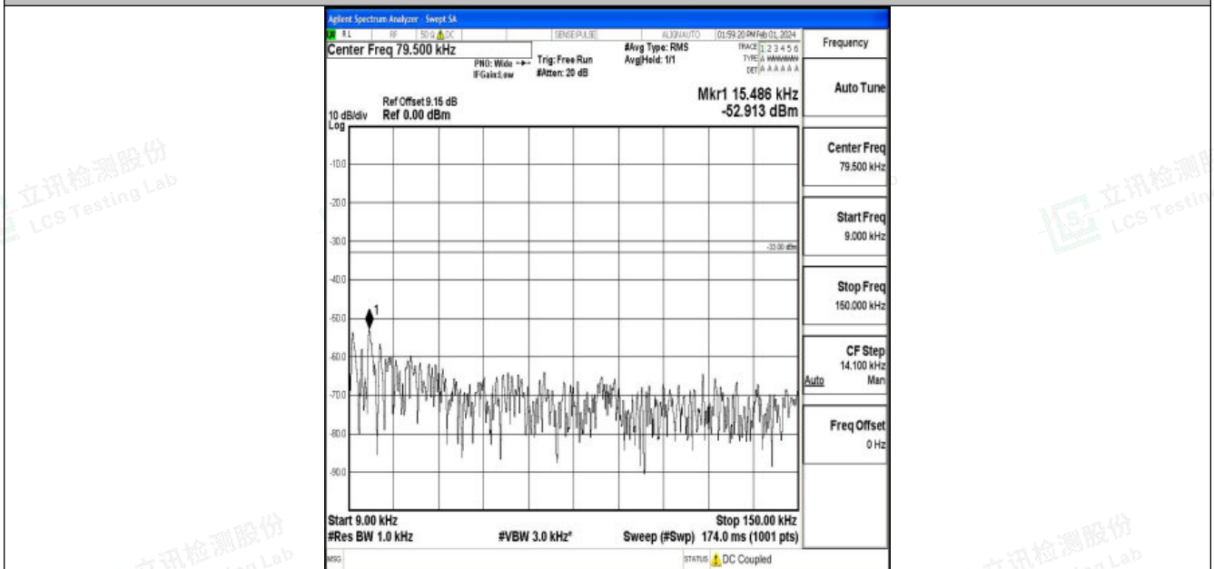
Band5_10MHz_16QAM_20525_1RB#0_0.009~0.15_0.009~0.15
