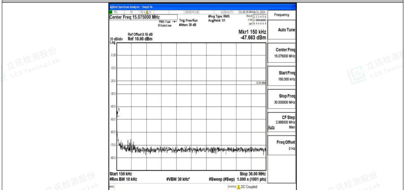
Band5_5MHz_QPSK_20525_1RB#0_0.15~30_0.15~30
