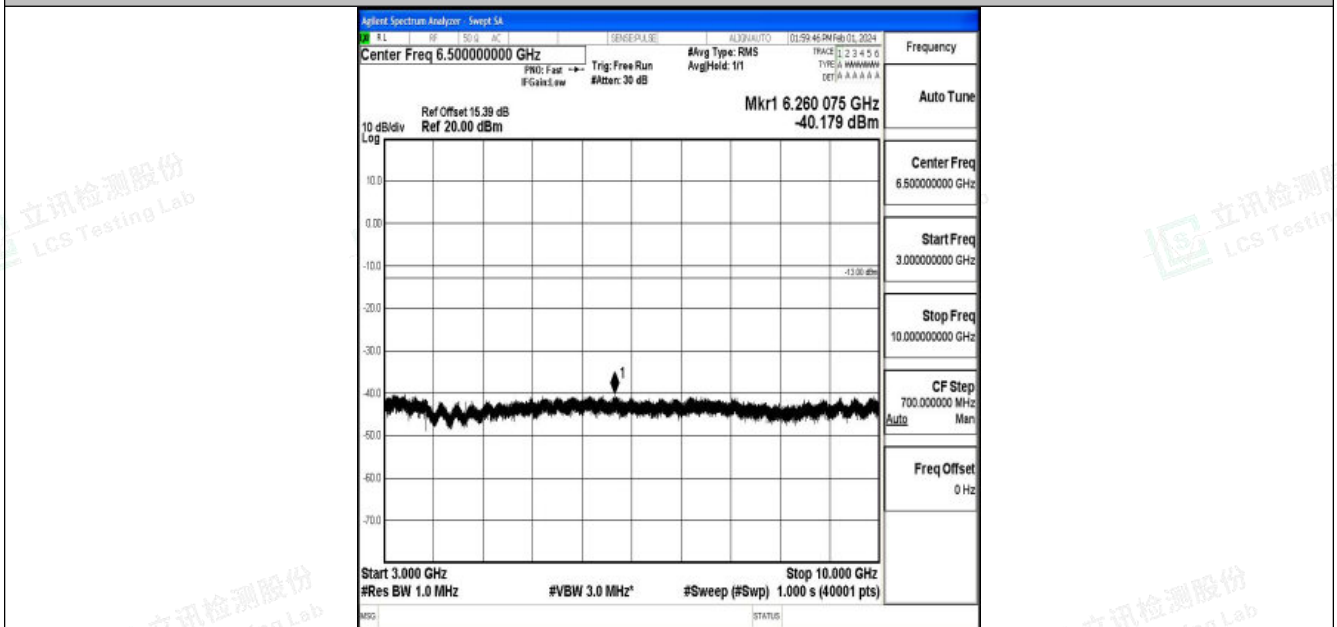
Band5_10MHz_16QAM_20525_1RB#0_3000~10000_3000~10000
