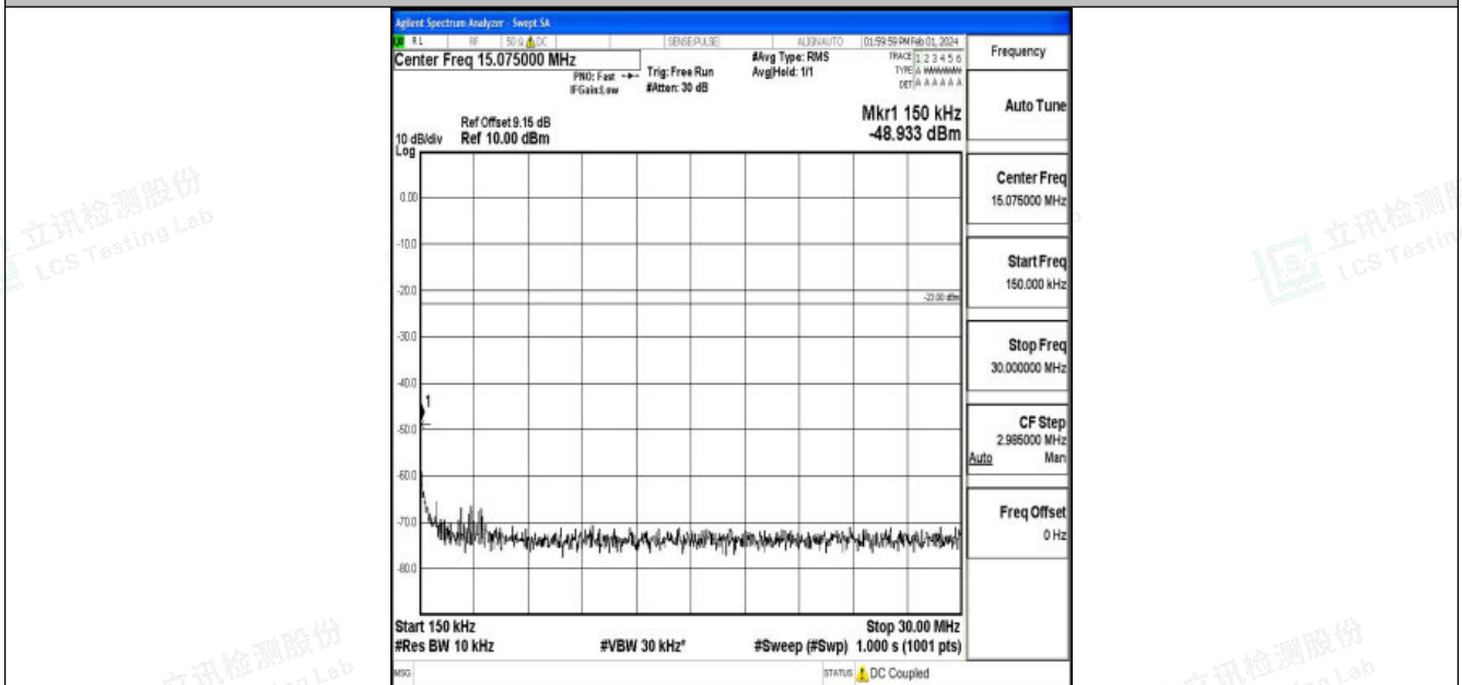
Band5_10MHz_QPSK_20600_1RB#0_0.15~30_0.15~30
