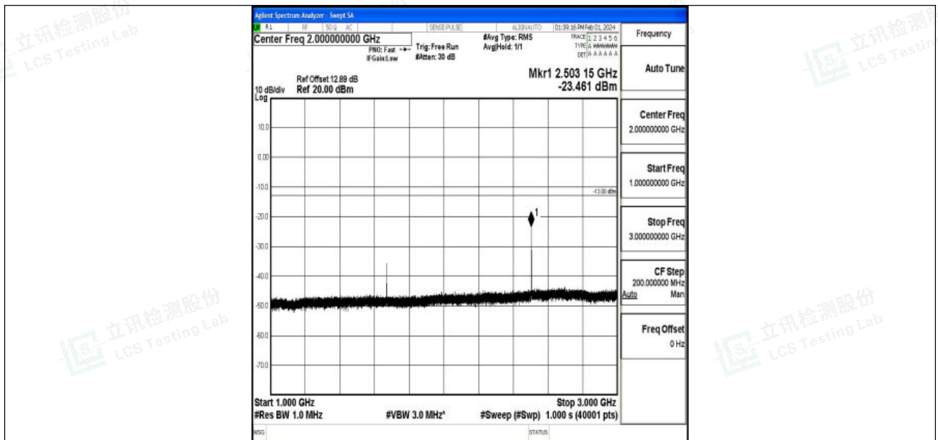
Band5_5MHz_16QAM_20525_1RB#0_1000~3000_1000~3000
