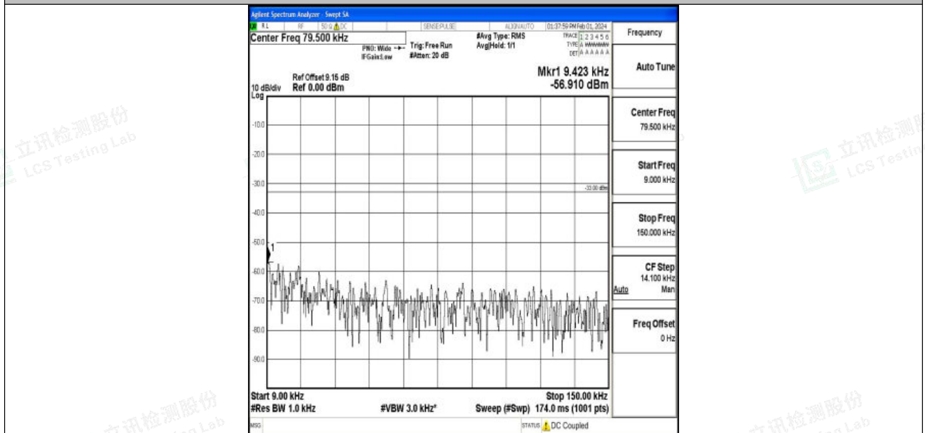
Band5_5MHz_16QAM_20425_1RB#0_0.009~0.15_0.009~0.15
