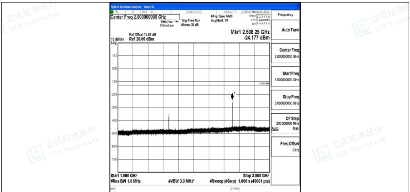
Band5_1.4MHz_16QAM_20525_1RB#0_1000~3000_1000~3000
