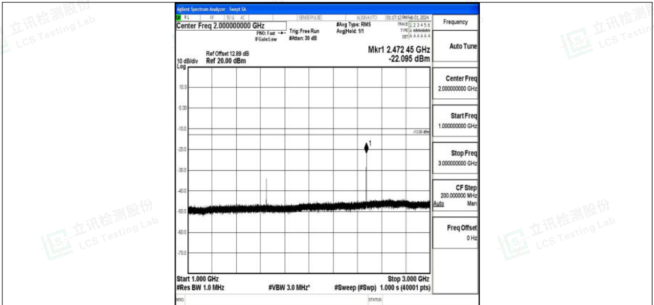
Band5_3MHz_16QAM_20415_1RB#0_1000~3000_1000~3000
