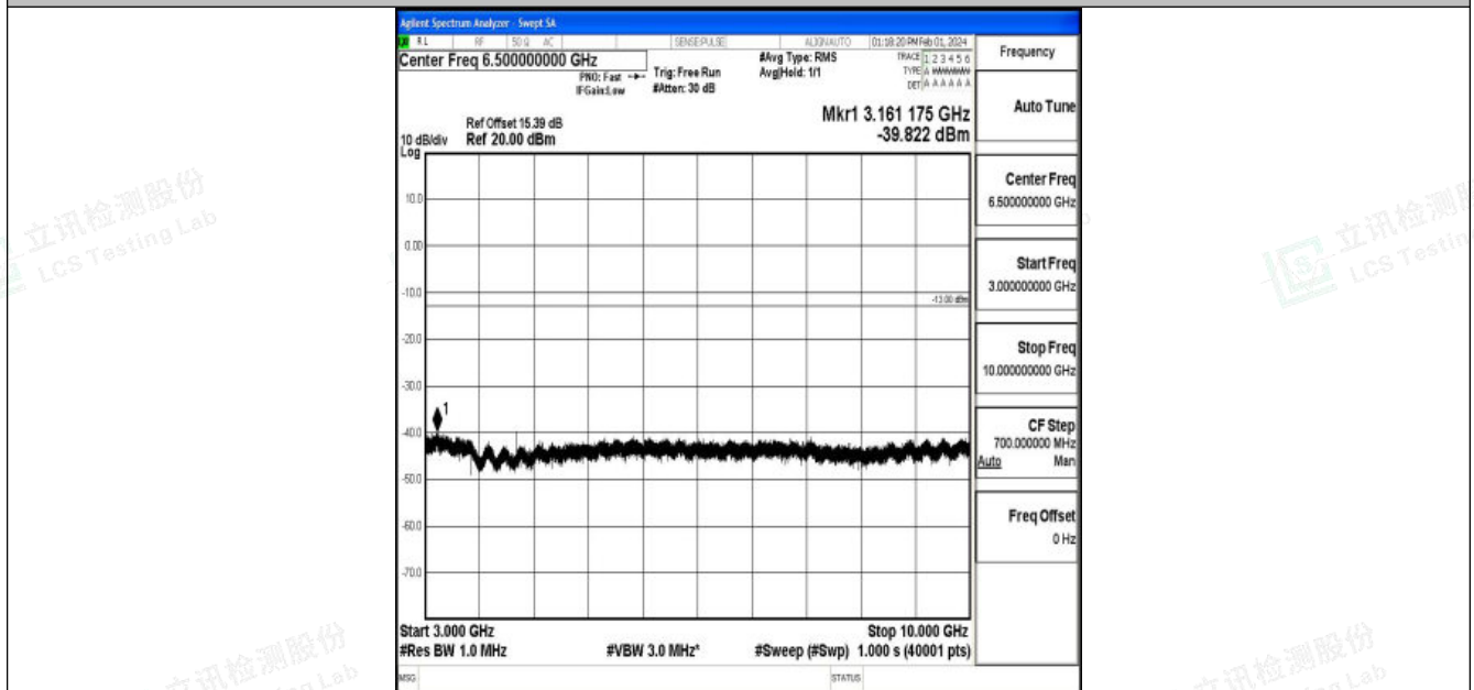
Band5_3MHz_16QAM_20525_1RB#0_3000~10000_3000~10000
