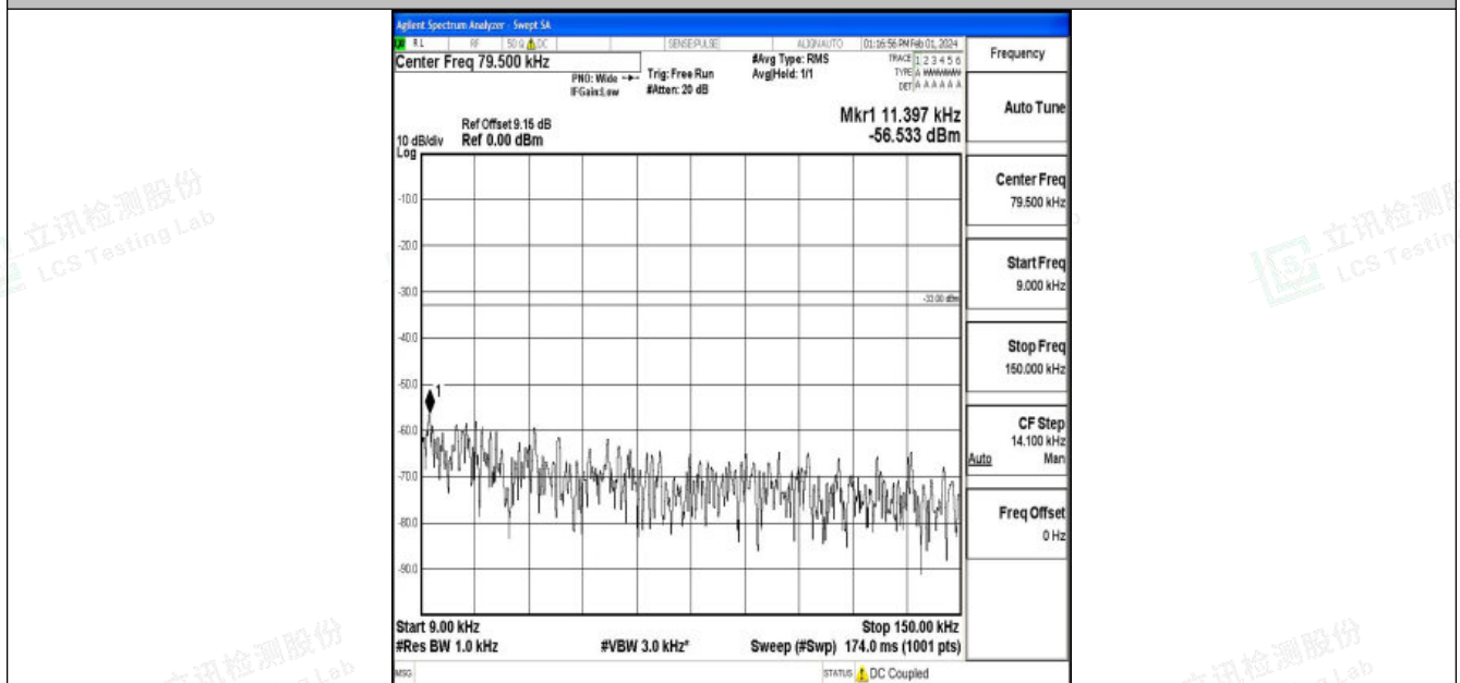
Band5_3MHz_16QAM_20415_1RB#0_0.009~0.15_0.009~0.15
