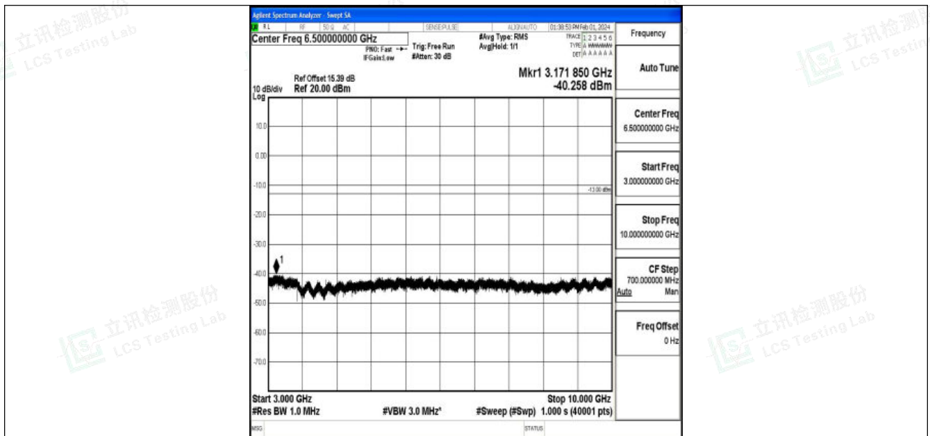
Band5_5MHz_QPSK_20525_1RB#0_3000~10000_3000~10000
