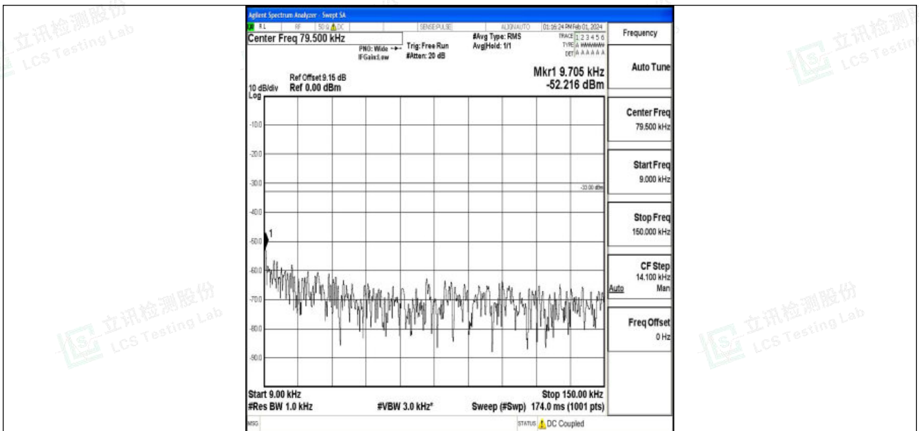
Band5_3MHz_QPSK_20415_1RB#0_0.009~0.15_0.009~0.15
