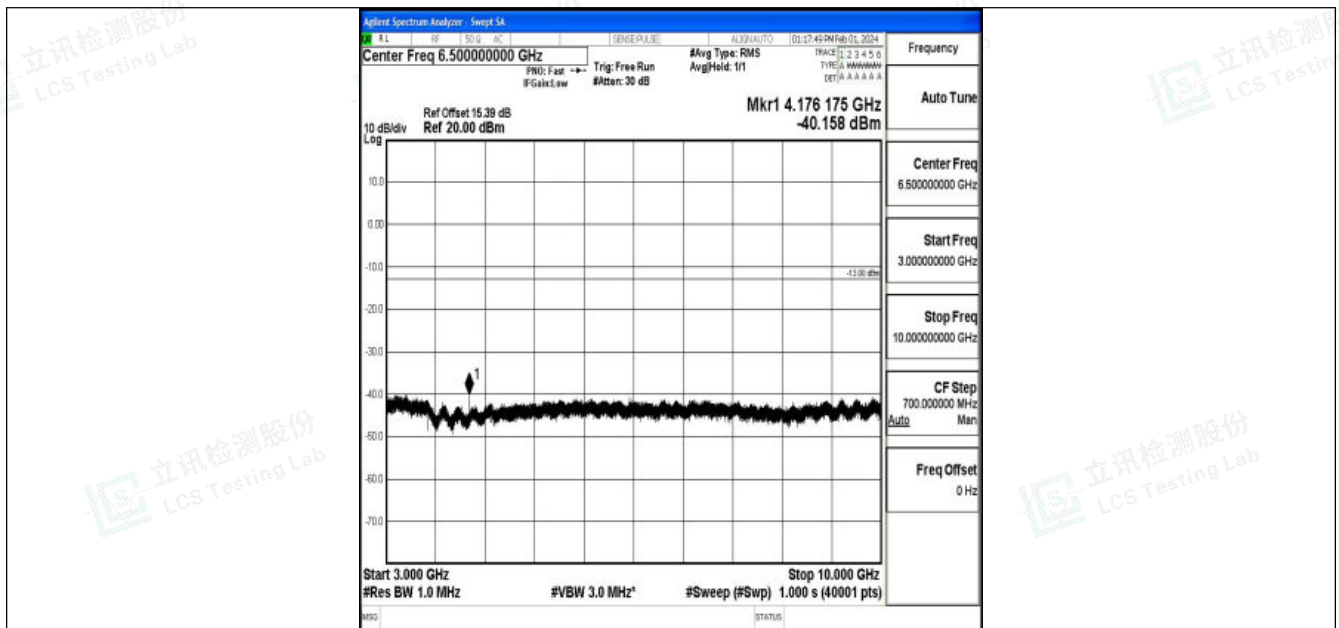
Band5_3MHz_QPSK_20525_1RB#0_3000~10000_3000~10000
