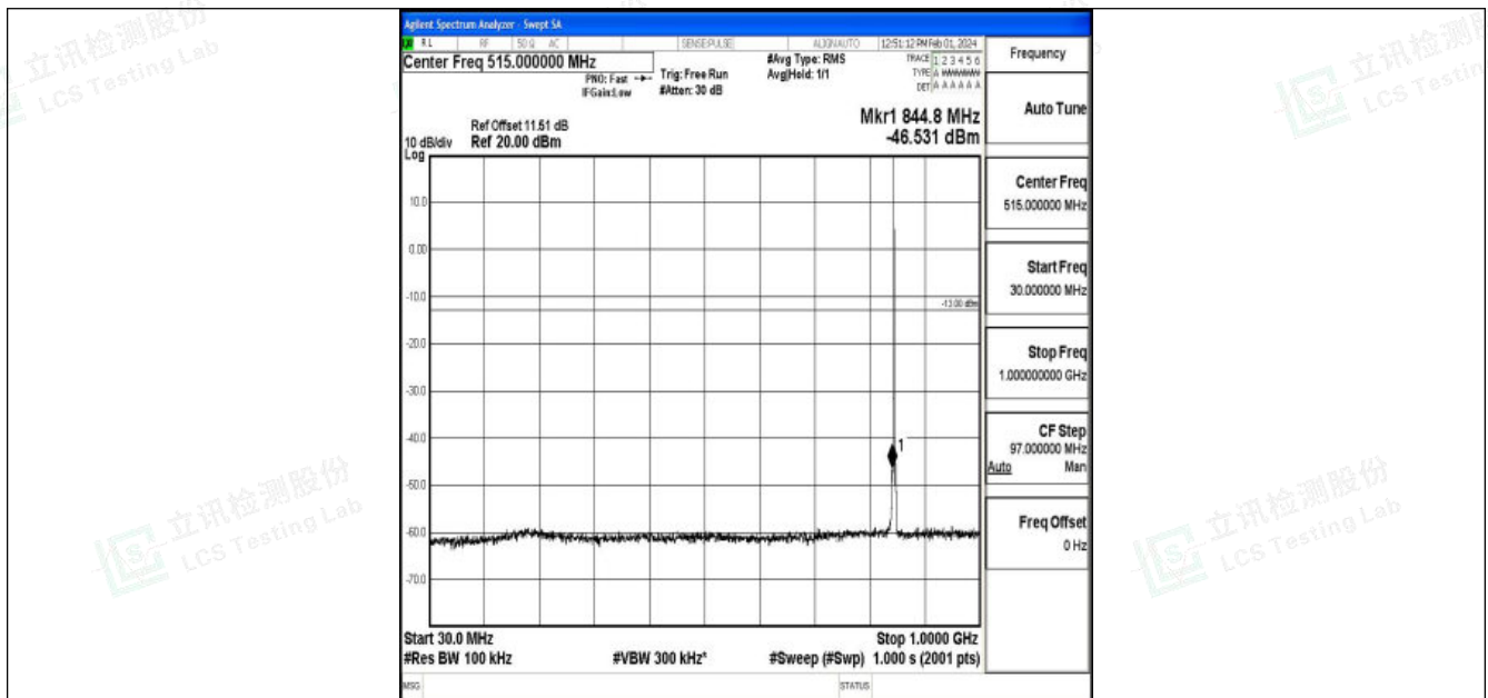
Band5_1.4MHz_QPSK_20643_1RB#0_30~1000_30~1000
