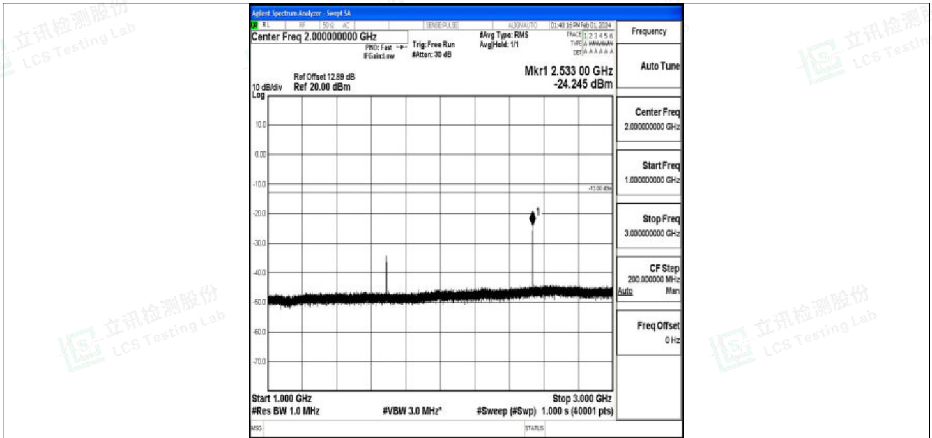
Band5_5MHz_16QAM_20625_1RB#0_1000~3000_1000~3000
