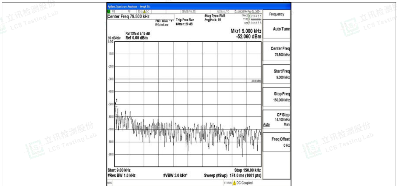
Band5_3MHz_QPSK_20635_1RB#0_0.009~0.15_0.009~0.15
