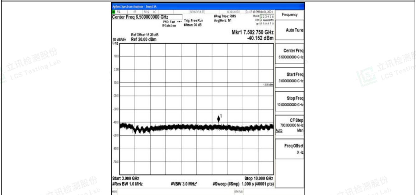
Band5_3MHz_16QAM_20415_1RB#0_3000~10000_3000~10000
