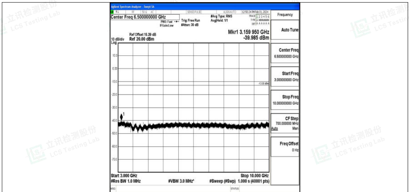
Band5_1.4MHz_QPSK_20525_1RB#0_3000~10000_3000~10000
