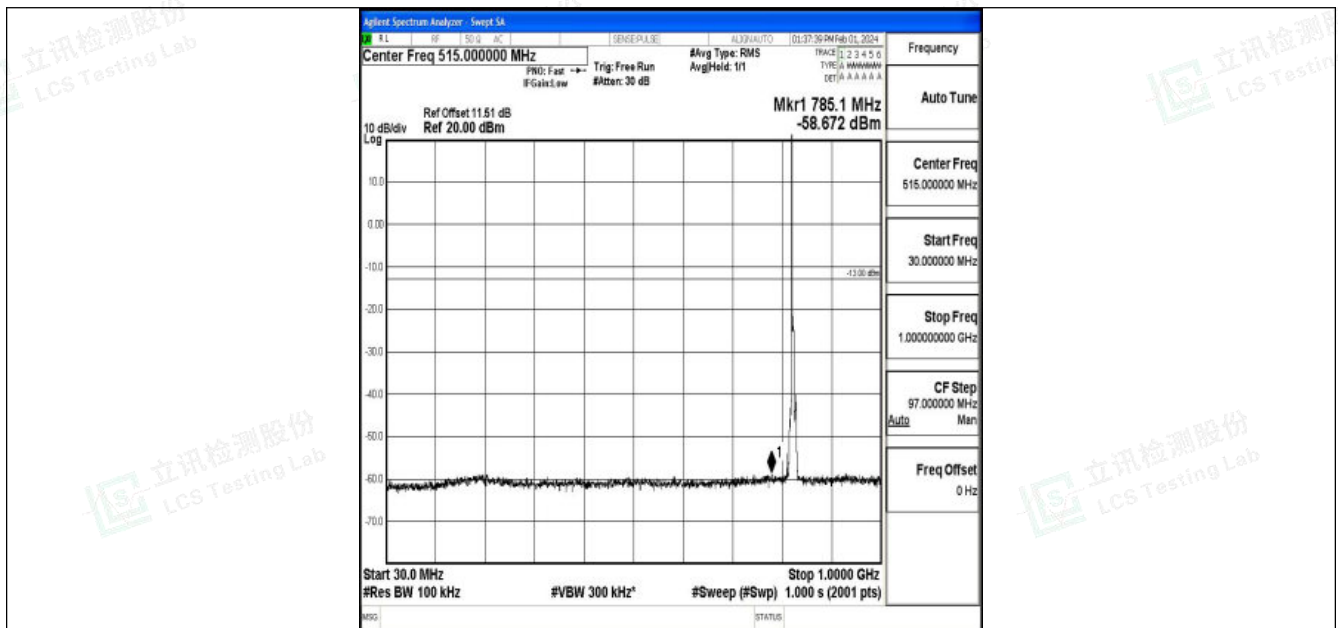
Band5_5MHz_QPSK_20425_1RB#0_30~1000_30~1000
