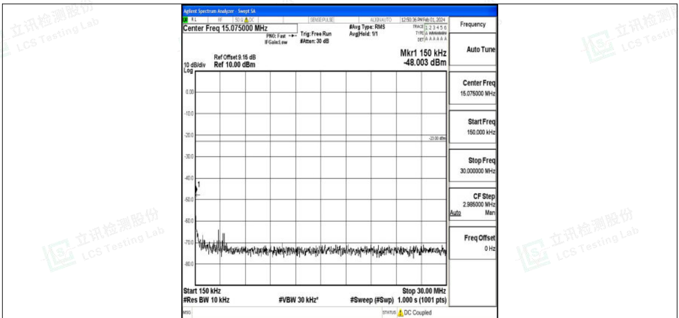
Band5_1.4MHz_16QAM_20525_1RB#0_0.15~30_0.15~30
