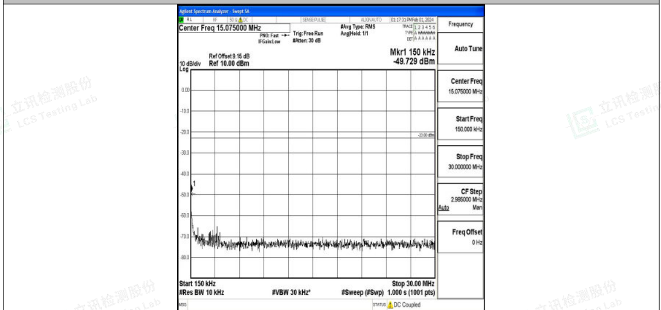
Band5_3MHz_QPSK_20525_1RB#0_0.15~30_0.15~30
