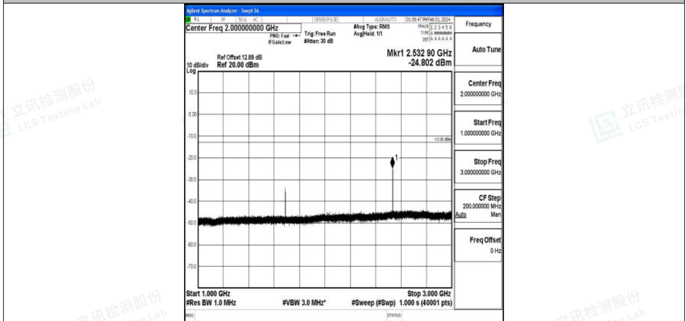
Band5_5MHz_QPSK_20625_1RB#0_1000~3000_1000~3000
