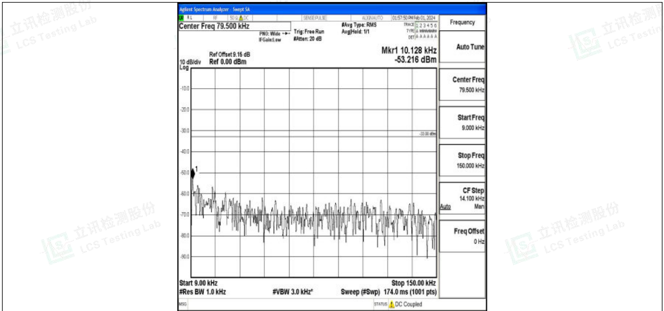
Band5_10MHz_QPSK_20450_1RB#0_0.009~0.15_0.009~0.15
