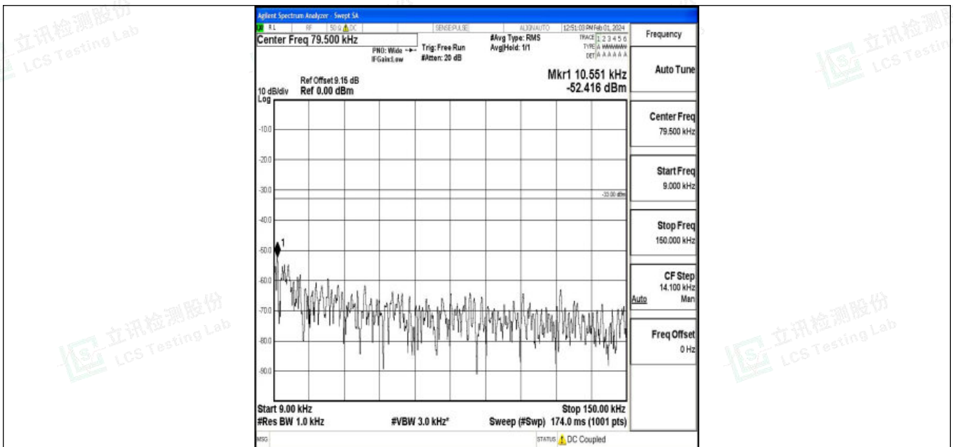
Band5_1.4MHz_QPSK_20643_1RB#0_0.009~0.15_0.009~0.15
