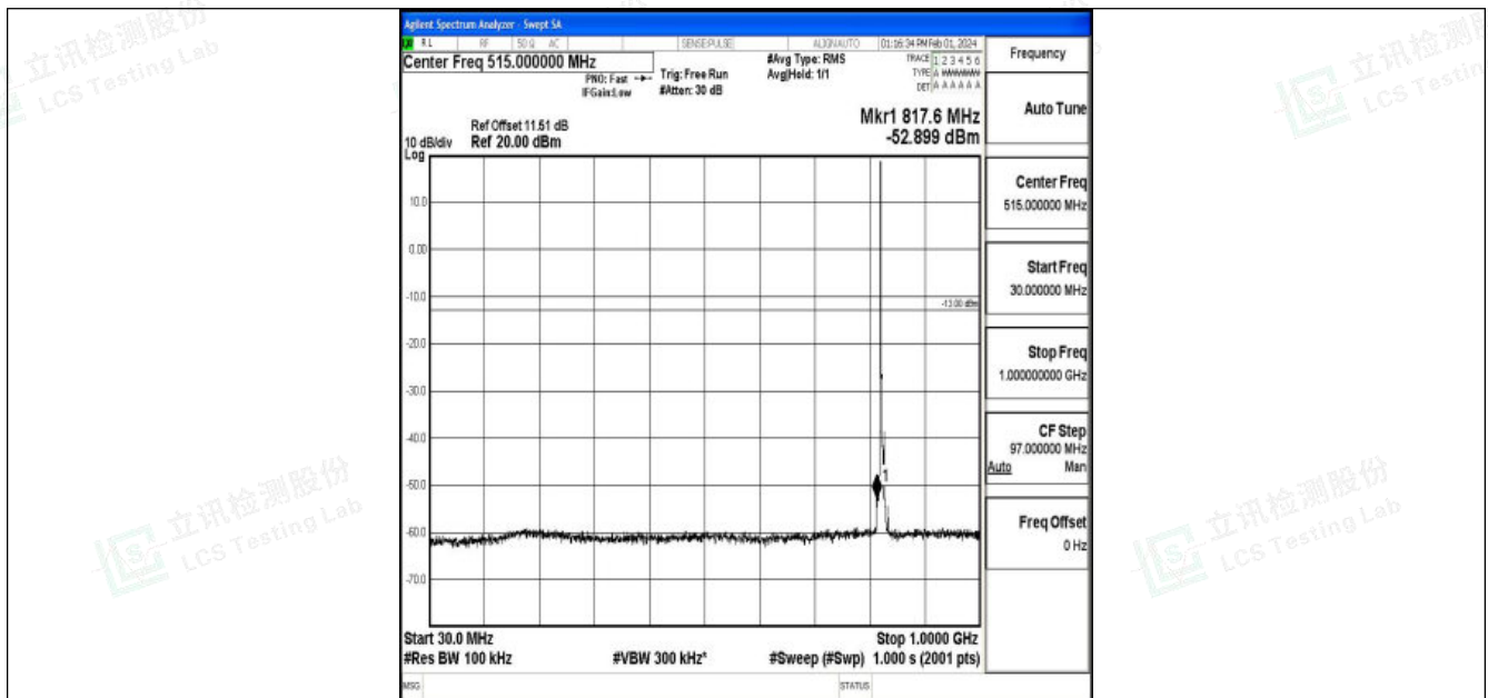
Band5_3MHz_QPSK_20415_1RB#0_30~1000_30~1000
