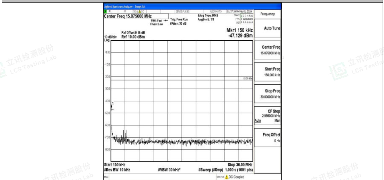
Band5_5MHz_QPSK_20425_1RB#0_0.15~30_0.15~30
