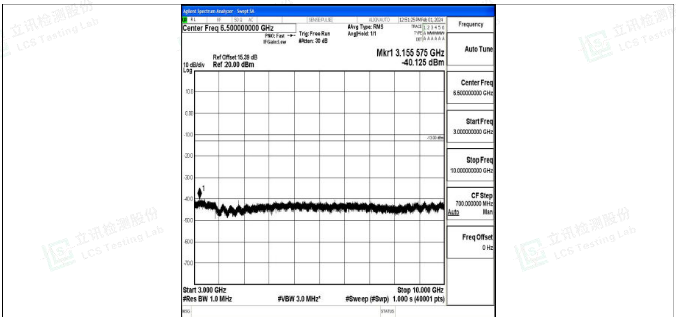
Band5_1.4MHz_QPSK_20643_1RB#0_3000~10000_3000~10000
