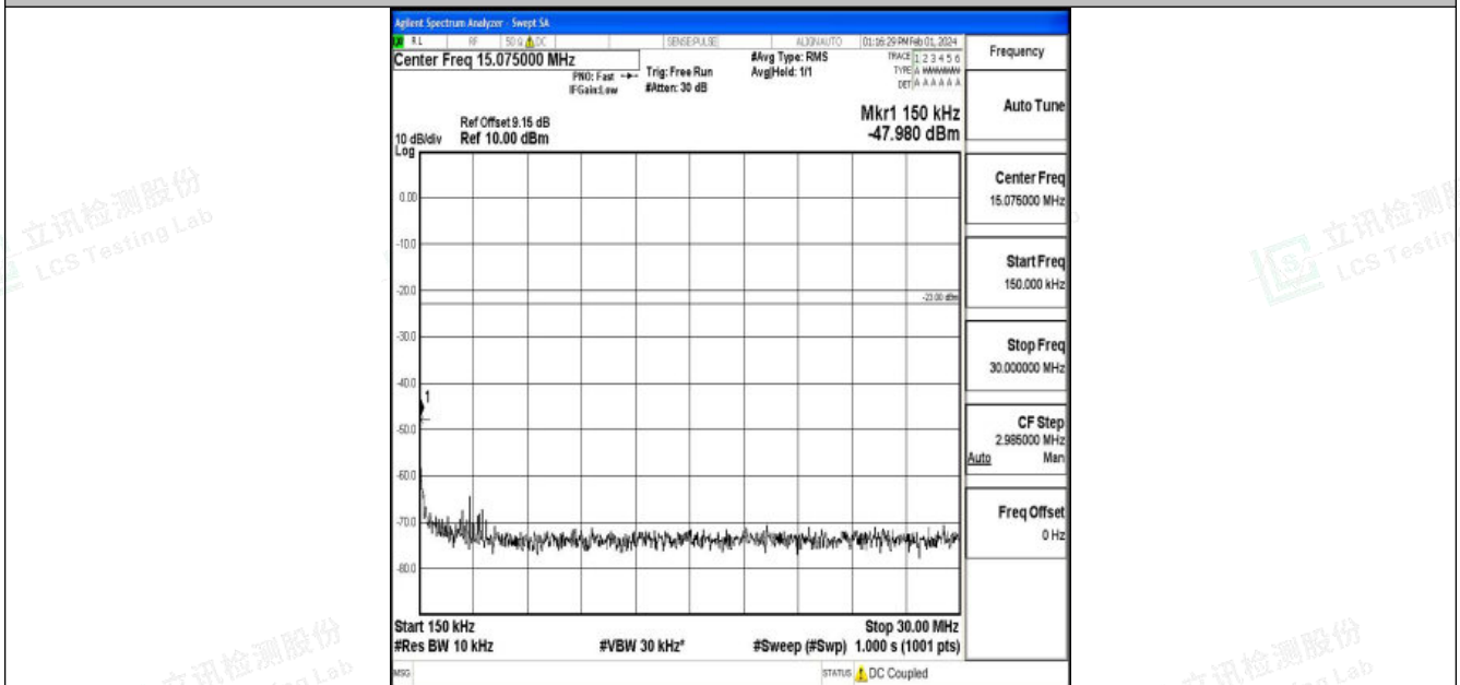
Band5_3MHz_QPSK_20415_1RB#0_0.15~30_0.15~30
