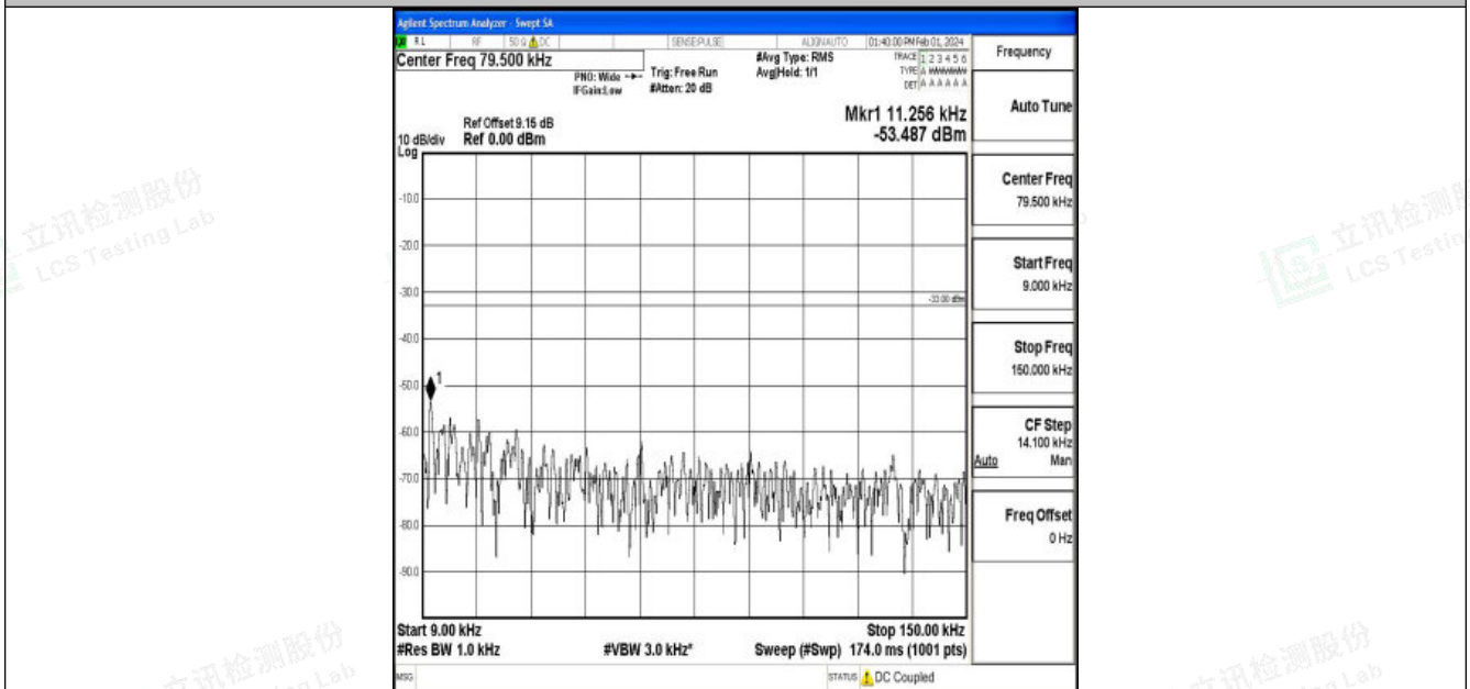
Band5_5MHz_16QAM_20625_1RB#0_0.009~0.15_0.009~0.15
