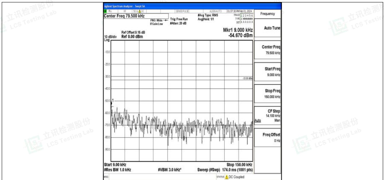
Band5_5MHz_QPSK_20425_1RB#0_0.009~0.15_0.009~0.15
