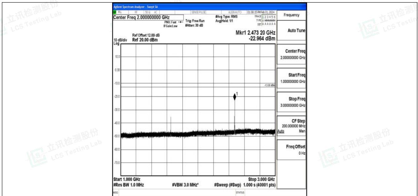
Band5_5MHz_16QAM_20425_1RB#0_1000~3000_1000~3000
