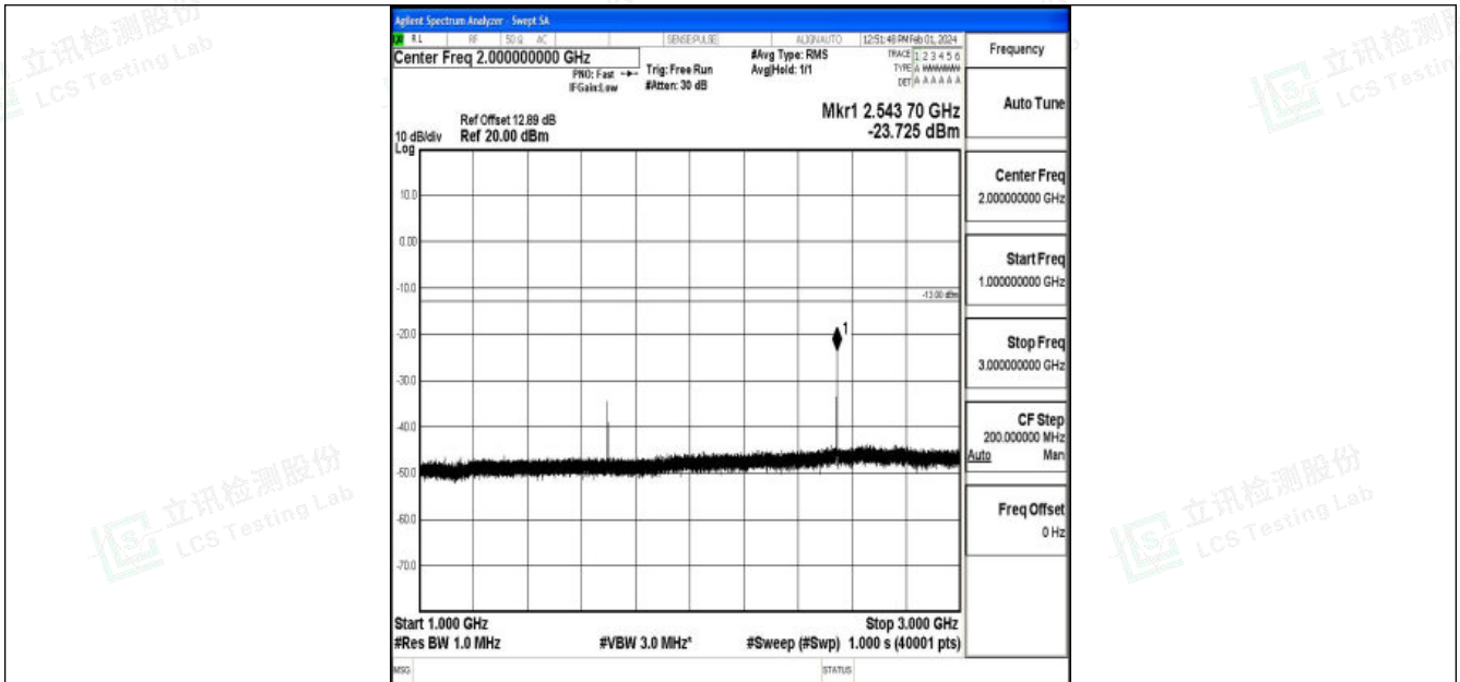
Band5_1.4MHz_16QAM_20643_1RB#0_1000~3000_1000~3000
