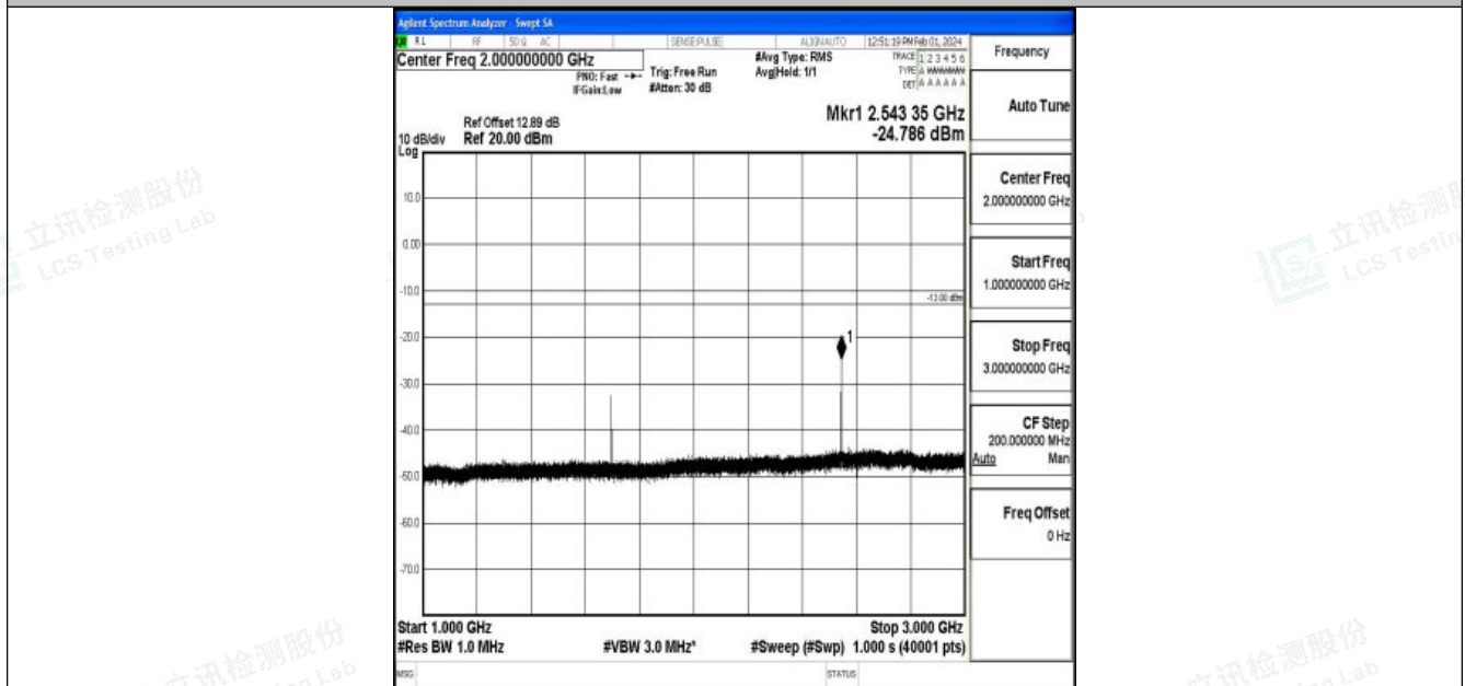
Band5_1.4MHz_QPSK_20643_1RB#0_1000~3000_1000~3000
