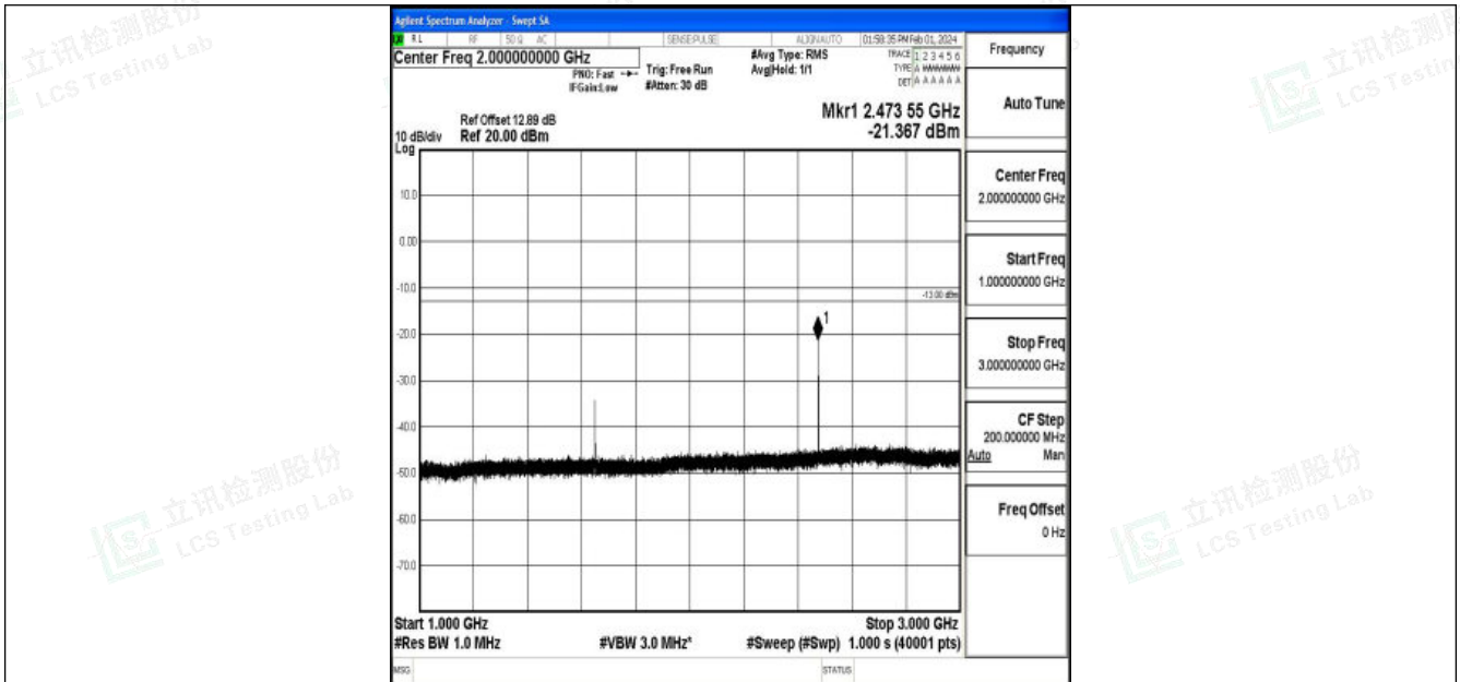
Band5_10MHz_16QAM_20450_1RB#0_1000~3000_1000~3000
