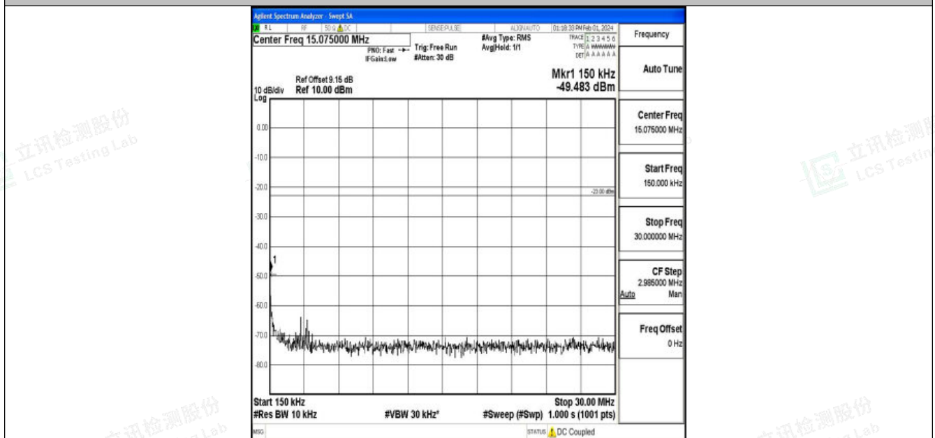
Band5_3MHz_QPSK_20635_1RB#0_0.15~30_0.15~30
