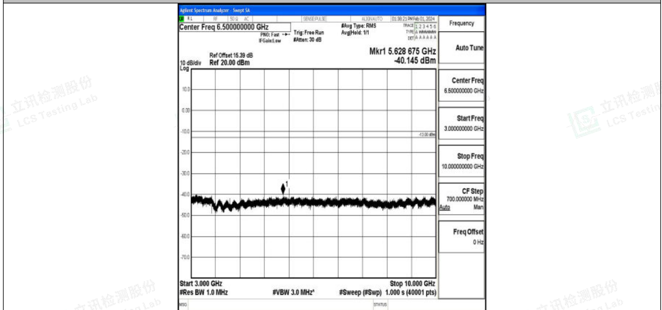
Band5_5MHz_16QAM_20425_1RB#0_3000~10000_3000~10000
