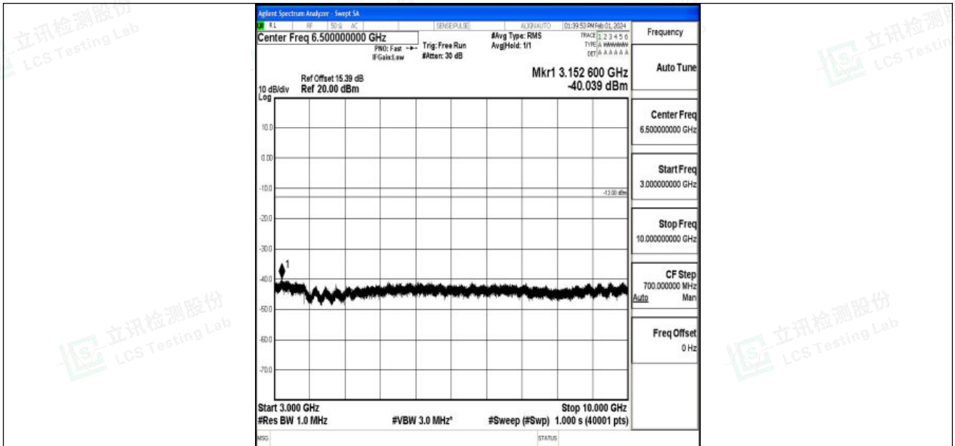
Band5_5MHz_QPSK_20625_1RB#0_3000~10000_3000~10000
