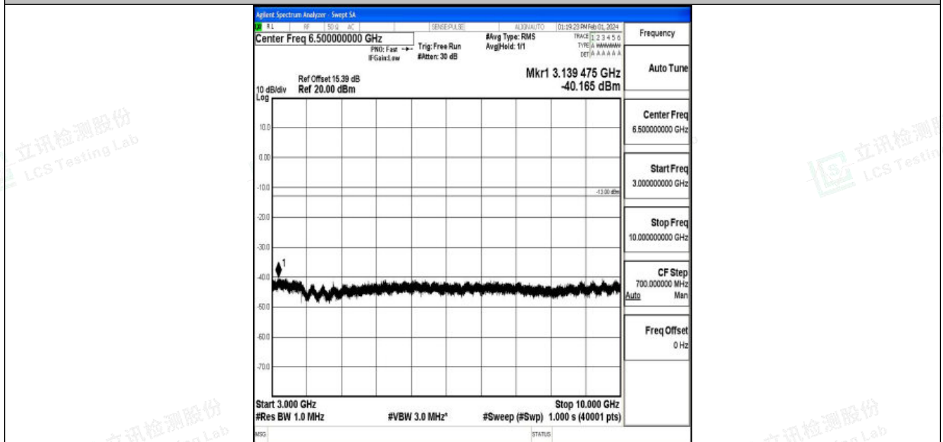
Band5_3MHz_16QAM_20635_1RB#0_3000~10000_3000~10000
