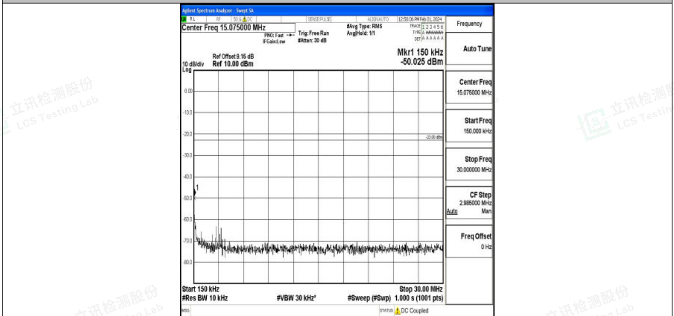
Band5_1.4MHz_QPSK_20525_1RB#0_0.15~30_0.15~30
