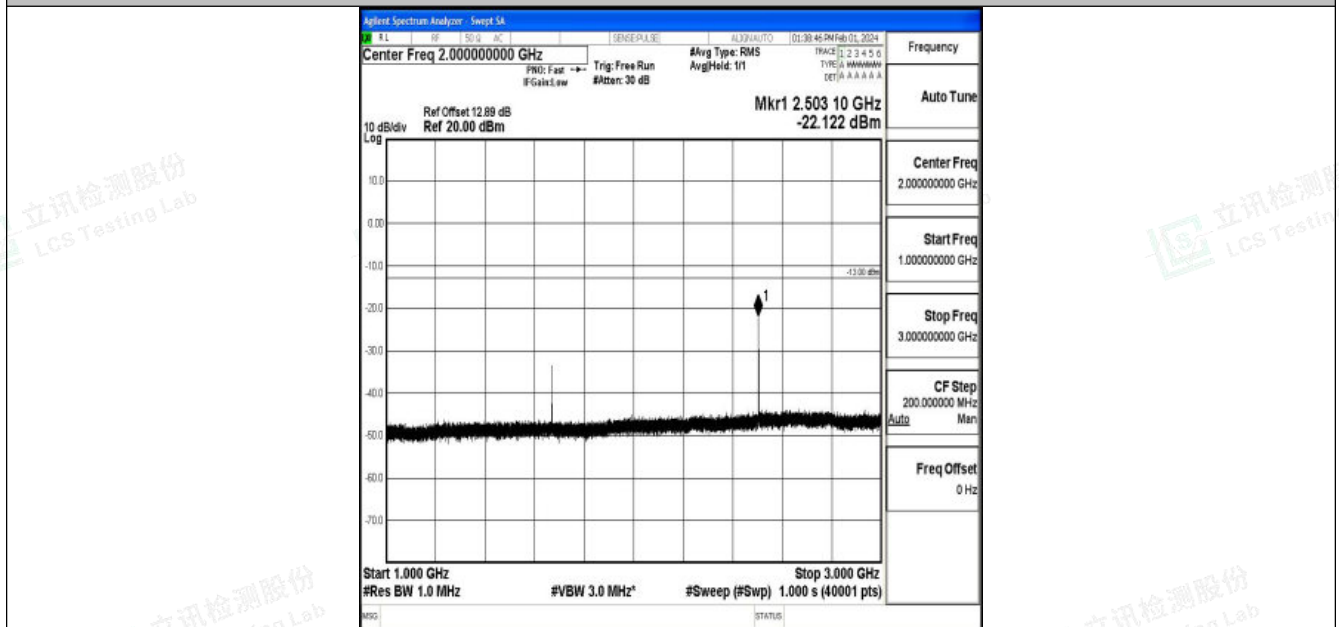
Band5_5MHz_QPSK_20525_1RB#0_1000~3000_1000~3000
