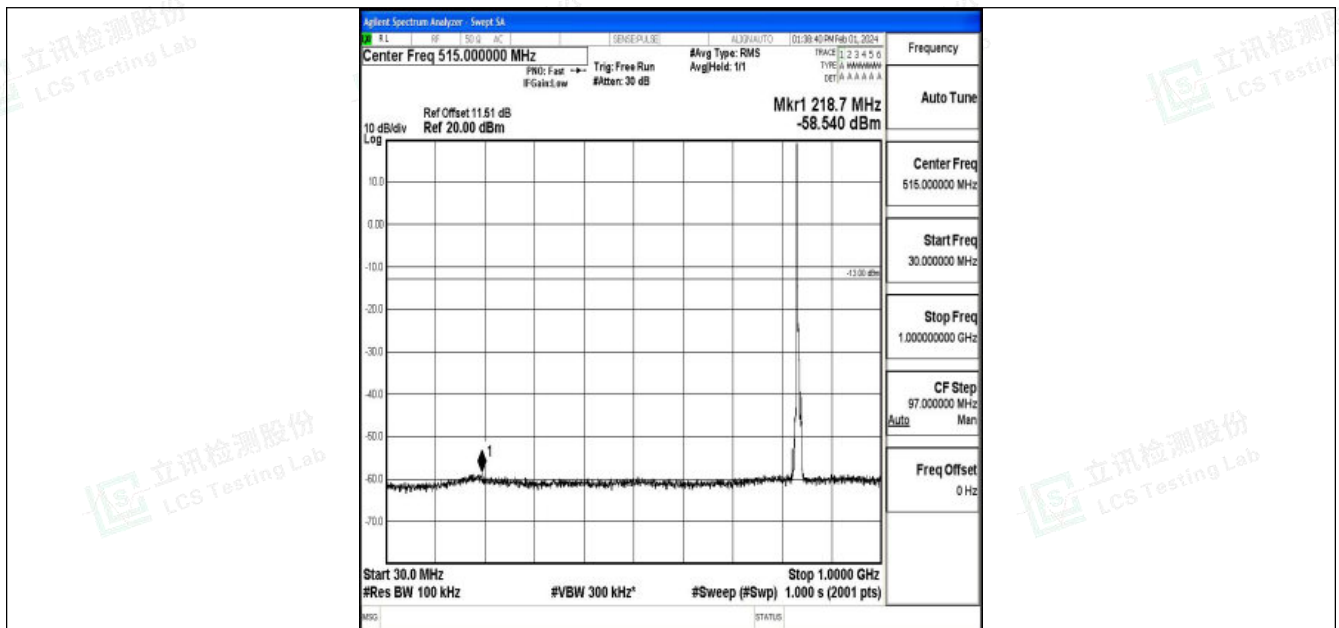
Band5_5MHz_QPSK_20525_1RB#0_30~1000_30~1000
