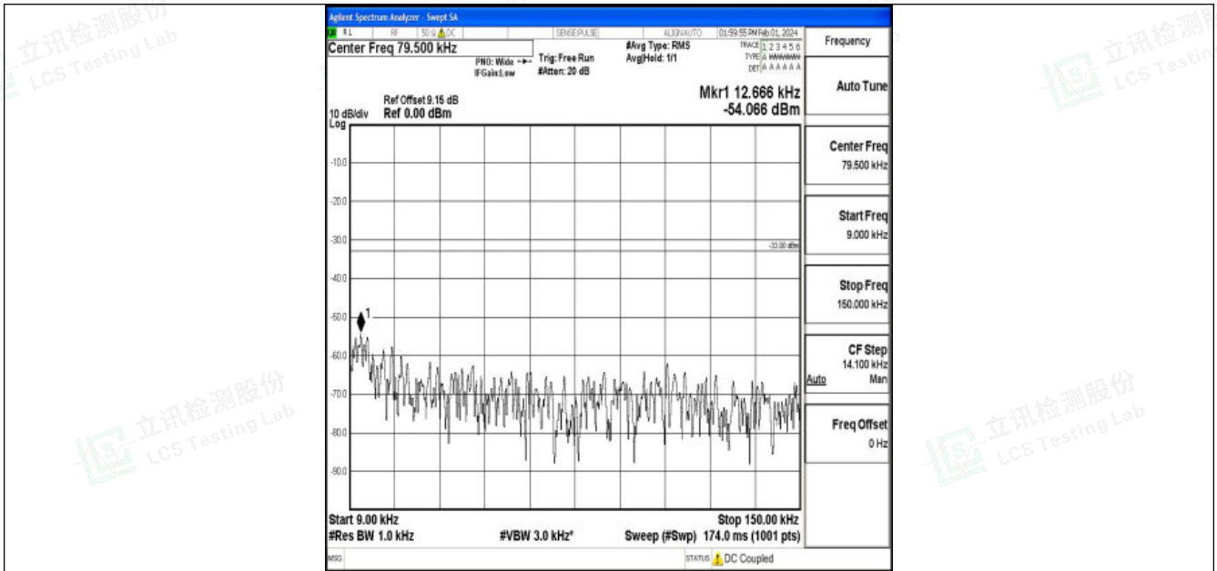
Band5_10MHz_QPSK_20600_1RB#0_0.009~0.15_0.009~0.15
