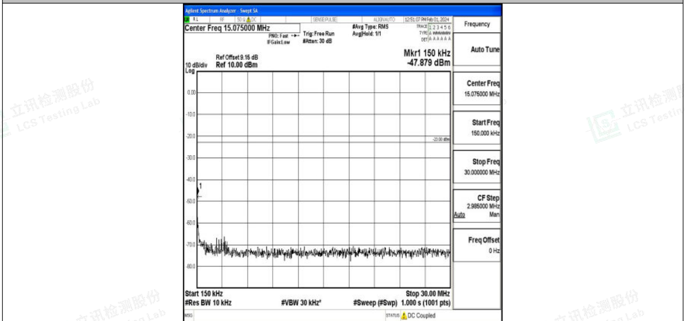
Band5_1.4MHz_QPSK_20643_1RB#0_0.15~30_0.15~30
