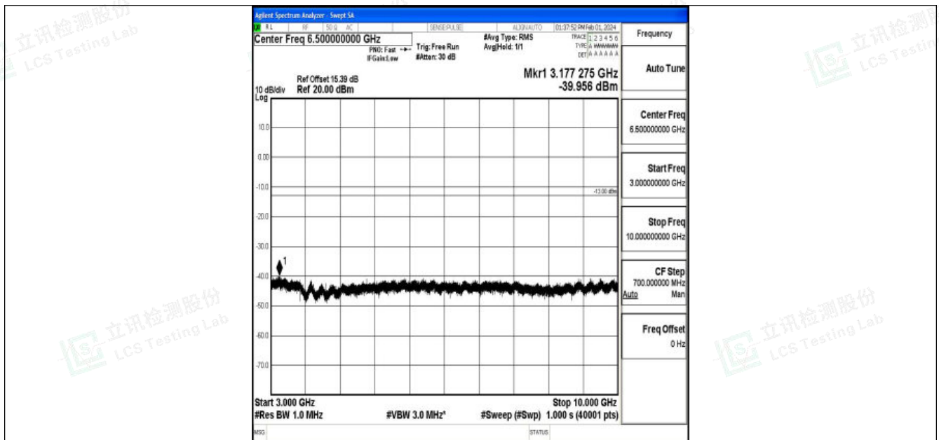
Band5_5MHz_QPSK_20425_1RB#0_3000~10000_3000~10000
