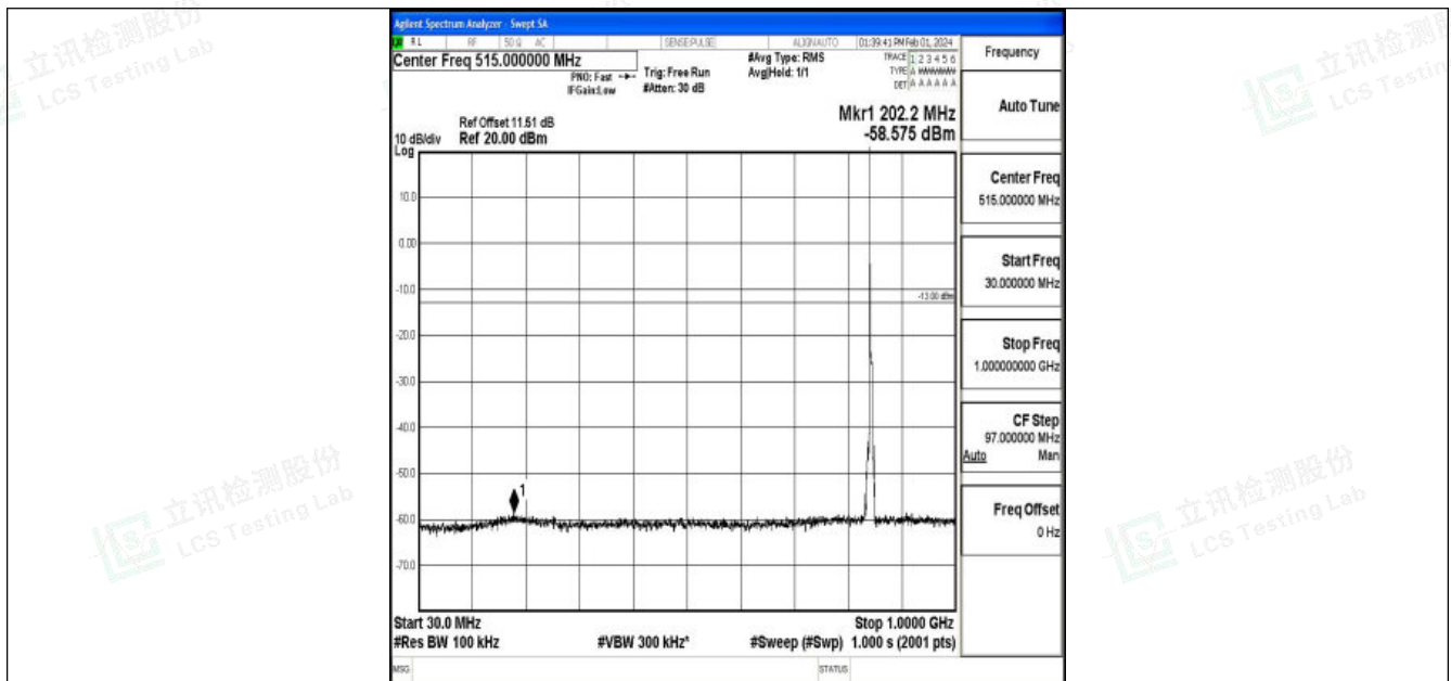
Band5_5MHz_QPSK_20625_1RB#0_30~1000_30~1000
