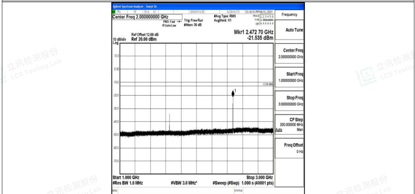
Band5_3MHz_QPSK_20415_1RB#0_1000~3000_1000~3000
