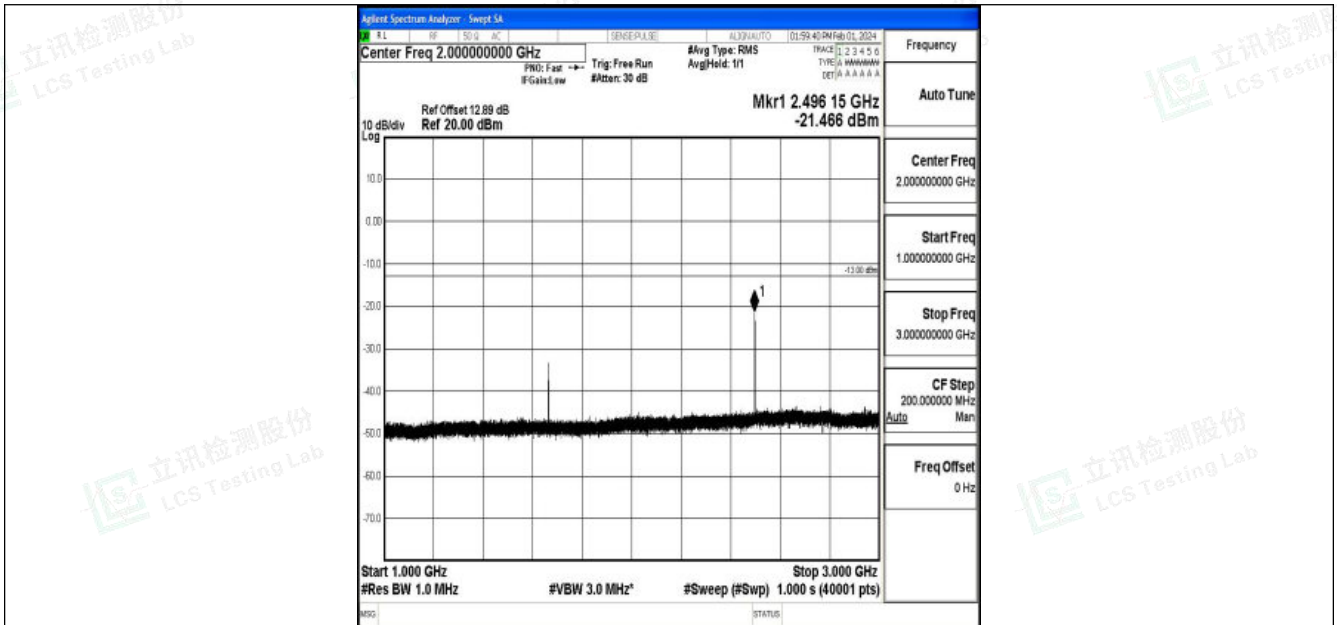
Band5_10MHz_16QAM_20525_1RB#0_1000~3000_1000~3000
