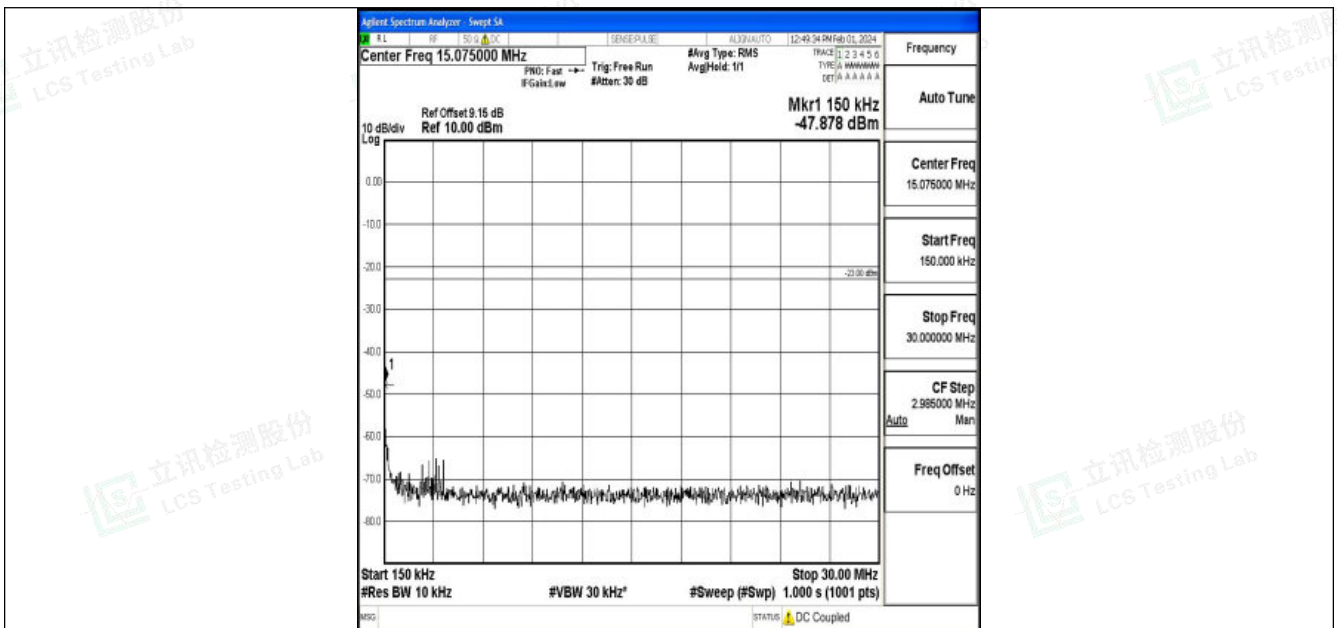
Band5_1.4MHz_16QAM_20407_1RB#0_0.15~30_0.15~30
