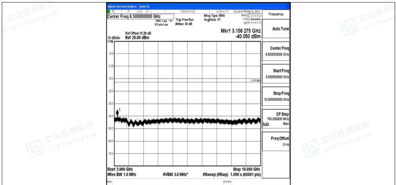
Band5_3MHz_QPSK_20415_1RB#0_3000~10000_3000~10000
