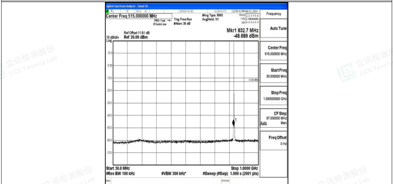
Band5_1.4MHz_16QAM_20525_1RB#0_30~1000_30~1000
