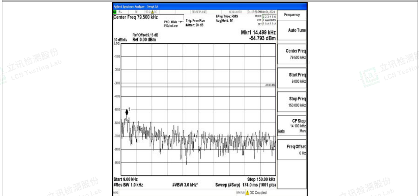
Band5_3MHz_16QAM_20525_1RB#0_0.009~0.15_0.009~0.15
