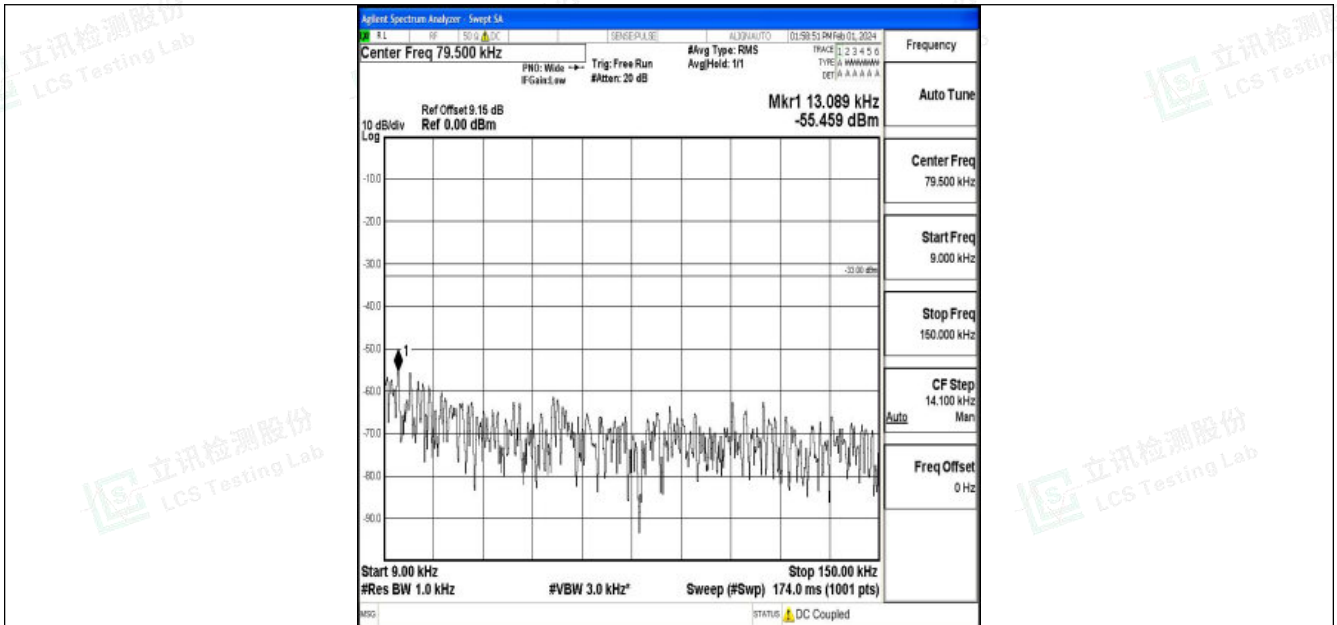
Band5_10MHz_QPSK_20525_1RB#0_0.009~0.15_0.009~0.15
