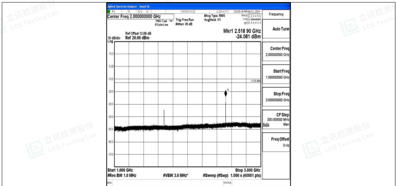
Band5_10MHz_16QAM_20600_1RB#0_1000~3000_1000~3000
