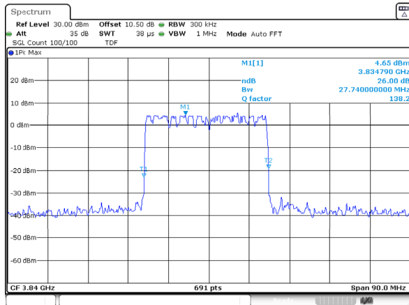
n77_3_30MHz_30kHz_3840MHz_DFT-s-OFDM QPSK_RB75@0 26 dB Emission Bandwidth
