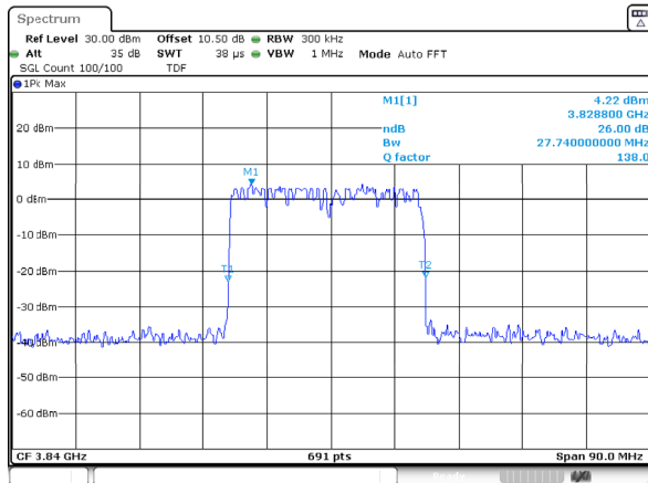
n77_3_30MHz_30kHz_3840MHz_DFT-s-OFDM 16 QAM_RB75@0 26 dB Emission Bandwidth
