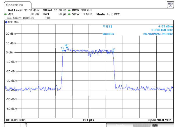
n77_3_30MHz_30kHz_3840MHz_DFT-s-OFDM 64 QAM_RB75@0 Occupied Bandwidth
