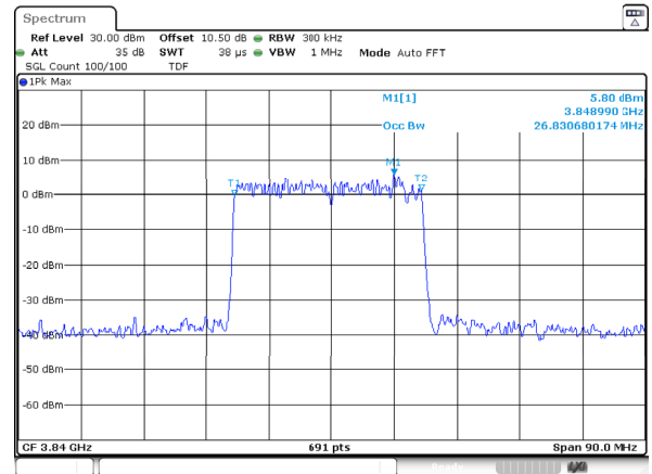
n77_3_30MHz_30kHz_3840MHz_DFT-s-OFDM 16 QAM_RB75@0 Occupied Bandwidth
