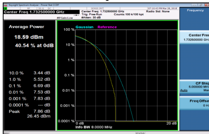
LTE_Band4_20MHz_16QAM_100_0_MidCH20175-1732.5
