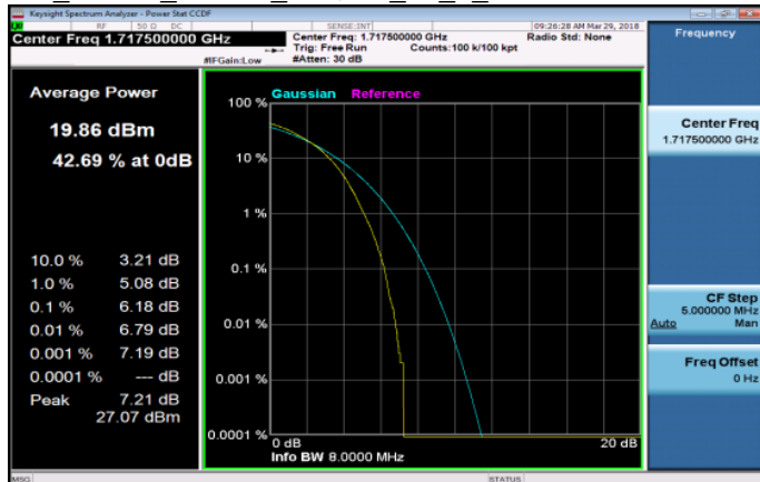
LTE_Band4_15MHz_16QAM_75_0_LowCH20025-1717.5
