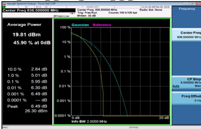
LTE_Band5_1_4MHz_16QAM_6_0_MidCH20525-836.5
