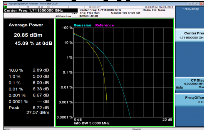
LTE_Band4_3MHz_16QAM_15_0_LowCH19965-1711.5
