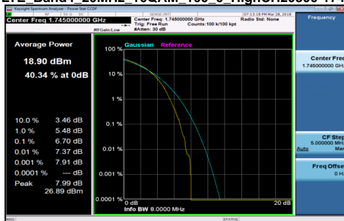
LTE_Band4_20MHz_16QAM_100_0_HighCH20300-1745
