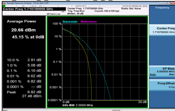
LTE_Band4_1_4MHz_16QAM_6_0_LowCH19957-1710.7
