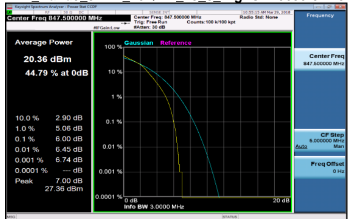
LTE_Band5_3MHz_16QAM_15_0_HighCH20635-847.5
