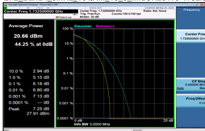
LTE_Band4_3MHz_16QAM_15_0_MidCH20175-1732.5
