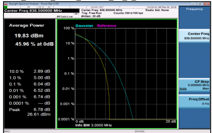
LTE_Band5_3MHz_16QAM_15_0_MidCH20525-836.5
