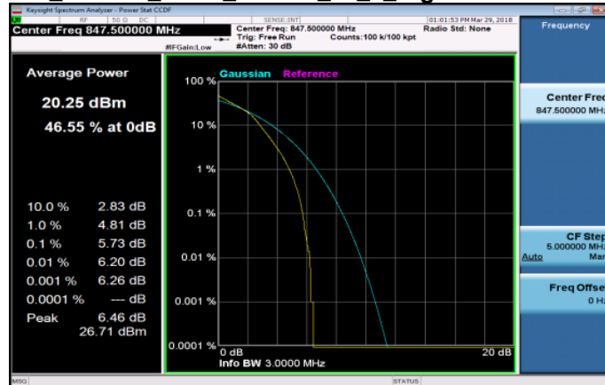
LTE_Band26_3MHz_16QAM_15_0_HighCH27025-847.5
