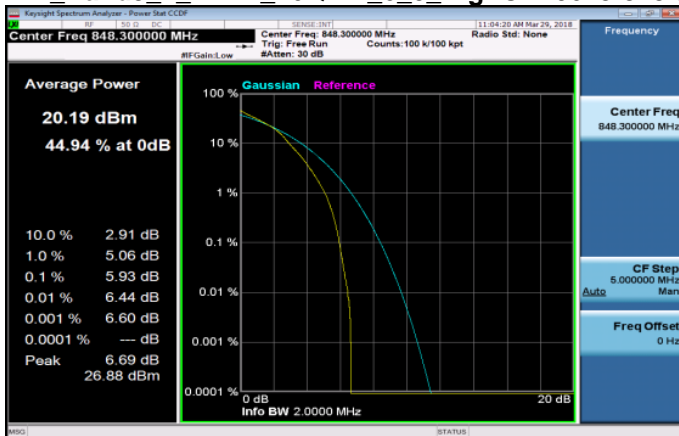
LTE_Band5_1_4MHz_16QAM_6_0_HighCH20643-848.3
