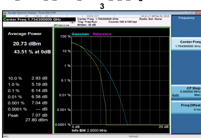
LTE_Band4_1_4MHz_16QAM_6_0_HighCH20393-1754.3
