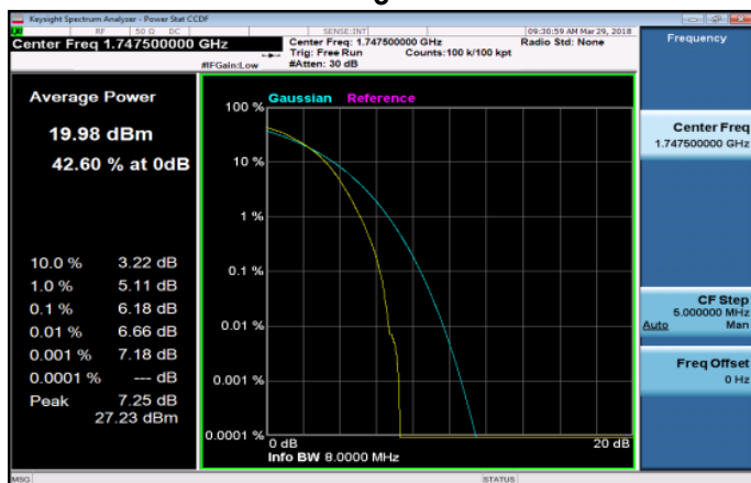
LTE_Band4_15MHz_16QAM_75_0_HighCH20325-1747.5
