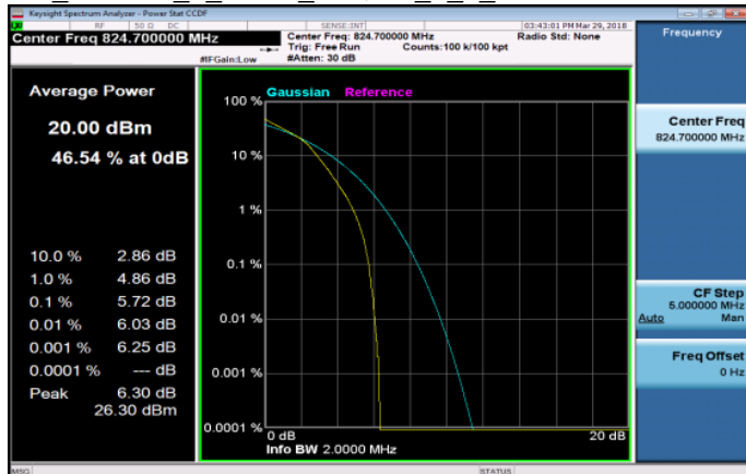
LTE_Band26_1_4MHz_16QAM_6_0_LowCH26797-824.7
