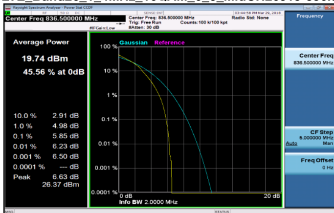
LTE_Band26_1_4MHz_16QAM_6_0_MidCH26915-836.5
