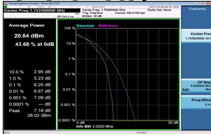
LTE_Band4_3MHz_16QAM_15_0_HighCH20385-1753.5
