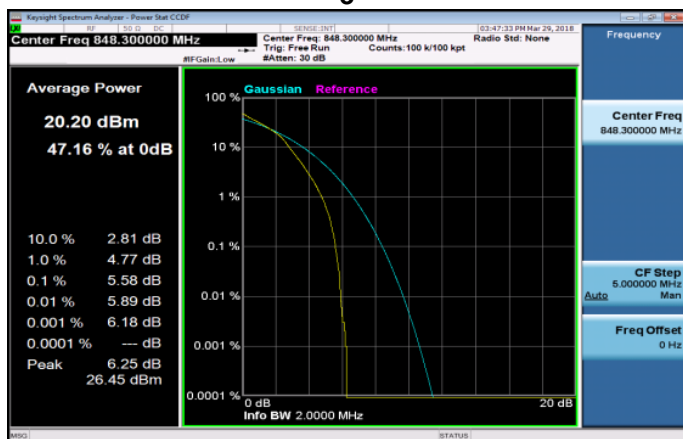
LTE_Band26_1_4MHz_16QAM_6_0_HighCH27033-848.
