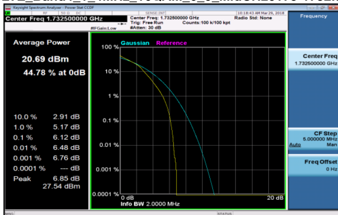
LTE_Band4_1_4MHz_16QAM_6_0_MidCH20175-1732.5
