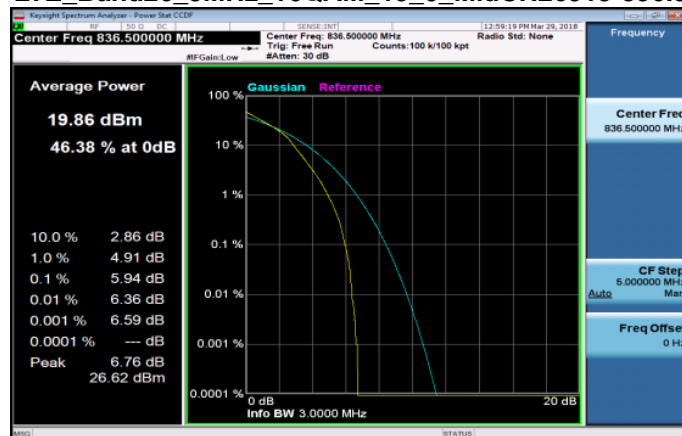
LTE_Band26_3MHz_16QAM_15_0_MidCH26915-836.5
