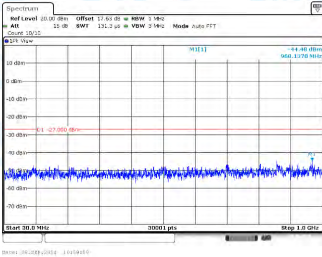
11AC20-CDD-Ant3-5240-30~1000-PASS
