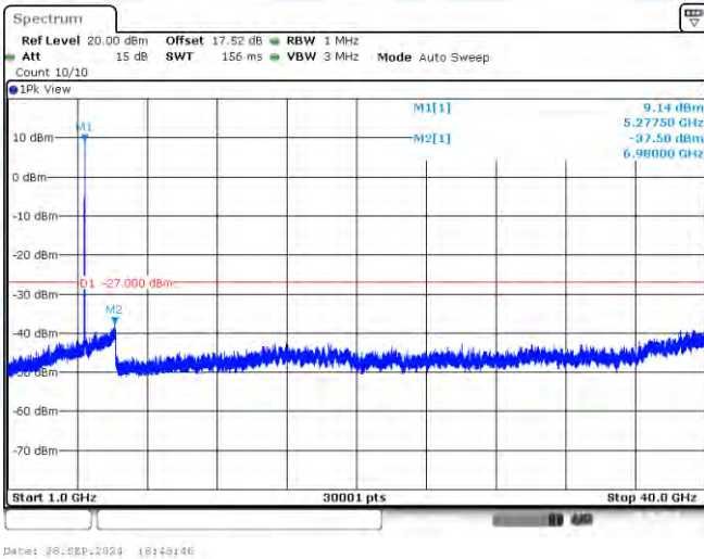
11AC20-CDD-Ant2-5280-1000~40000-PASS
