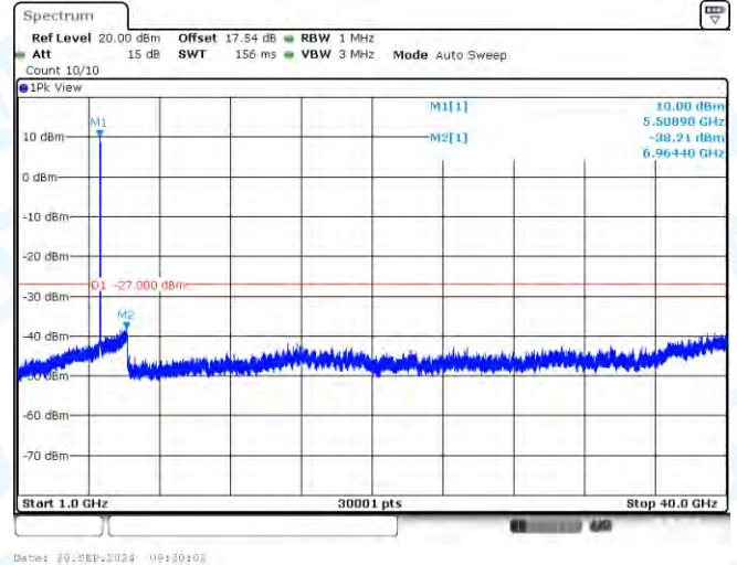
11N40-CDD-Ant1-5510-1000~40000-PASS
