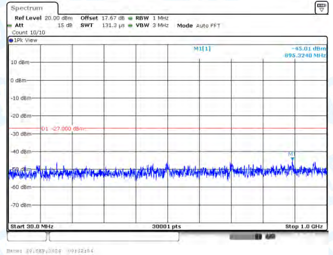
11N40-CDD-Ant2-5550-30~1000-PASS
