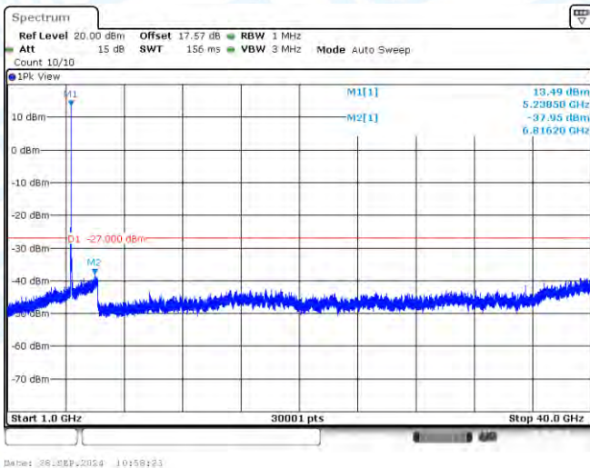
11AC20-CDD-Ant2-5240-1000~40000-PASS
