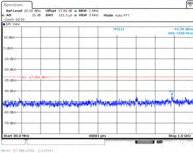
11N40-CDD-Ant1-5795-30~1000-PASS
