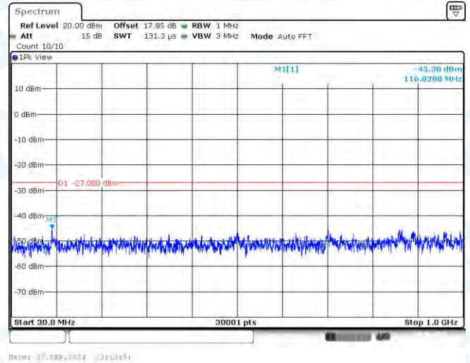
11AC20-CDD-Ant2-5825-30~1000-PASS
