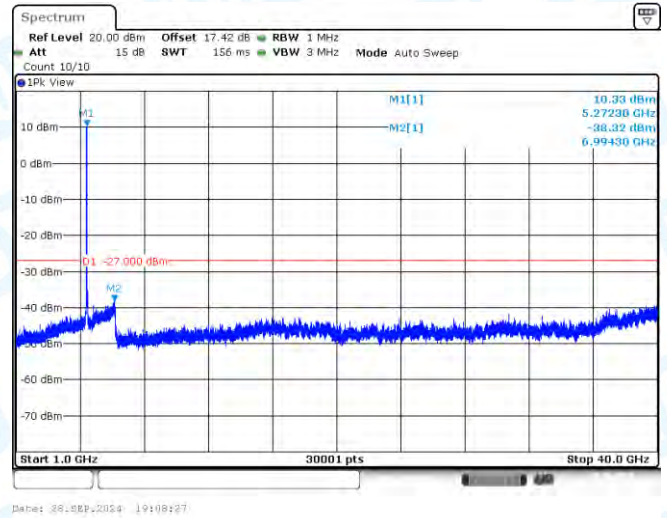
11AC40-CDD-Ant1-5270-1000~40000-PASS
