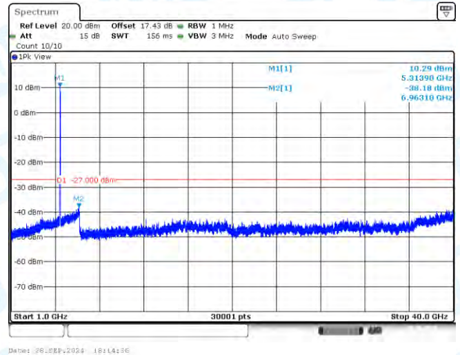
11N40-CDD-Ant1-5310-1000~40000-PASS
