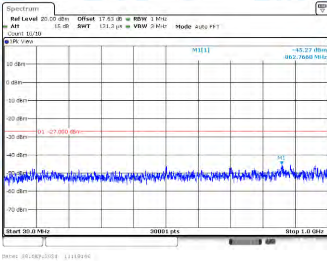
11AC40-CDD-Ant3-5230-30~1000-PASS
