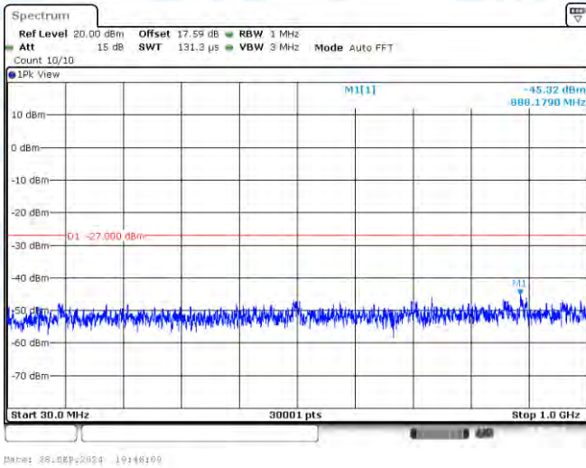
11AC80-CDD-Ant3-5290-30~1000-PASS
