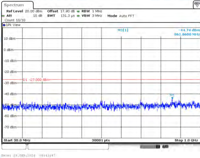
11N40-CDD-Ant1-5710-30~1000-PASS
