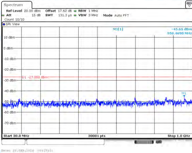
11N40-CDD-Ant1-5550-30~1000-PASS
