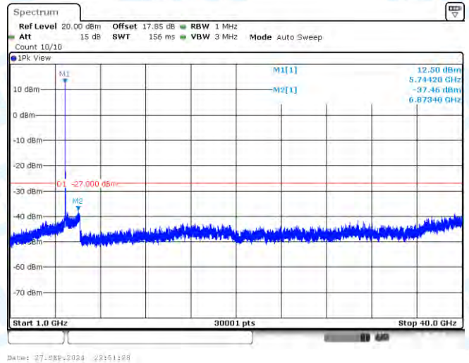
11AC20-CDD-Ant3-5745-1000~40000-PASS
