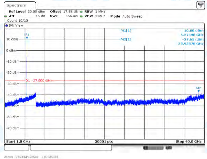
11AC20-CDD-Ant3-5280-1000~40000-PASS
