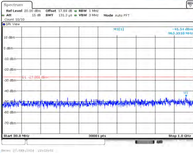
11AC40-CDD-Ant1-5795-30~1000-PASS
