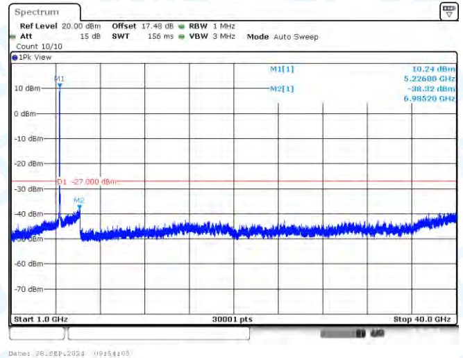
11N40-CDD-Ant1-5230-1000~40000-PASS
