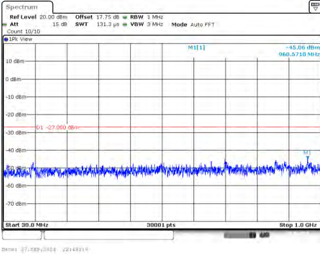
11AC20-CDD-Ant2-5745-30~1000-PASS
