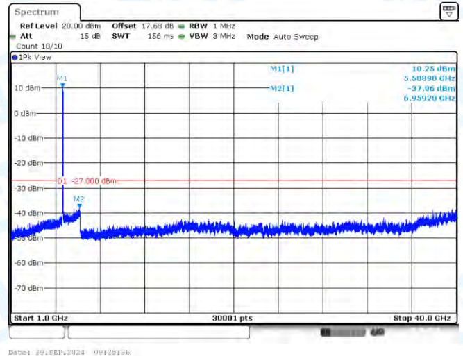
11N40-CDD-Ant3-5510-1000~40000-PASS
