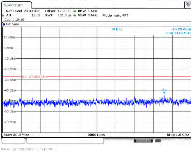
11AC20-CDD-Ant3-5720-30~1000-PASS
