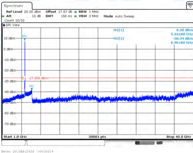
11N40-CDD-Ant2-5550-1000~40000-PASS
