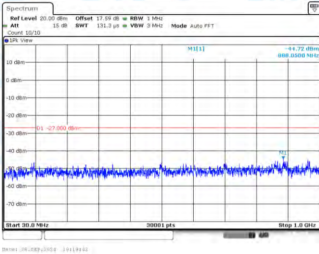
11AC40-CDD-Ant3-5310-30~1000-PASS
