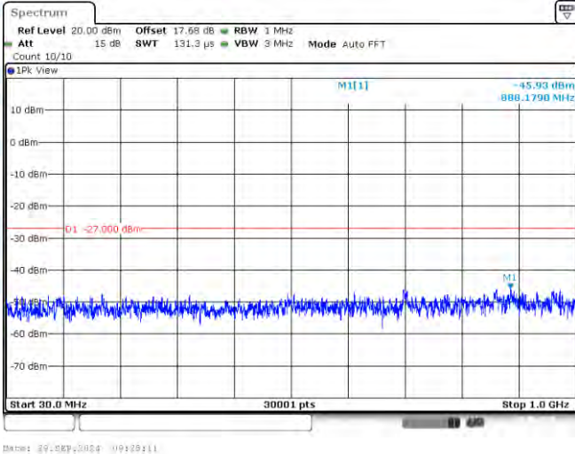
11N40-CDD-Ant3-5510-30~1000-PASS
