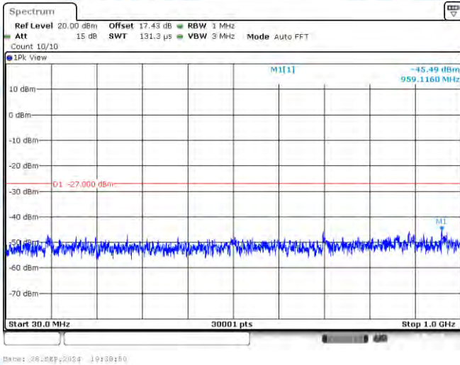
11AC80-CDD-Ant1-5290-30~1000-PASS
