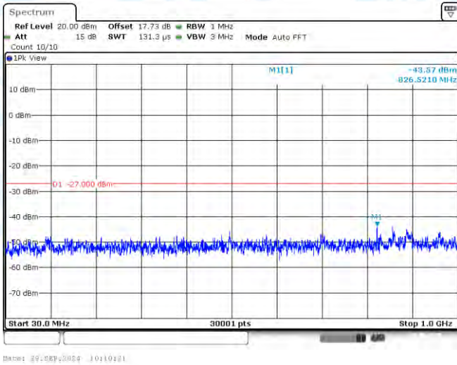
11AC40-CDD-Ant3-5550-30~1000-PASS
