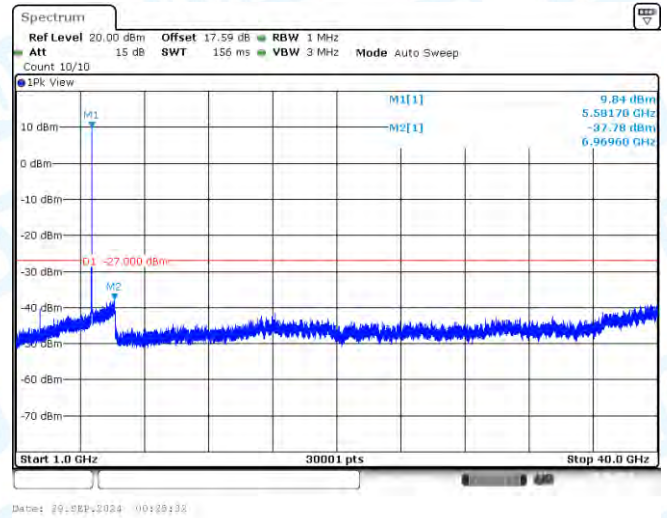
11AC20-CDD-Ant1-5580-1000~40000-PASS
