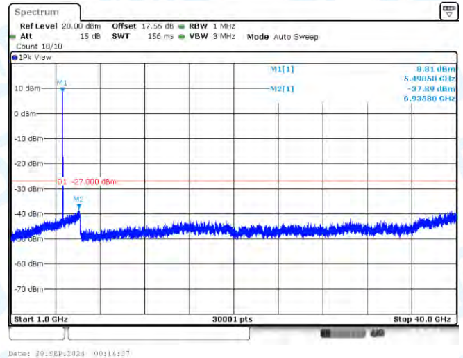
11AC20-CDD-Ant1-5500-1000~40000-PASS
