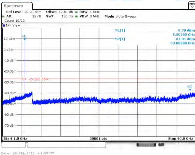
11AC40-CDD-Ant2-5510-1000~40000-PASS
