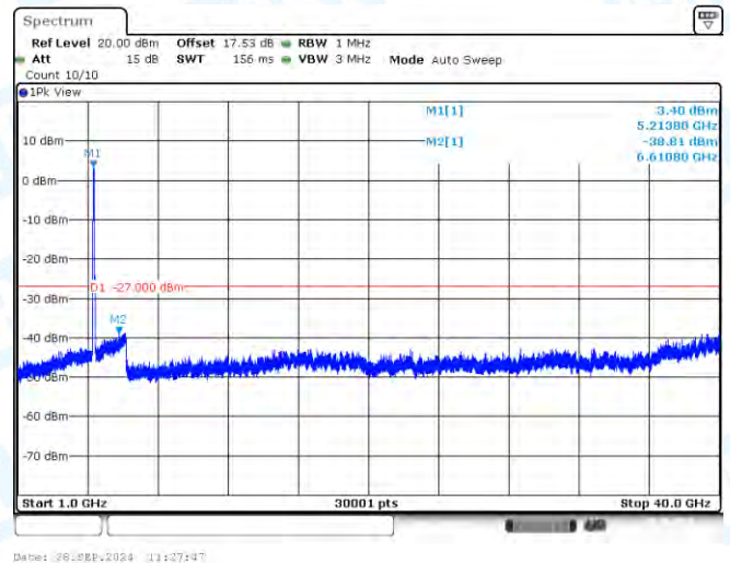
11AC80-CDD-Ant3-5210-1000~40000-PASS
