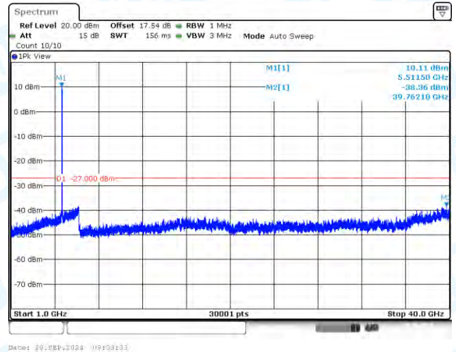
11AC40-CDD-Ant1-5510-1000~40000-PASS
