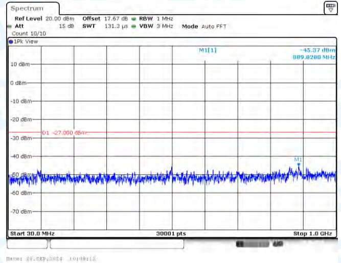
11AC40-CDD-Ant2-5550-30~1000-PASS
