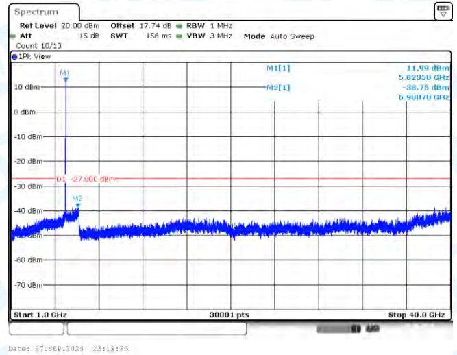
11AC20-CDD-Ant1-5825-1000~40000-PASS
