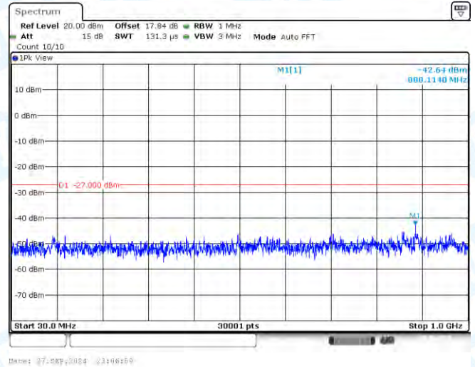
11AC20-CDD-Ant3-5785-30~1000-PASS
