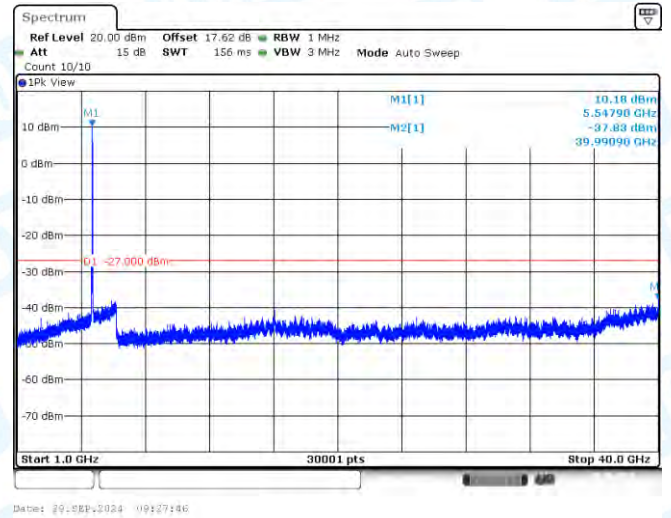
11N40-CDD-Ant1-5550-1000~40000-PASS
