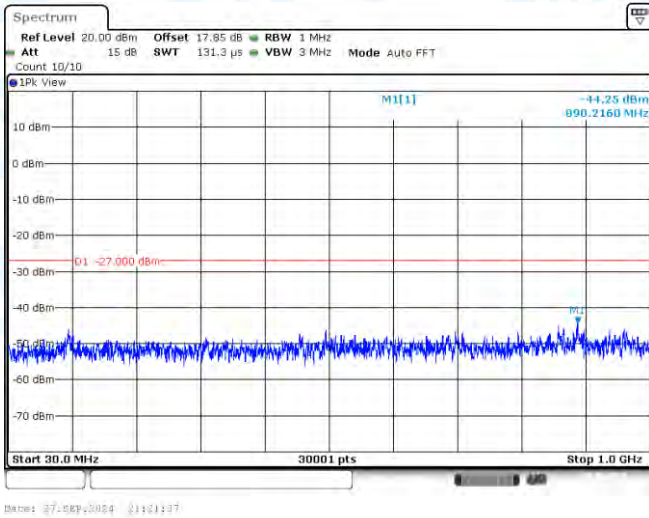
11N40-CDD-Ant3-5755-30~1000-PASS
