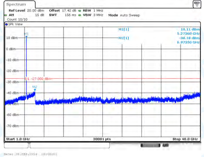
11N40-CDD-Ant1-5270-1000~40000-PASS
