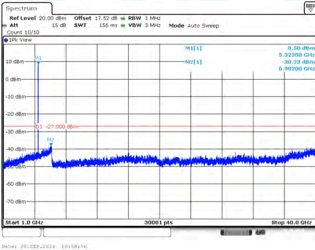
11AC20-CDD-Ant2-5320-1000~40000-PASS
