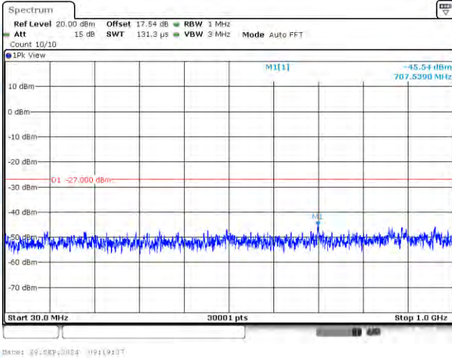
11N40-CDD-Ant1-5510-30~1000-PASS
