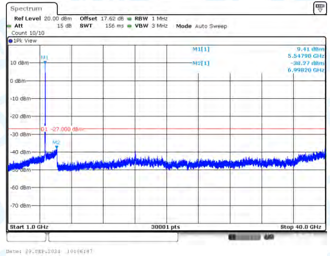
11AC40-CDD-Ant1-5550-1000~40000-PASS
