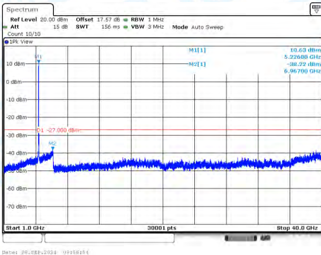
11N40-CDD-Ant2-5230-1000~40000-PASS
