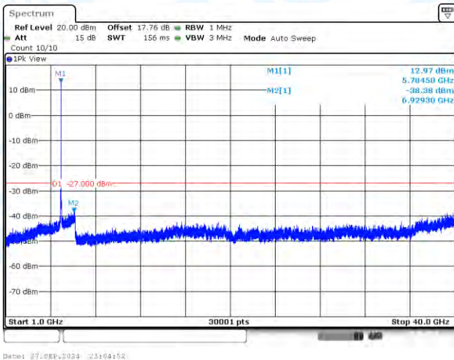
11AC20-CDD-Ant2-5785-1000~40000-PASS
