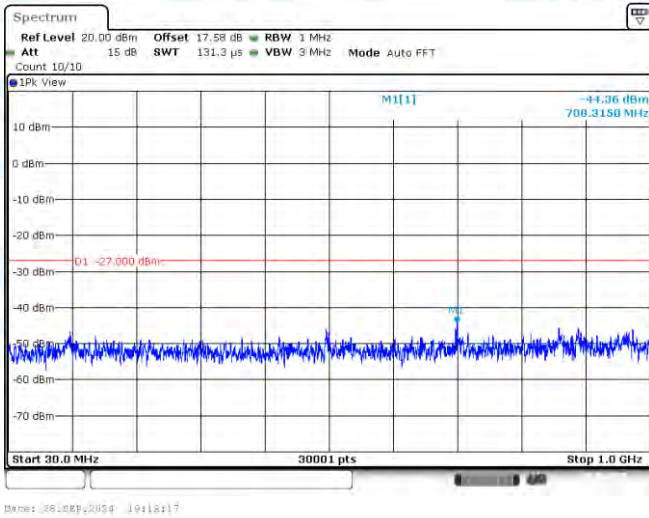
11AC40-CDD-Ant3-5270-30~1000-PASS
