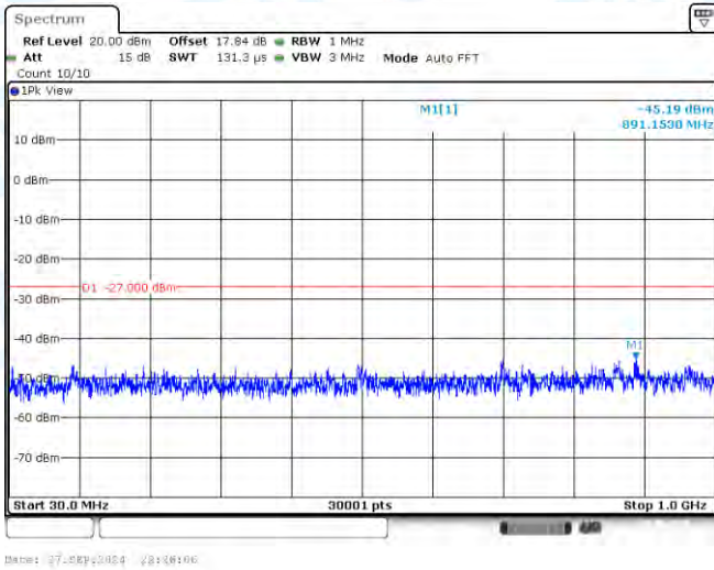
11AC40-CDD-Ant3-5795-30~1000-PASS
