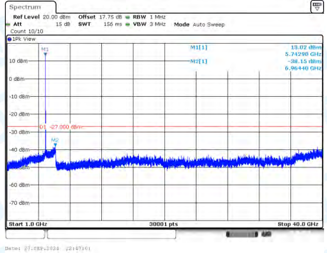
11AC20-CDD-Ant1-5745-1000~40000-PASS
