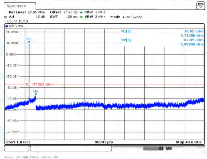
11N40-CDD-Ant3-5710-1000~40000-PASS
