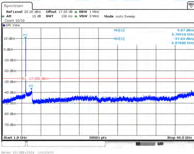
11AC40-CDD-Ant2-5710-1000~40000-PASS
