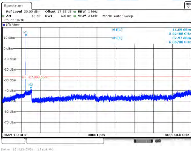
11AC20-CDD-Ant2-5825-1000~40000-PASS
