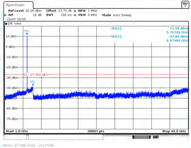
11AC40-CDD-Ant1-5755-1000~40000-PASS
