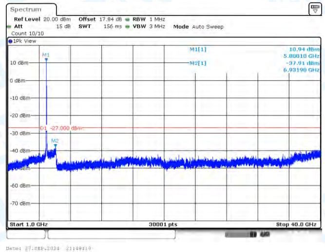
11N40-CDD-Ant3-5795-1000~40000-PASS
