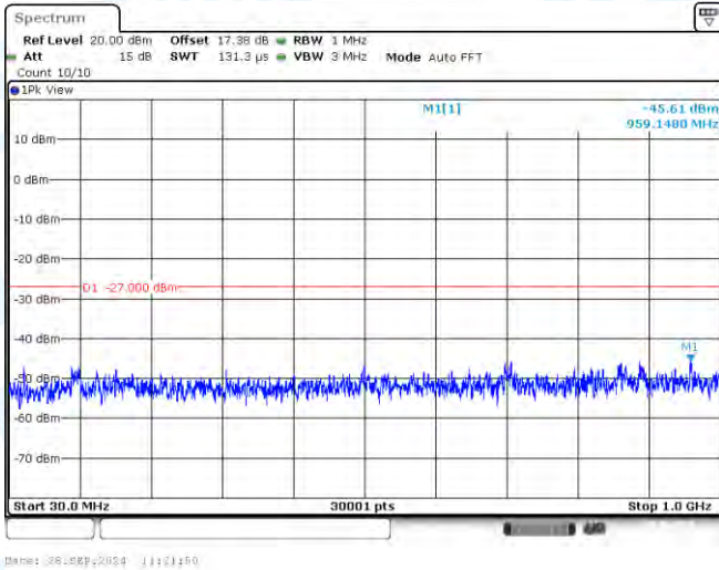
11AC80-CDD-Ant1-5210-30~1000-PASS
