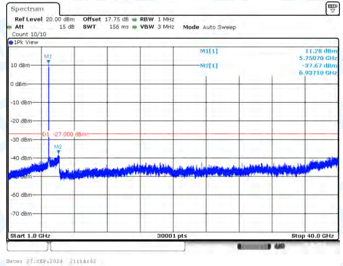
11N40-CDD-Ant1-5755-1000~40000-PASS
