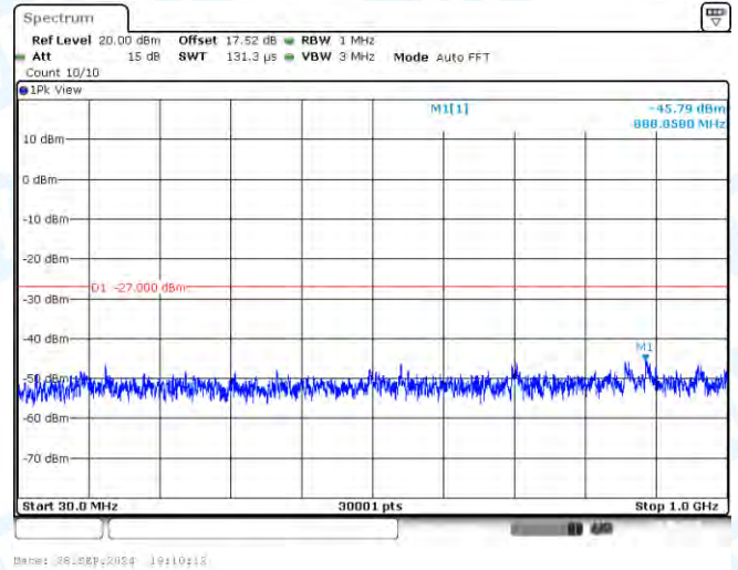
11AC40-CDD-Ant2-5270-30~1000-PASS
