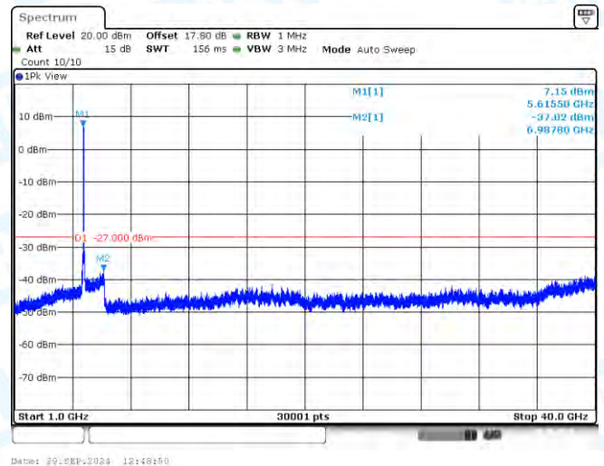
11AC80-CDD-Ant3-5610-1000~40000-PASS
