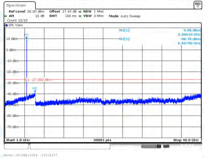
11AC40-CDD-Ant1-5310-1000~40000-PASS
