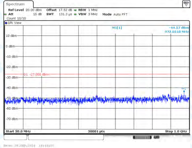
11AC20-CDD-Ant2-5280-30~1000-PASS
