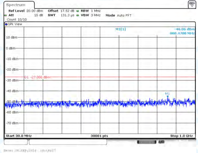
11N40-CDD-Ant2-5310-30~1000-PASS
