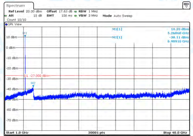
11AC20-CDD-Ant1-5260-1000~40000-PASS
