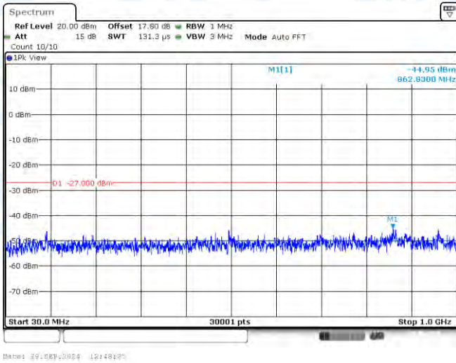
11AC80-CDD-Ant3-5610-30~1000-PASS
