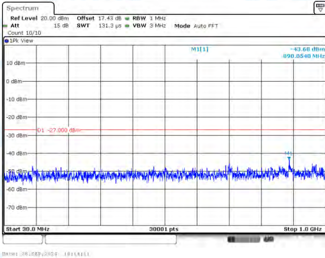
11N40-CDD-Ant1-5310-30~1000-PASS
