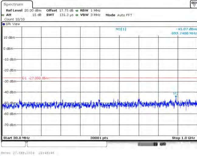
11AC20-CDD-Ant1-5745-30~1000-PASS
