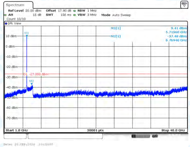
11AC40-CDD-Ant1-5710-1000~40000-PASS
