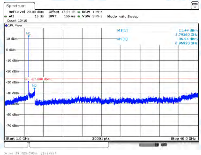
11AC40-CDD-Ant3-5795-1000~40000-PASS
