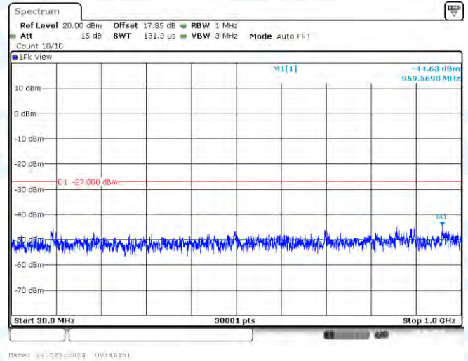
11N40-CDD-Ant2-5710-30~1000-PASS
