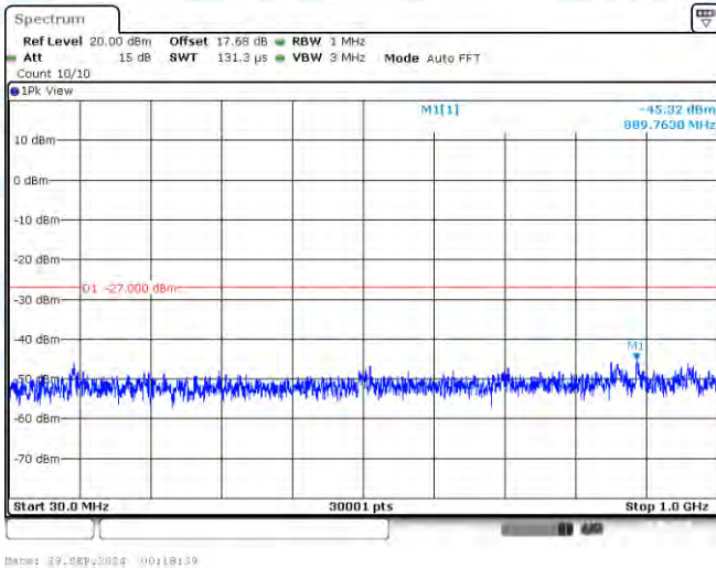
11AC20-CDD-Ant3-5500-30~1000-PASS
