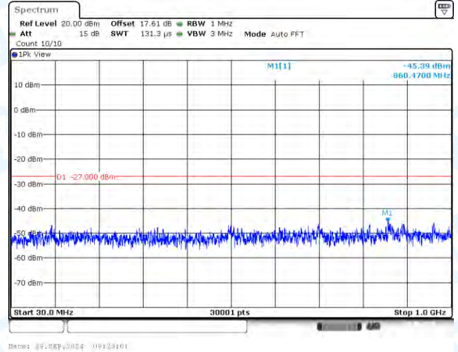
11N40-CDD-Ant2-5510-30~1000-PASS
