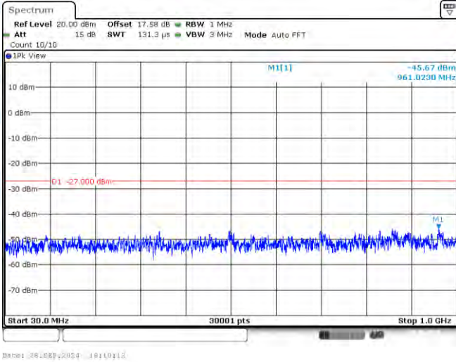
11N40-CDD-Ant3-5270-30~1000-PASS
