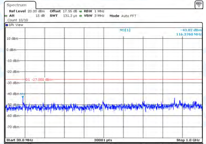
11AC20-CDD-Ant2-5260-30~1000-PASS
