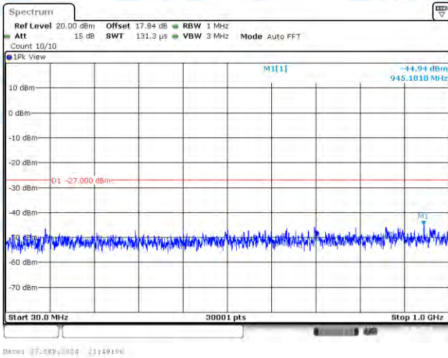
11N40-CDD-Ant3-5795-30~1000-PASS
