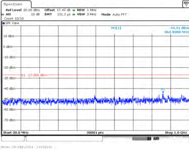
11AC20-CDD-Ant1-5320-30~1000-PASS
