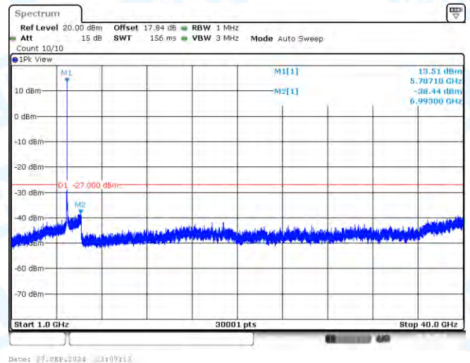
11AC20-CDD-Ant3-5785-1000~40000-PASS
