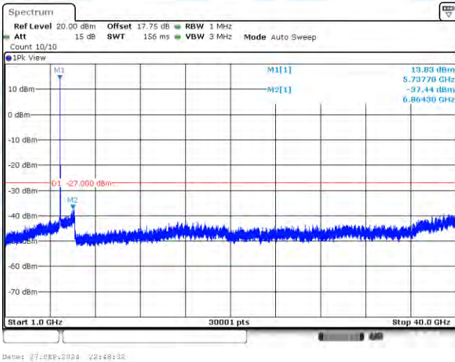
11AC20-CDD-Ant2-5745-1000~40000-PASS
