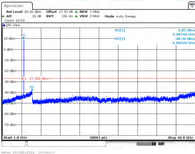
11AC40-CDD-Ant2-5310-1000~40000-PASS
