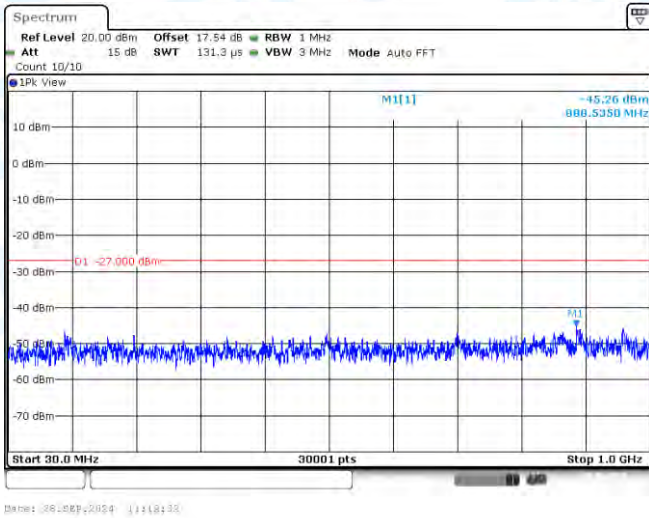
11AC40-CDD-Ant3-5190-30~1000-PASS
