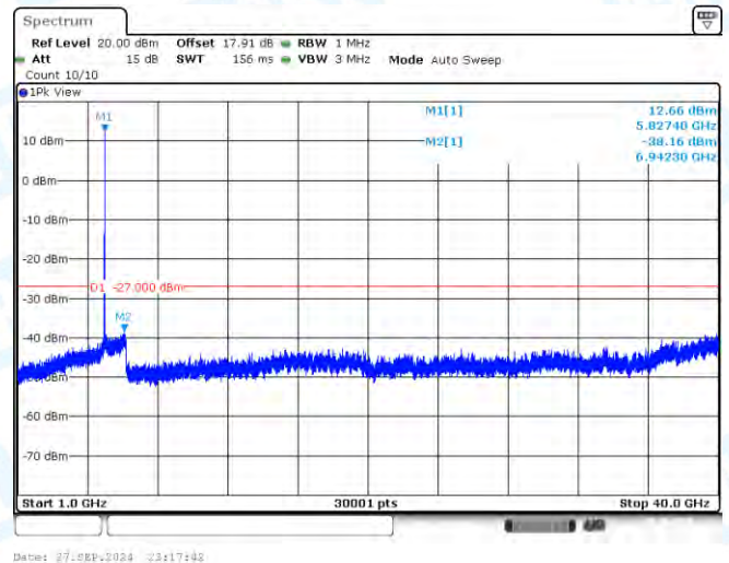
11AC20-CDD-Ant3-5825-1000~40000-PASS
