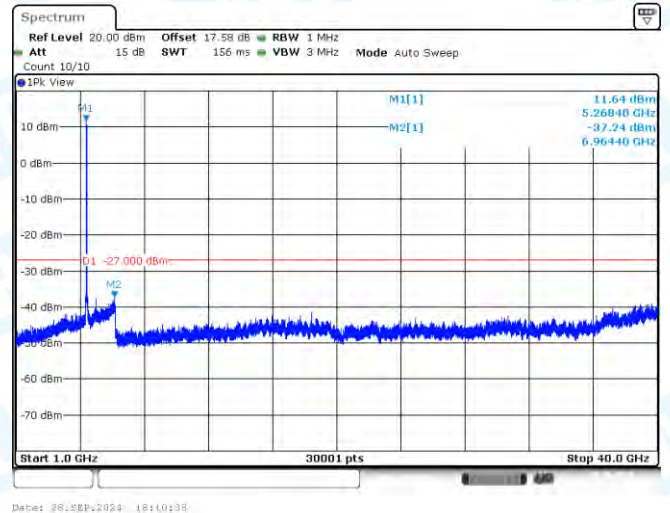
11N40-CDD-Ant3-5270-1000~40000-PASS
