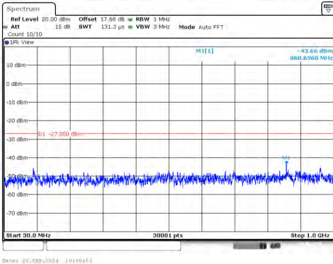
11AC40-CDD-Ant3-5510-30~1000-PASS
