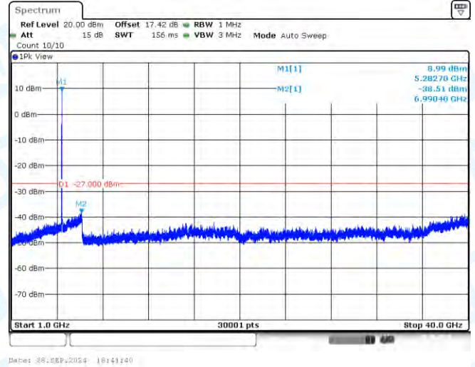
11AC20-CDD-Ant1-5280-1000~40000-PASS
