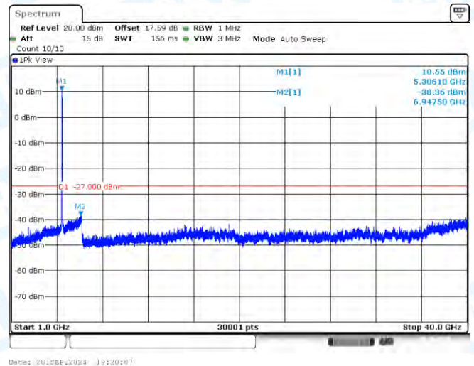
11AC40-CDD-Ant3-5310-1000~40000-PASS
