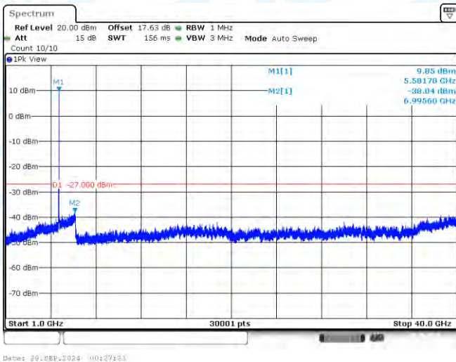
11AC20-CDD-Ant2-5580-1000~40000-PASS
