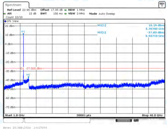
11AC40-CDD-Ant3-5710-1000~40000-PASS
