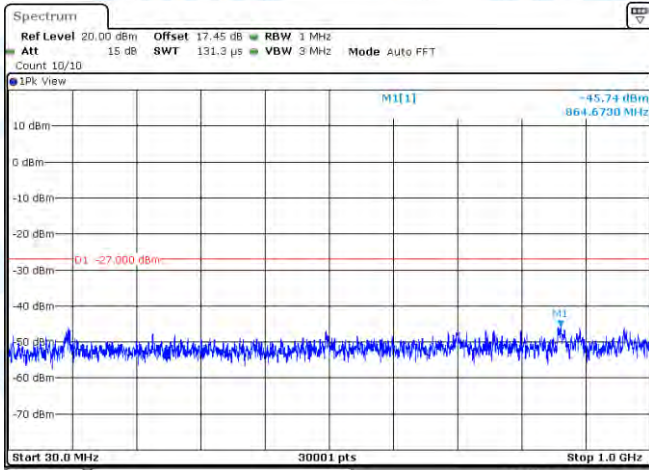
11AC20-CDD-Ant1-5180-30~1000-PASS
