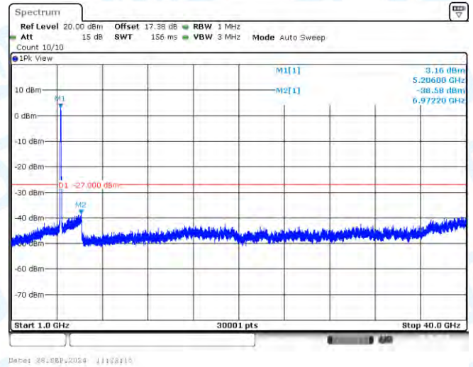
11AC80-CDD-Ant1-5210-1000~40000-PASS
