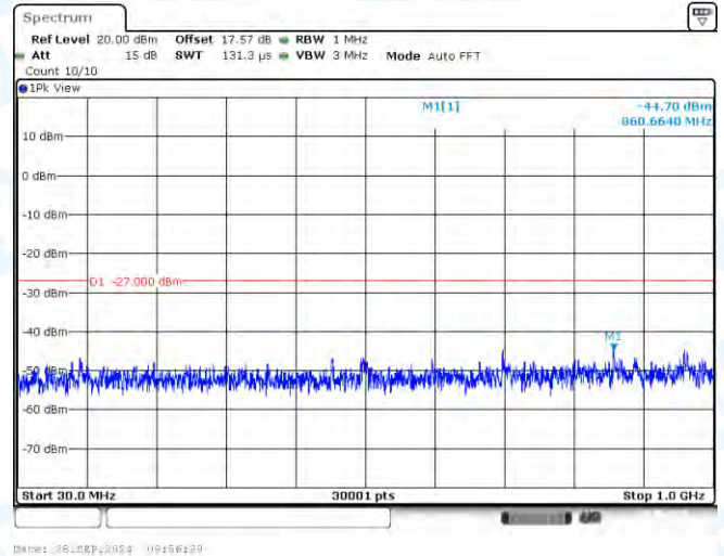
11N40-CDD-Ant2-5230-30~1000-PASS
