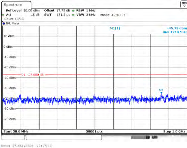
11AC40-CDD-Ant1-5755-30~1000-PASS
