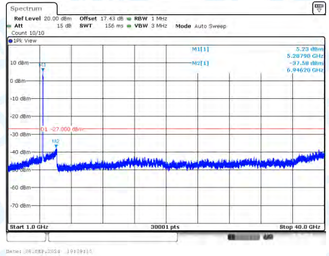
11AC80-CDD-Ant1-5290-1000~40000-PASS
