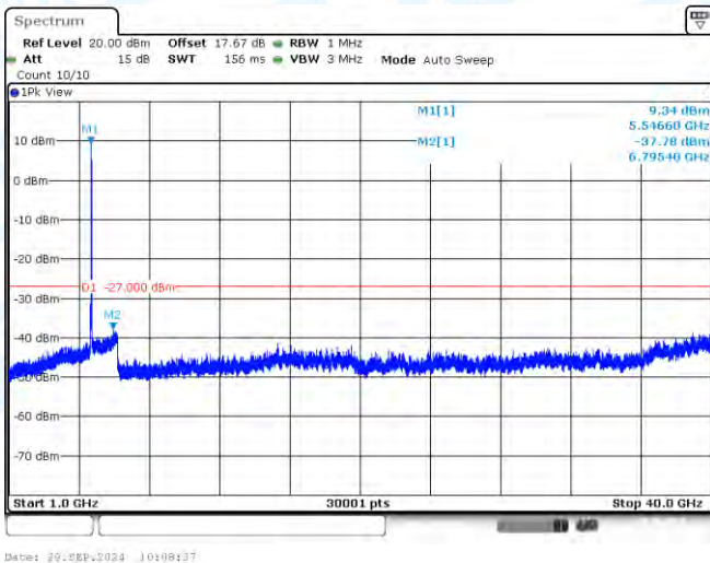
11AC40-CDD-Ant2-5550-1000~40000-PASS
