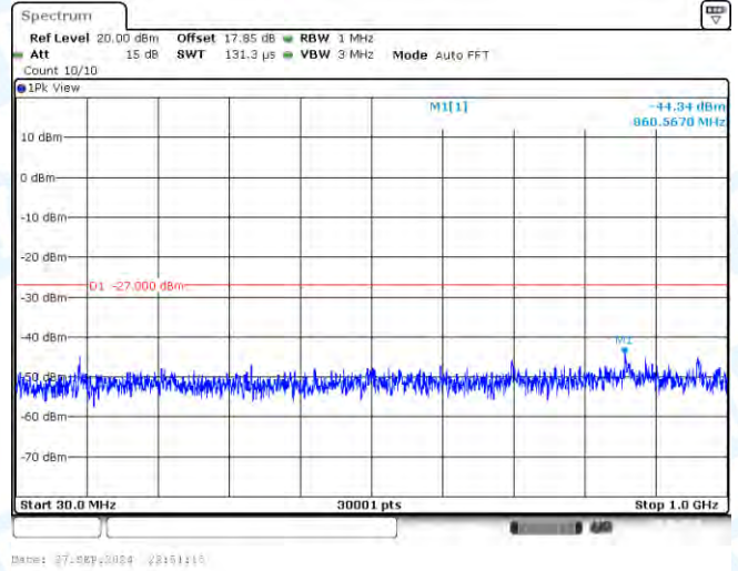
11AC20-CDD-Ant3-5745-30~1000-PASS
