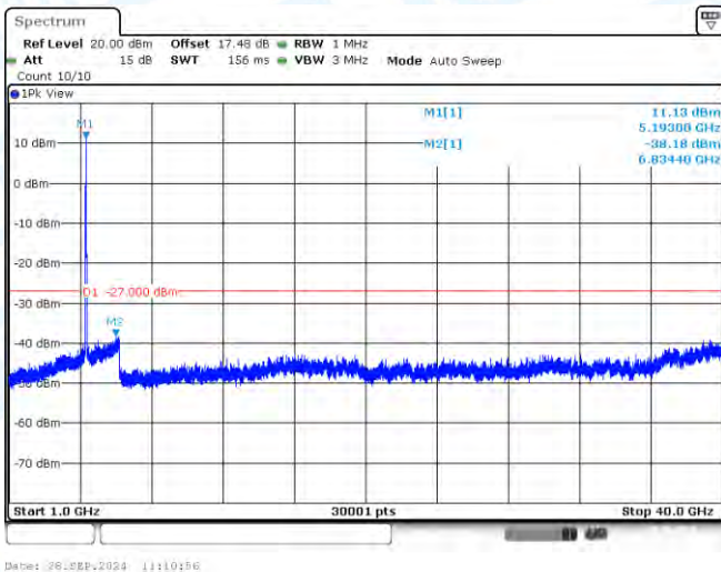
11AC40-CDD-Ant2-5190-1000~40000-PASS
