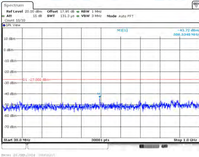
11N40-CDD-Ant3-5710-30~1000-PASS
