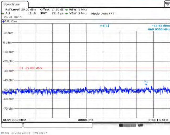
11AC20-CDD-Ant1-5720-30~1000-PASS
