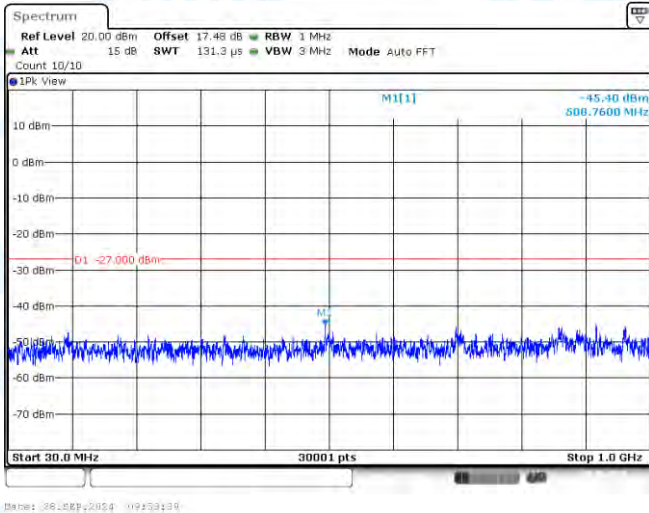
11N40-CDD-Ant1-5230-30~1000-PASS
