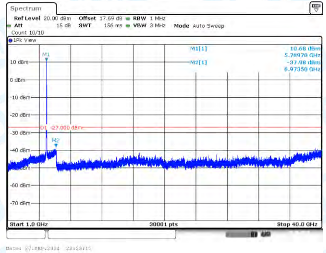
11AC40-CDD-Ant1-5795-1000~40000-PASS
