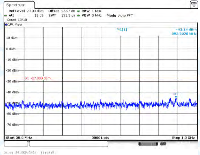
11AC40-CDD-Ant2-5230-30~1000-PASS
