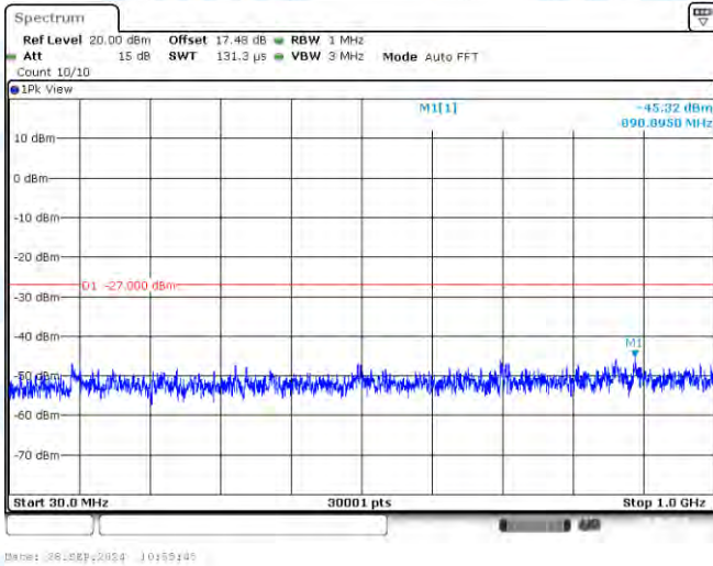
11AC20-CDD-Ant1-5240-30~1000-PASS
