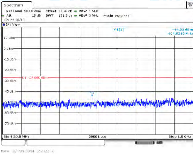
11AC20-CDD-Ant2-5785-30~1000-PASS
