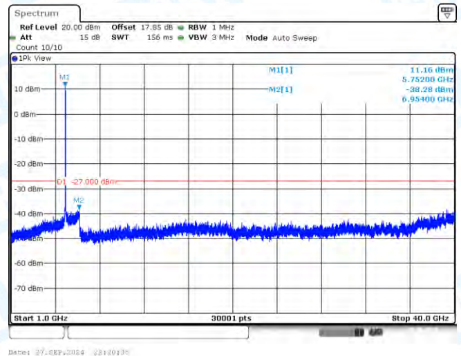
11AC40-CDD-Ant3-5755-1000~40000-PASS
