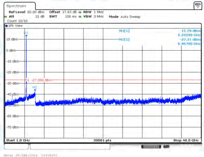
11N40-CDD-Ant3-5230-1000~40000-PASS
