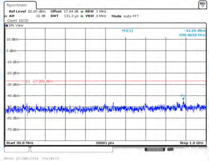
11AC20-CDD-Ant2-5500-30~1000-PASS
