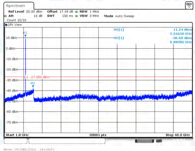
11N40-CDD-Ant3-5310-1000~40000-PASS
