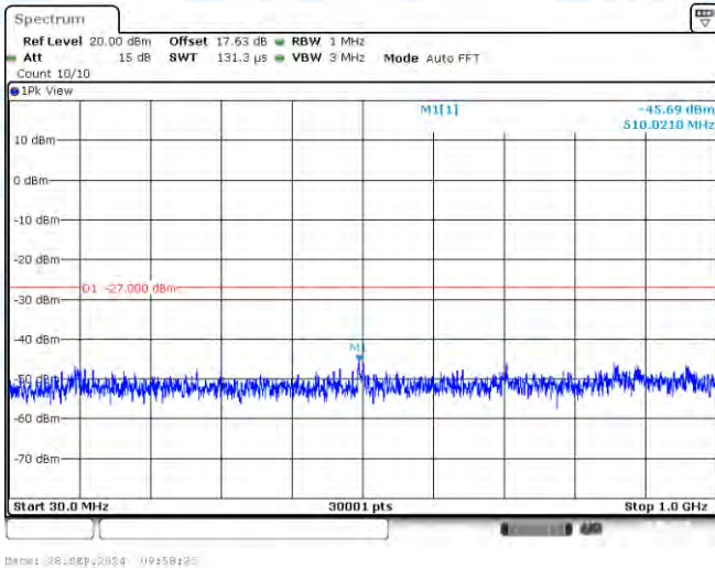
11N40-CDD-Ant3-5230-30~1000-PASS
