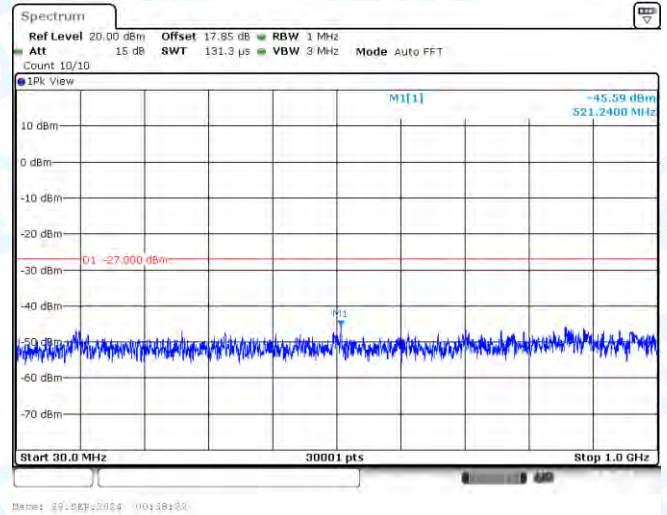
11AC20-CDD-Ant2-5720-30~1000-PASS
