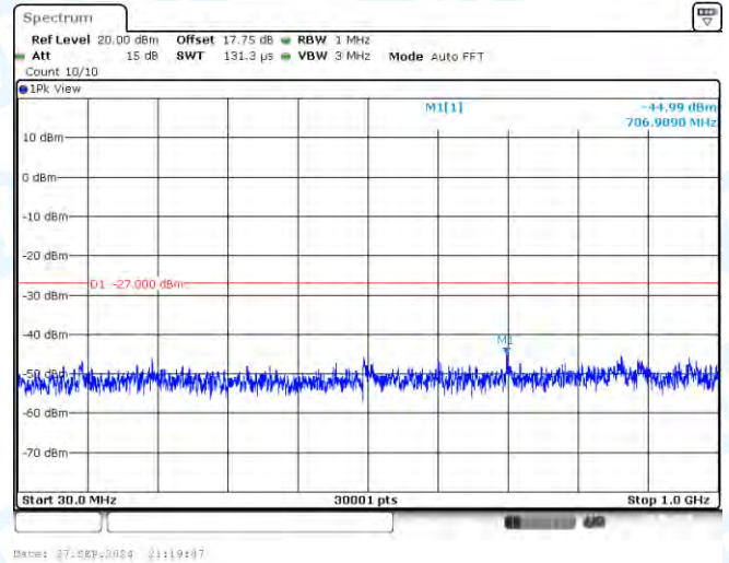
11N40-CDD-Ant2-5755-30~1000-PASS
