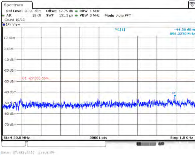
11N40-CDD-Ant1-5755-30~1000-PASS
