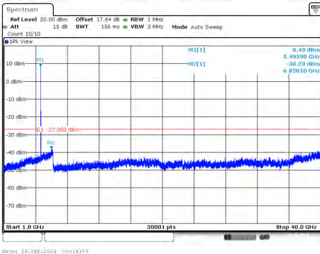
11AC20-CDD-Ant2-5500-1000~40000-PASS
