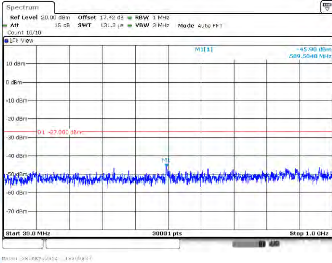
11N40-CDD-Ant1-5270-30~1000-PASS
