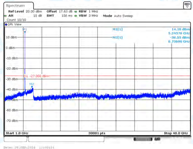
11AC20-CDD-Ant3-5240-1000~40000-PASS
