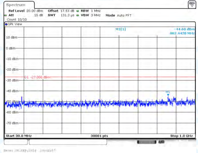
11AC80-CDD-Ant2-5290-30~1000-PASS
