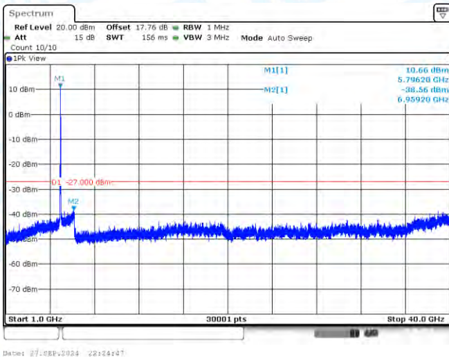
11AC40-CDD-Ant2-5795-1000~40000-PASS
