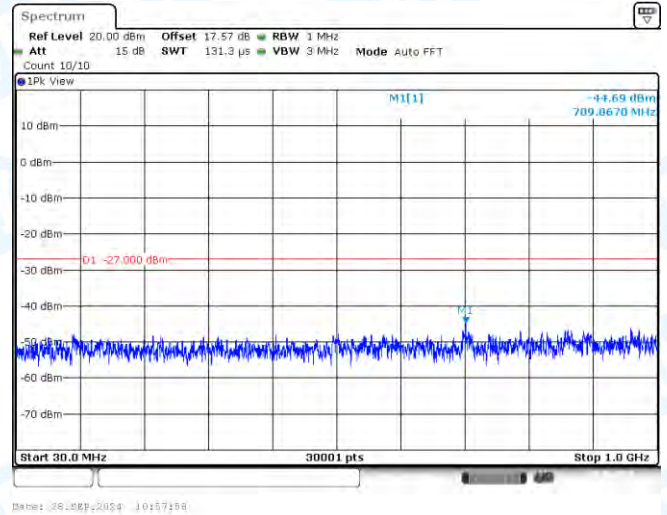
11AC20-CDD-Ant2-5240-30~1000-PASS
