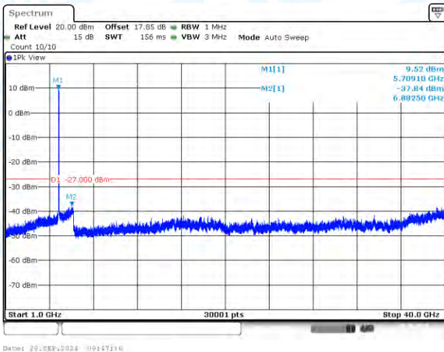
11N40-CDD-Ant2-5710-1000~40000-PASS
