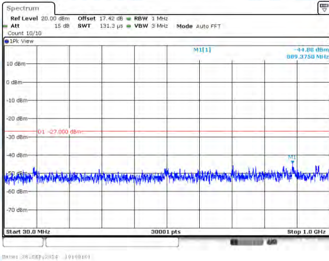
11AC40-CDD-Ant1-5270-30~1000-PASS
