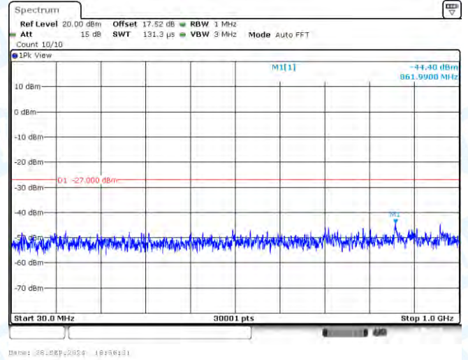
11AC20-CDD-Ant2-5320-30~1000-PASS
