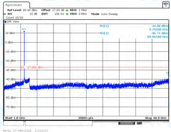
11N40-CDD-Ant3-5755-1000~40000-PASS
