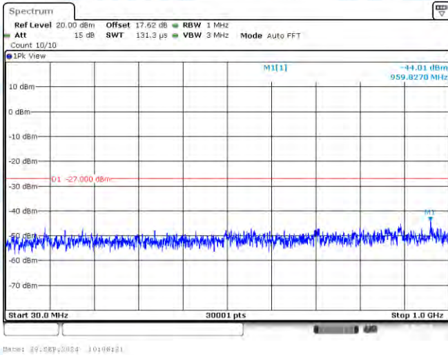
11AC40-CDD-Ant1-5550-30~1000-PASS
