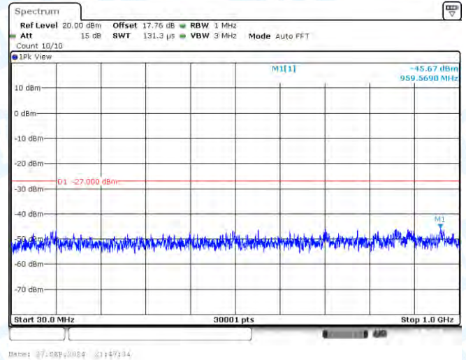
11N40-CDD-Ant2-5795-30~1000-PASS
