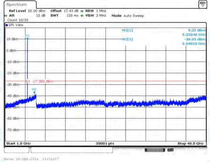
11AC20-CDD-Ant1-5320-1000~40000-PASS
