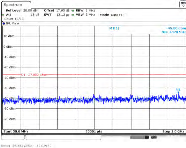
11AC40-CDD-Ant1-5710-30~1000-PASS
