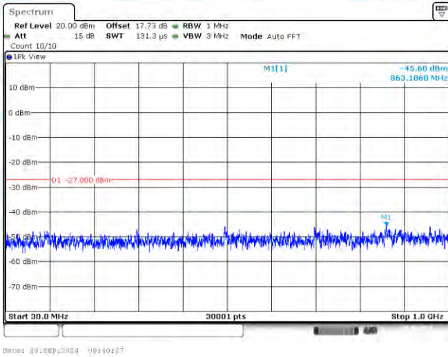
11N40-CDD-Ant3-5550-30~1000-PASS
