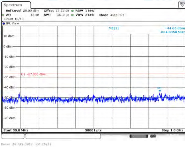
11AC20-CDD-Ant3-5580-30~1000-PASS
