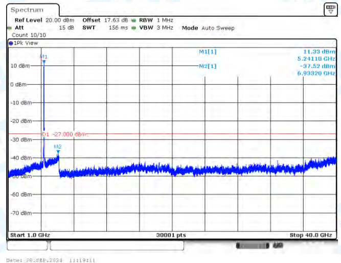
11AC40-CDD-Ant3-5230-1000~40000-PASS
