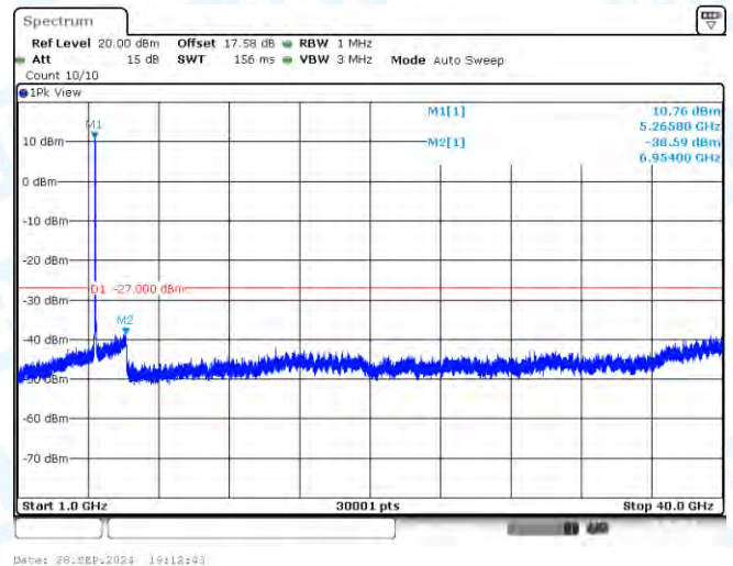
11AC40-CDD-Ant3-5270-1000~40000-PASS
