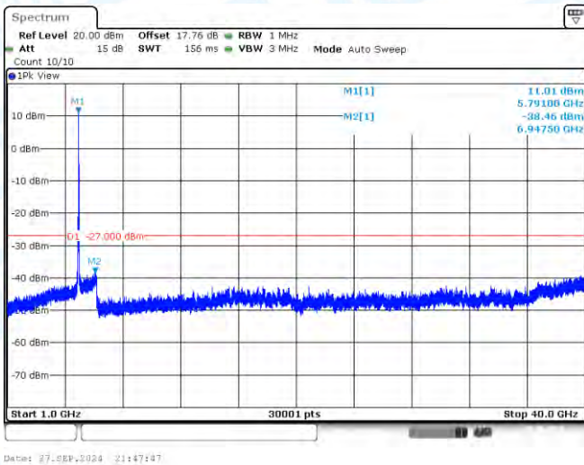
11N40-CDD-Ant2-5795-1000~40000-PASS
