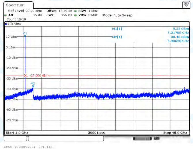
11AC20-CDD-Ant3-5320-1000~40000-PASS
