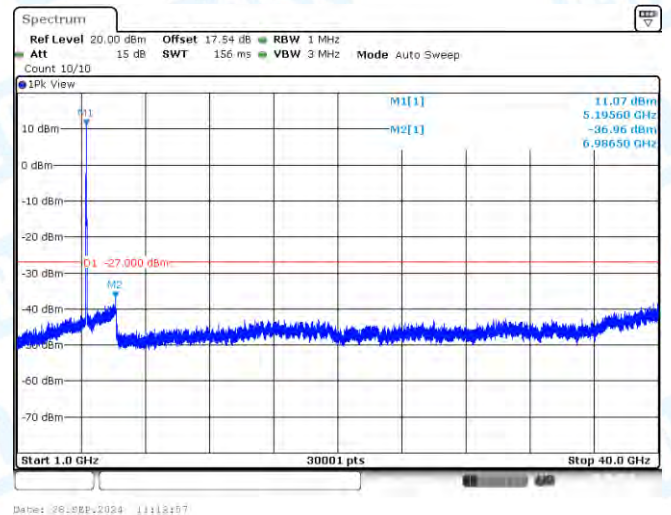
11AC40-CDD-Ant3-5190-1000~40000-PASS
