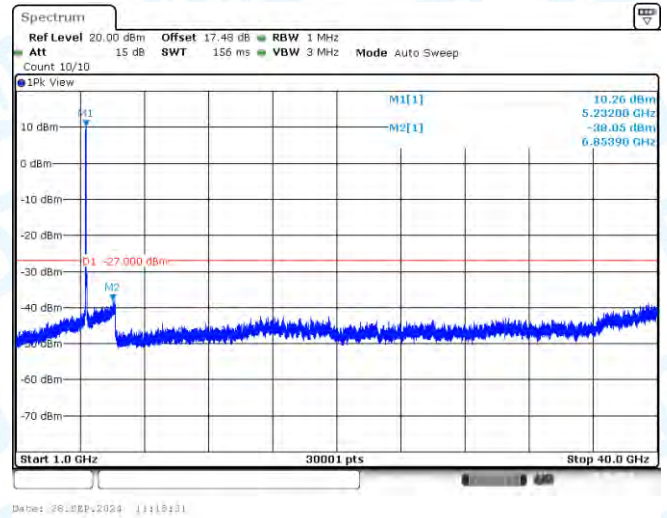
11AC40-CDD-Ant1-5230-1000~40000-PASS
