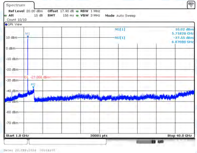
11AC20-CDD-Ant1-5720-1000~40000-PASS
