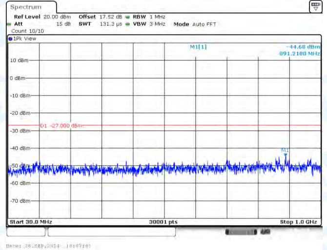
11N40-CDD-Ant2-5270-30~1000-PASS
