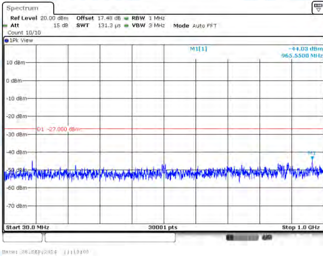
11AC40-CDD-Ant1-5230-30~1000-PASS
