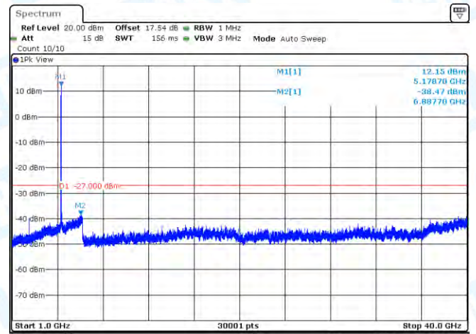
11AC20-CDD-Ant1-5180-1000~40000-PASS
