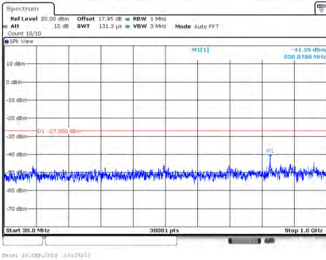
11AC40-CDD-Ant3-5710-30~1000-PASS
