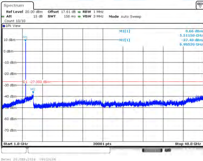
11N40-CDD-Ant2-5510-1000~40000-PASS
