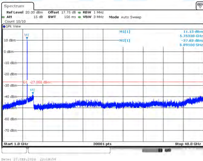
11AC40-CDD-Ant2-5755-1000~40000-PASS
