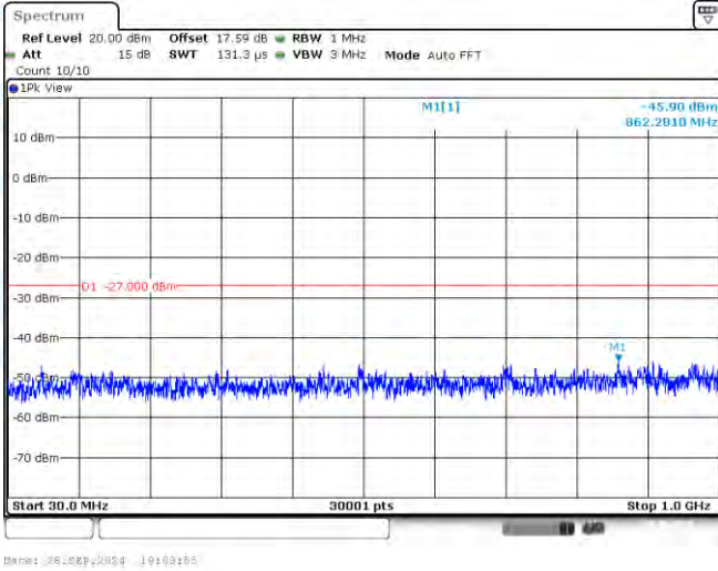
11AC20-CDD-Ant3-5320-30~1000-PASS
