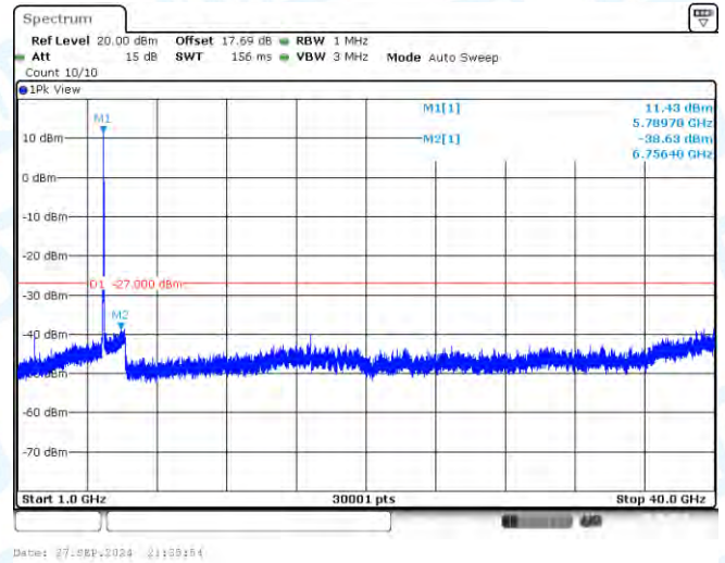
11N40-CDD-Ant1-5795-1000~40000-PASS
