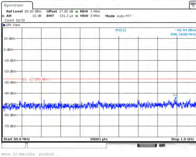
11AC40-CDD-Ant3-5755-30~1000-PASS
