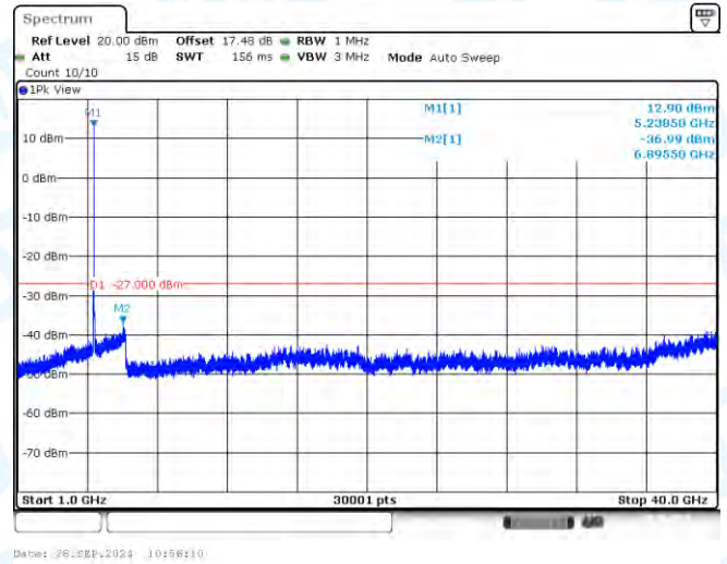
11AC20-CDD-Ant1-5240-1000~40000-PASS
