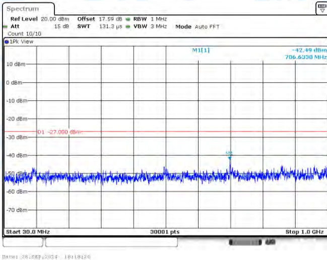
11N40-CDD-Ant3-5310-30~1000-PASS
