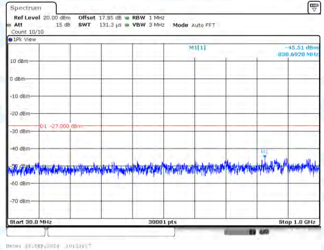
11AC40-CDD-Ant2-5710-30~1000-PASS
