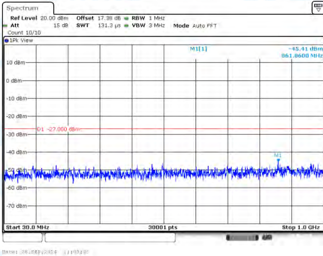
11AC40-CDD-Ant1-5190-30~1000-PASS
