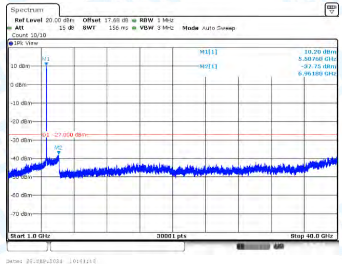
11AC40-CDD-Ant3-5510-1000~40000-PASS
