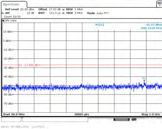
11AC80-CDD-Ant3-5210-30~1000-PASS
