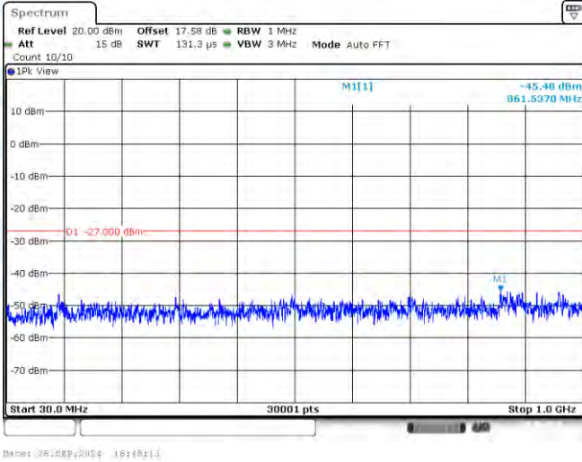
11AC20-CDD-Ant3-5280-30~1000-PASS
