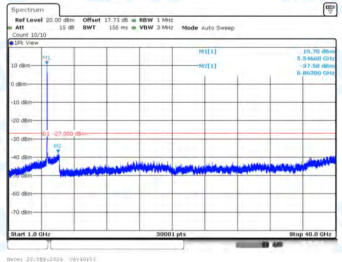
11N40-CDD-Ant3-5550-1000~40000-PASS
