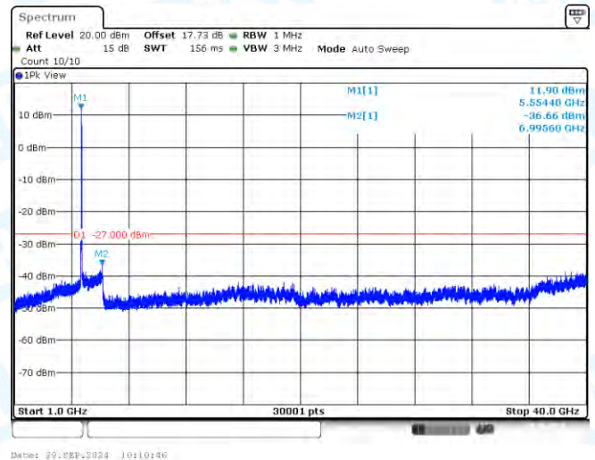
11AC40-CDD-Ant3-5550-1000~40000-PASS
