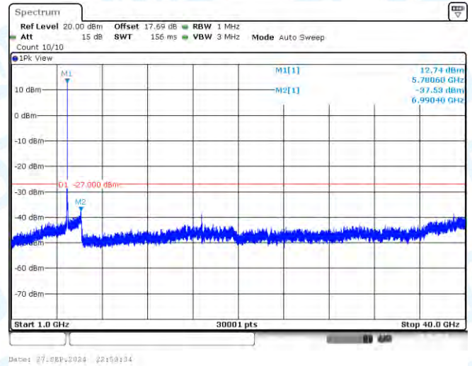
11AC20-CDD-Ant1-5785-1000~40000-PASS
