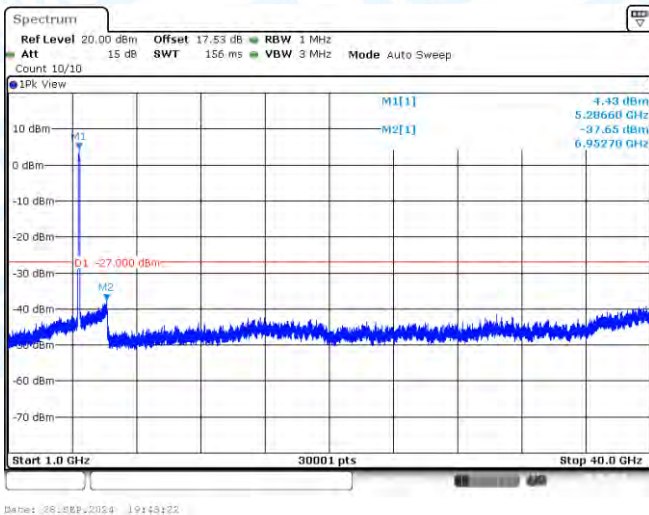
11AC80-CDD-Ant2-5290-1000~40000-PASS
