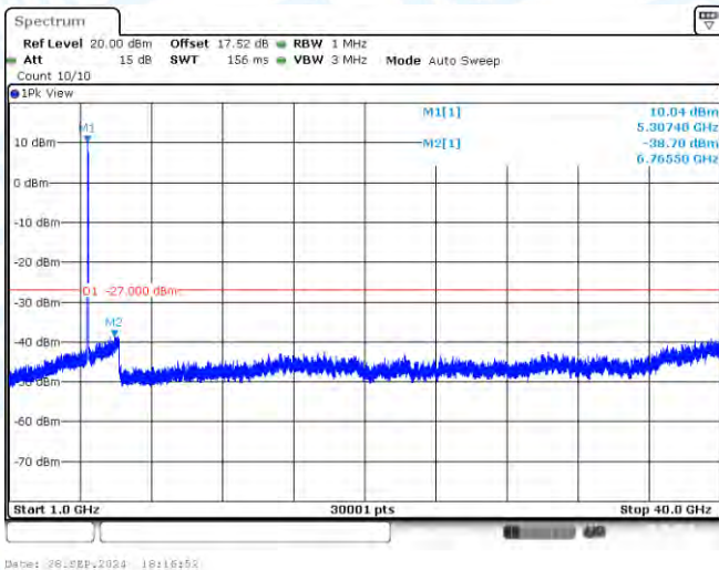
11N40-CDD-Ant2-5310-1000~40000-PASS
