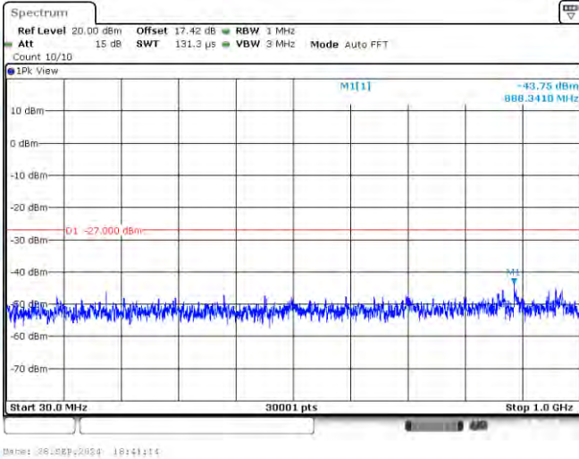
11AC20-CDD-Ant1-5280-30~1000-PASS
