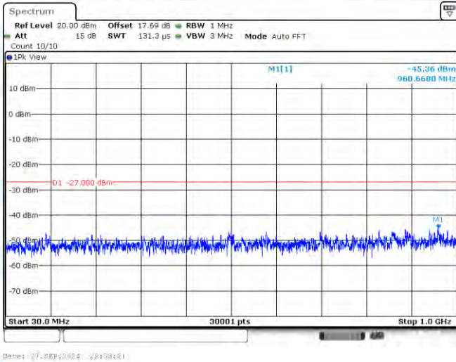
11AC20-CDD-Ant1-5785-30~1000-PASS
