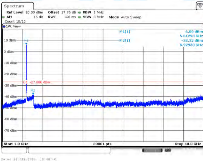
11AC80-CDD-Ant2-5610-1000~40000-PASS
