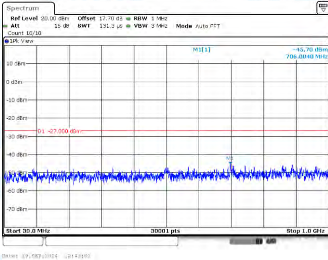
11AC80-CDD-Ant1-5610-30~1000-PASS
