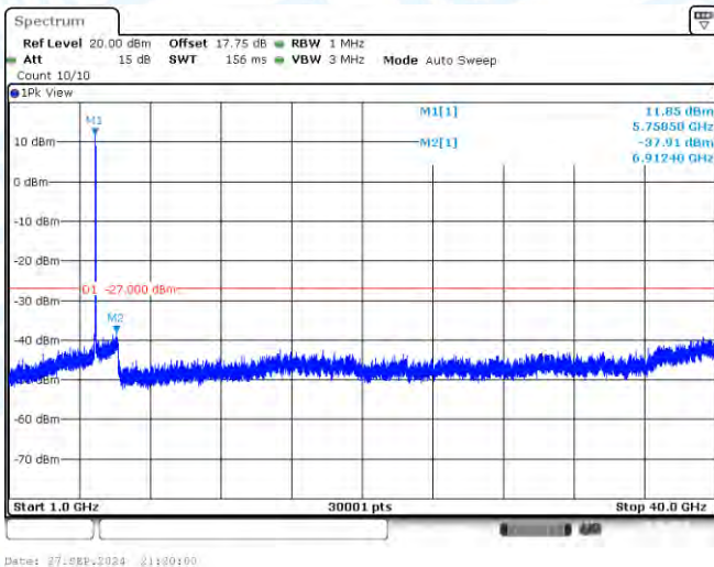
11N40-CDD-Ant2-5755-1000~40000-PASS
