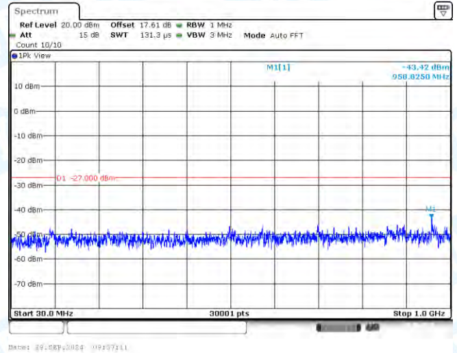
11AC40-CDD-Ant2-5510-30~1000-PASS
