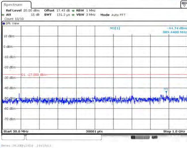
11AC40-CDD-Ant1-5310-30~1000-PASS
