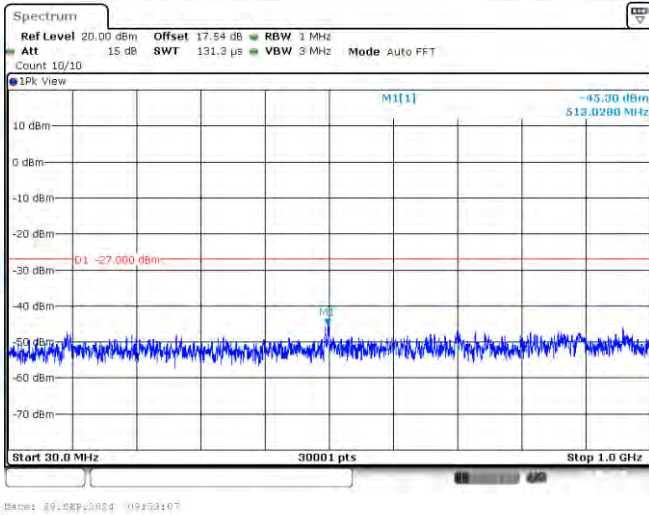
11AC40-CDD-Ant1-5510-30~1000-PASS
