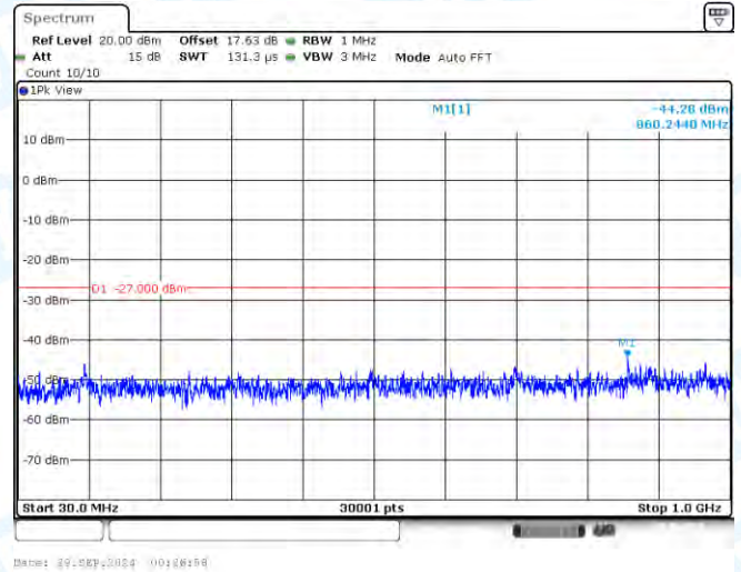
11AC20-CDD-Ant2-5580-30~1000-PASS
