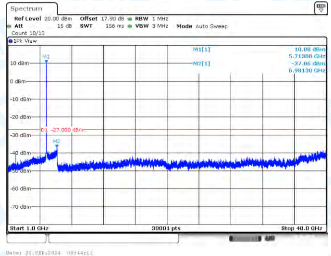
11N40-CDD-Ant1-5710-1000~40000-PASS
