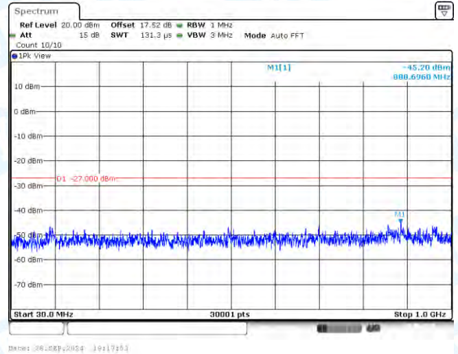
11AC40-CDD-Ant2-5310-30~1000-PASS
