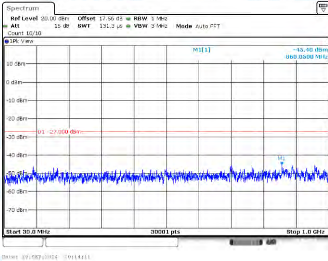
11AC20-CDD-Ant1-5500-30~1000-PASS
