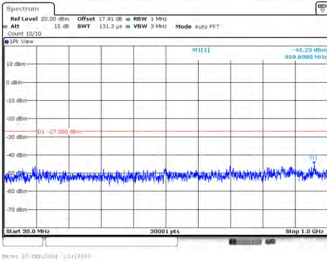
11AC20-CDD-Ant3-5825-30~1000-PASS
