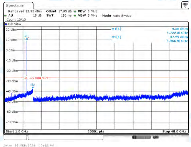
11AC20-CDD-Ant3-5720-1000~40000-PASS
