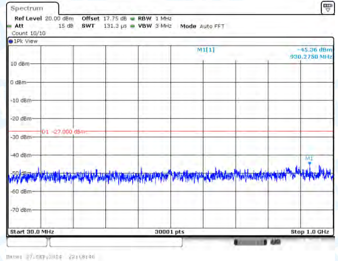
11AC40-CDD-Ant2-5755-30~1000-PASS
