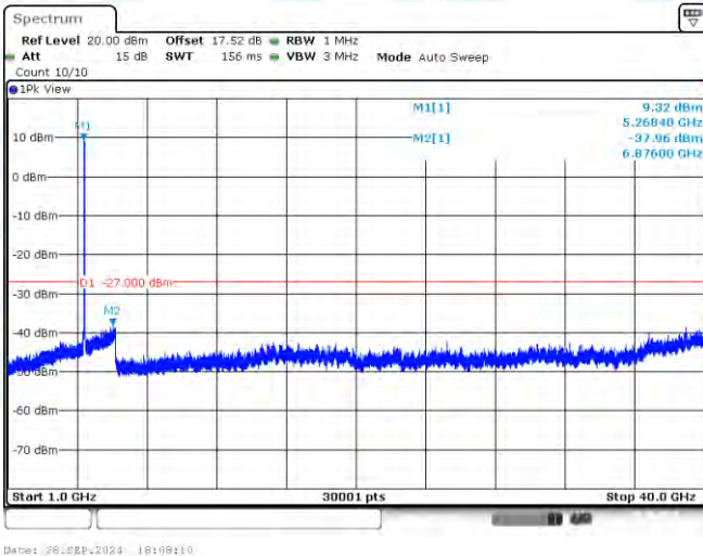
11N40-CDD-Ant2-5270-1000~40000-PASS
