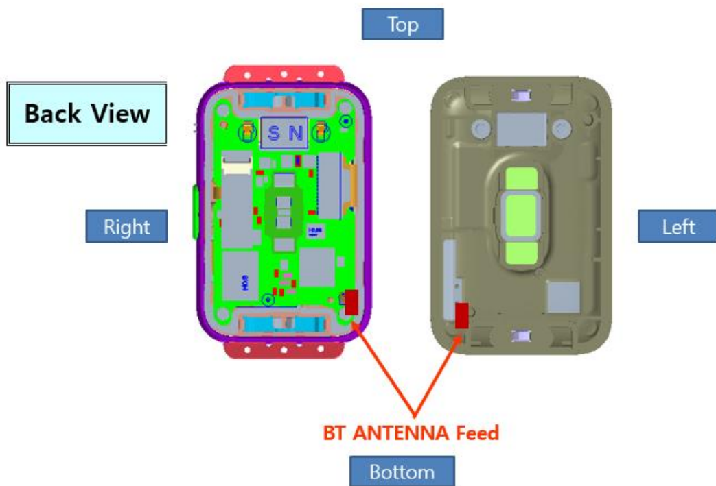
Picture 3 Antenna Locations
