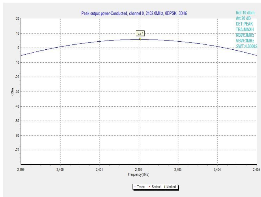
Fig. 7 Maximum Peak Output Power(8DPSK, Ch 0)
