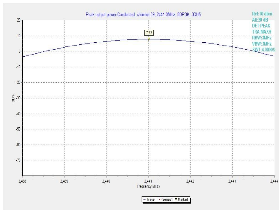
Fig. 8 Maximum Peak Output Power(8DPSK, Ch 39)
