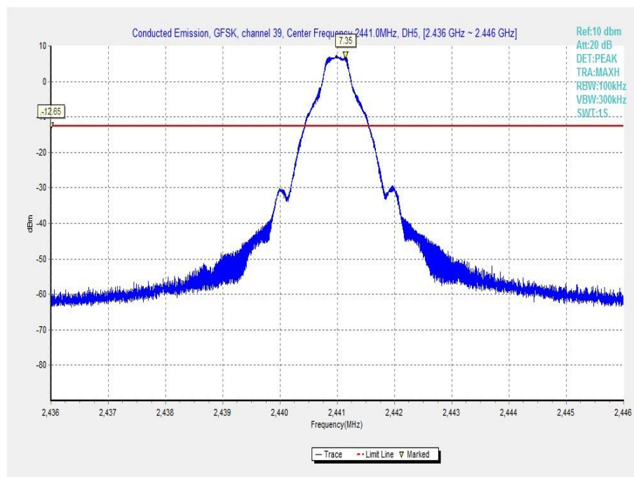
Fig. 26 Conducted Spurious Emission (GFSK, Ch39, 2.441GHz)
