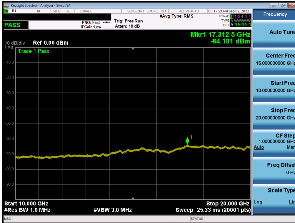
Plot 7-117. Conducted Spurious Plot (WCDMA Ch. 9262 - ANT A)
