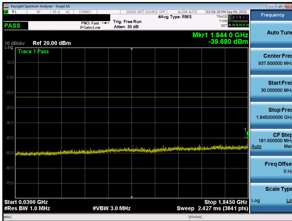
Plot 7-106. Conducted Spurious Plot (GPRS Ch. 512 - ANT A)
