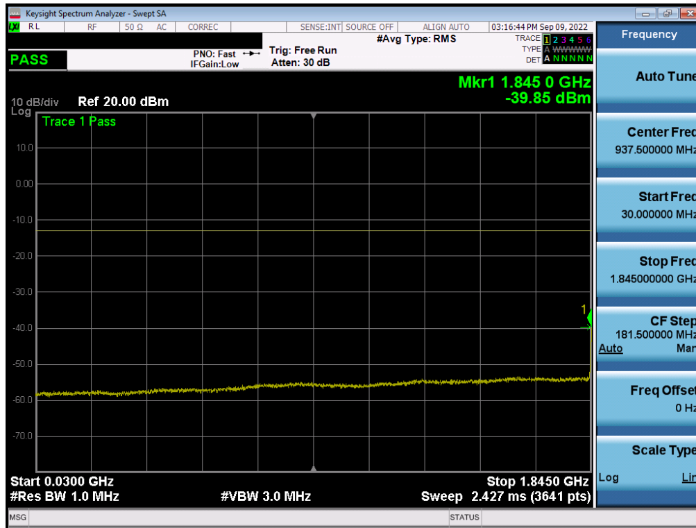
Plot 7-115. Conducted Spurious Plot (WCDMA Ch. 9262 - ANT A)
