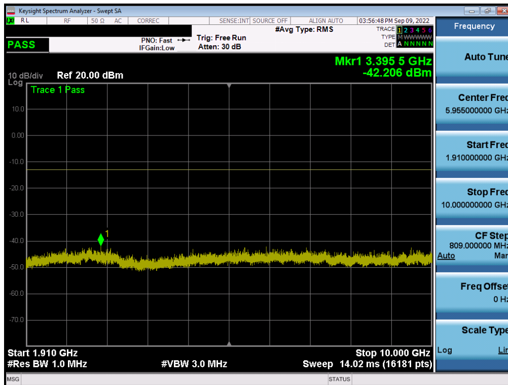
Plot 7-107. Conducted Spurious Plot (GPRS Ch. 512 - ANT A)
