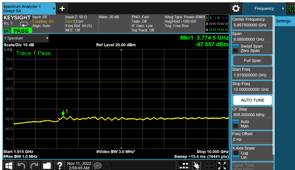
Plot 7-98. Conducted Spurious Plot (NR Band n25/2 - 40.0MHz - 1RB - Low Channel - ANT F)
