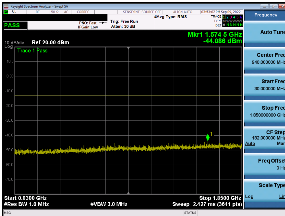
Plot 7-109. Conducted Spurious Plot (GPRS Ch. 661 - ANT A)
