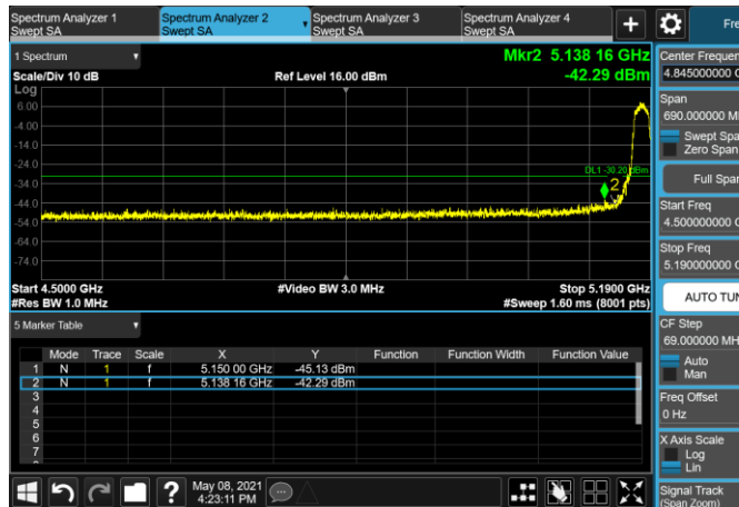
5180MHz with CDD PK
