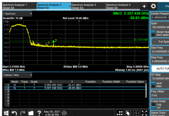
5320MHz with CDD PK
