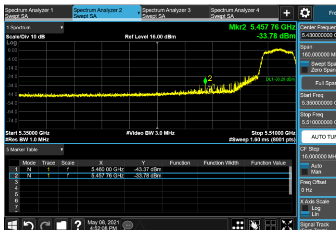
5500MHz with CDD PK
