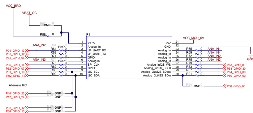
BOOSTER PACK INTERFACE
