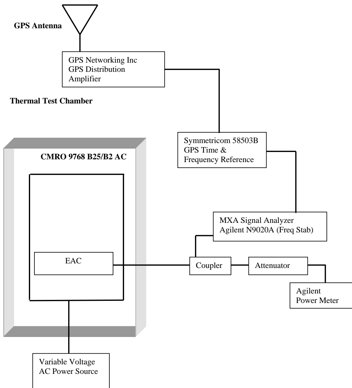
FIGURE 1: TEST SET-UP
