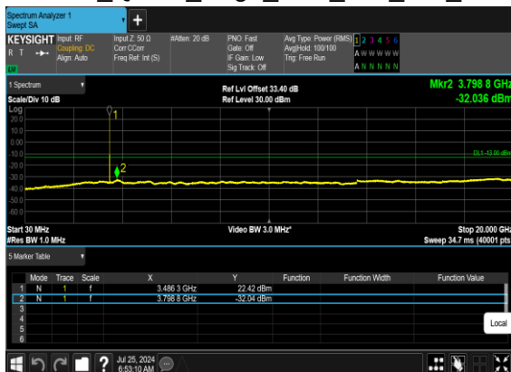
N78(30M)_DFT-s- OFDM_QPSK_Edge_1RB_Left_Mid_CH
