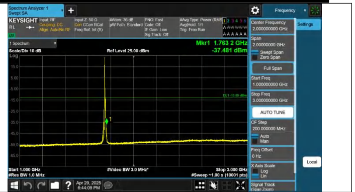
Band4-10MHz-QPSK-20350-1RB#0-1000~3000-PASS
