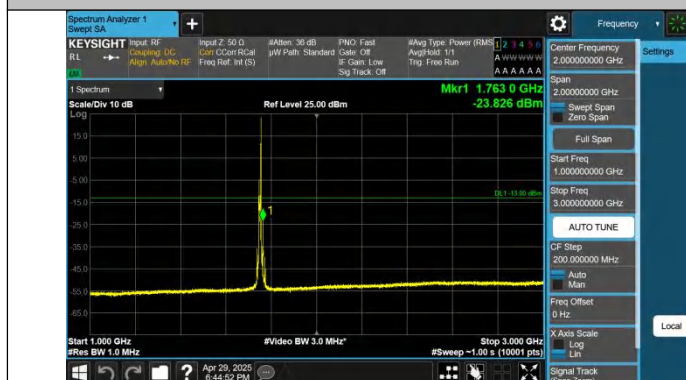
Band4-10MHz-QPSK-20350-1RB#49-1000~3000-PASS
