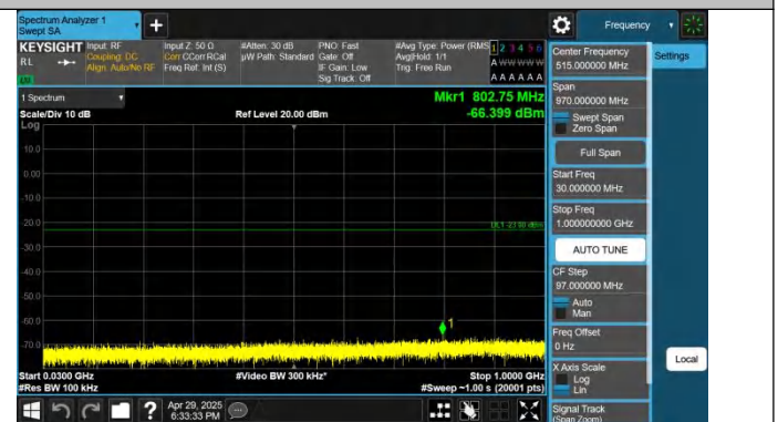
Band4-5MHz-QPSK-19975-1RB#24-30~1000-PASS
