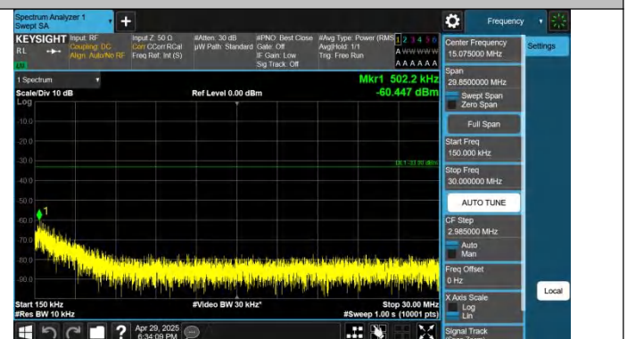
Band4-5MHz-QPSK-20175-1RB#0-0.15~30-PASS
