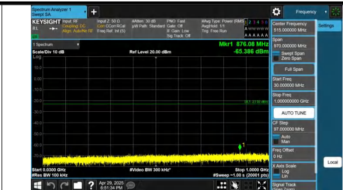
Band4-15MHz-QPSK-20175-1RB#74-30~1000-PASS
