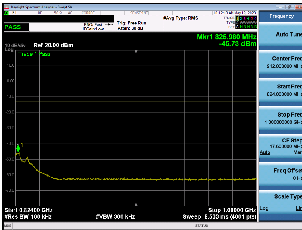
Plot 7-14. Conducted Spurious Plot (LTE Band 26 - 5MHz QPSK - RB Size 1, RB Offset 0 – Low Channel)
