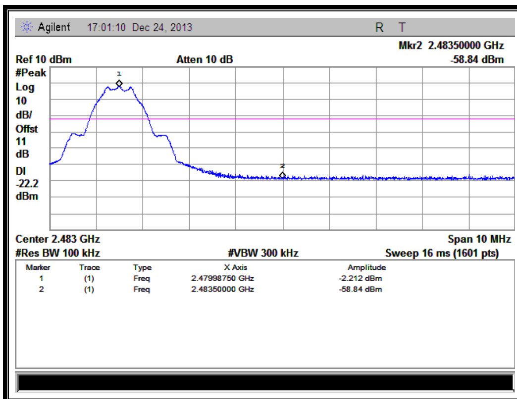
(Band Edge@ Channel = 39)
