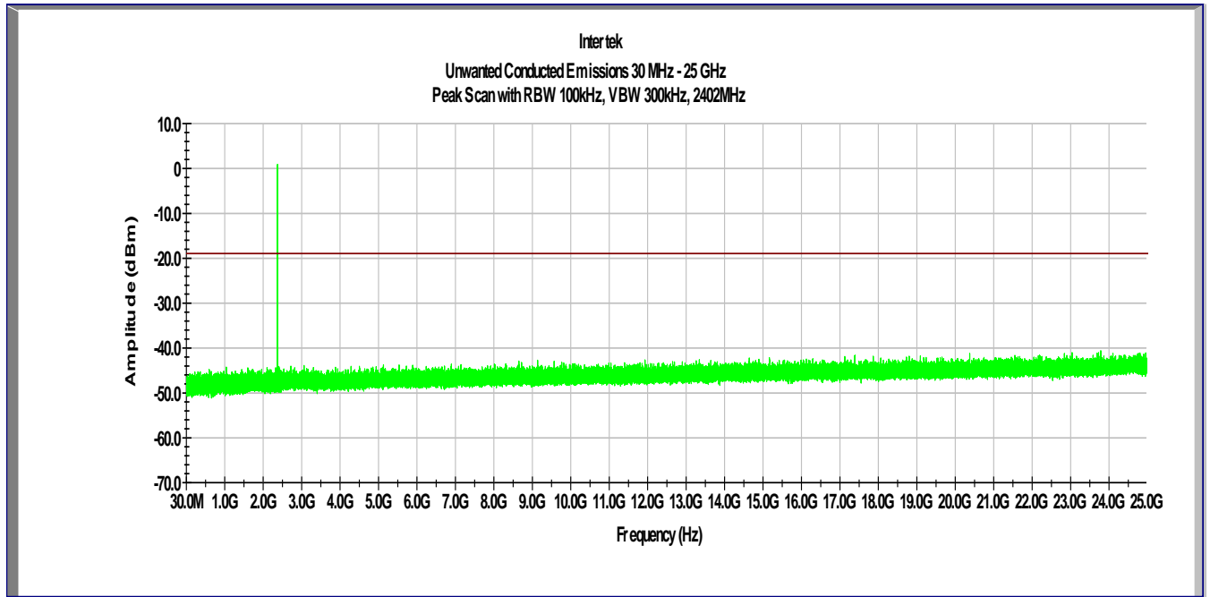
Tx @ Low Channel, 2402 MHz 30MHz -25GHz Conducted Spurious Plot 4.1
