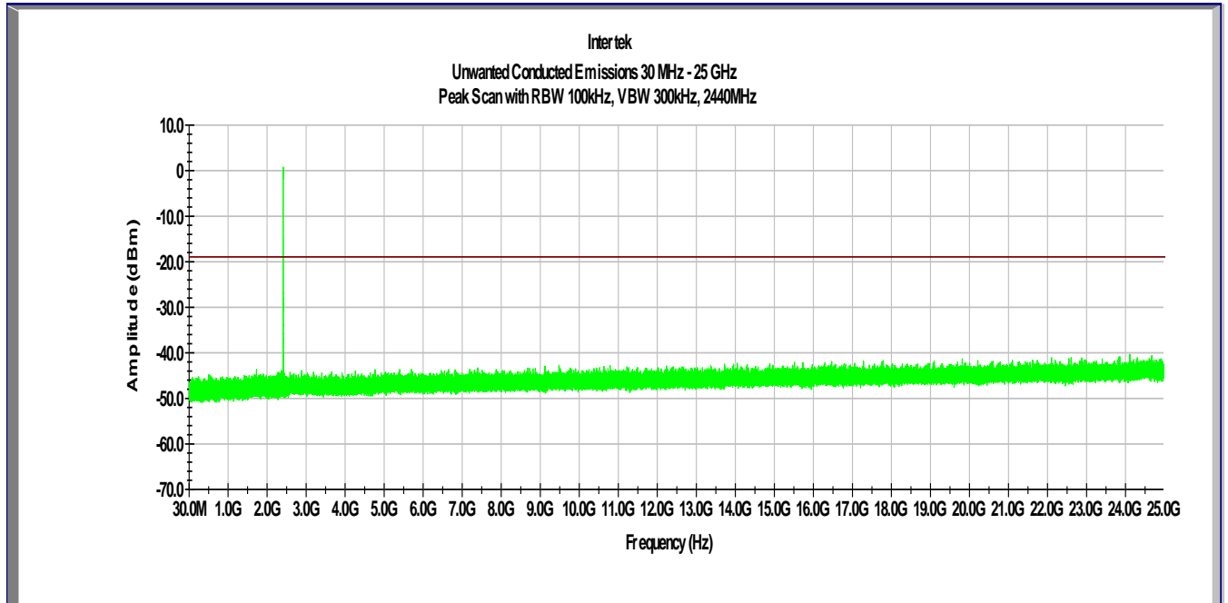
Tx @ Mid Channel, 2440 MHz 30MHz -25GHz Conducted Spurious Plot 4.2
