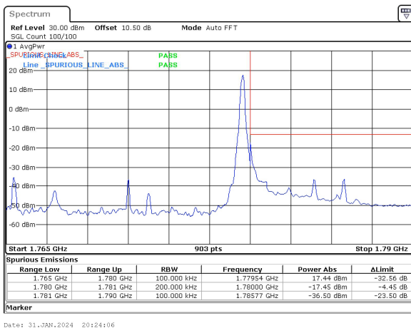
15MHz_15kHz_1772.5MHz_DFT-s-OFDM QPSK_RB1@78&amp;-17.45 dBm
