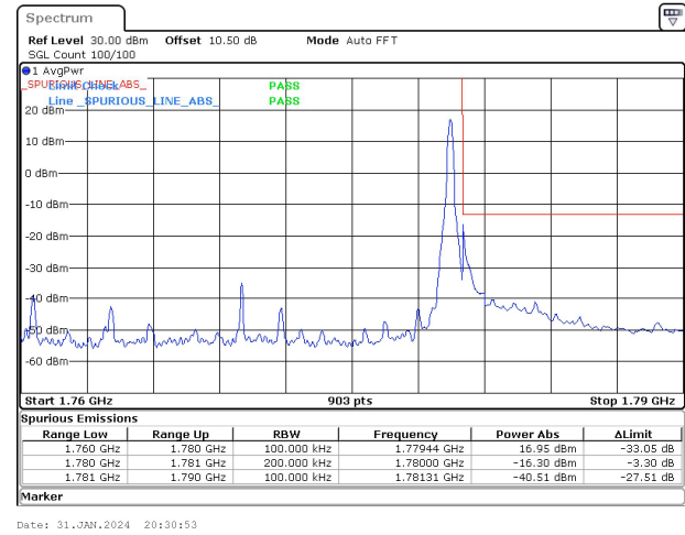
20MHz_15kHz_1770MHz_DFT-s-OFDM QPSK_RB1@105&-16.30 dBm
