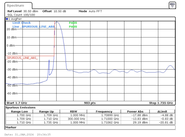
25MHz_15kHz_1722.5MHz_DFT-s-OFDM QPSK_RB1@0&-13.83 dBm
