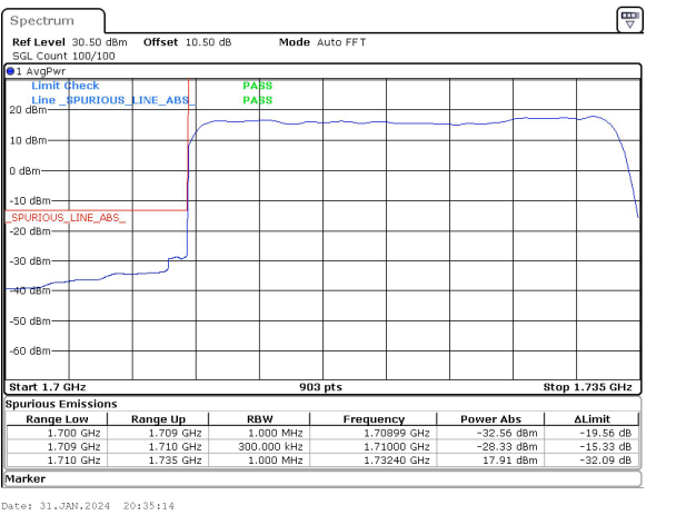
25MHz_15kHz_1722.5MHz_DFT-s-OFDM QPSK_RB128@0&-28.33 dBm
