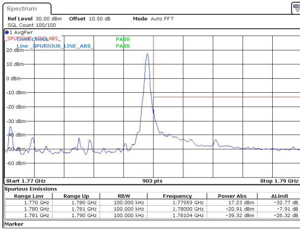
10MHz_15kHz_1775MHz_DFT-s-OFDM QPSK_RB1@51&amp;-20.91 dBm
