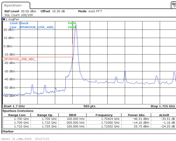
15MHz_15kHz_1717.5MHz_DFT-s-OFDM QPSK_RB1@0&amp;-14.16 dBm
