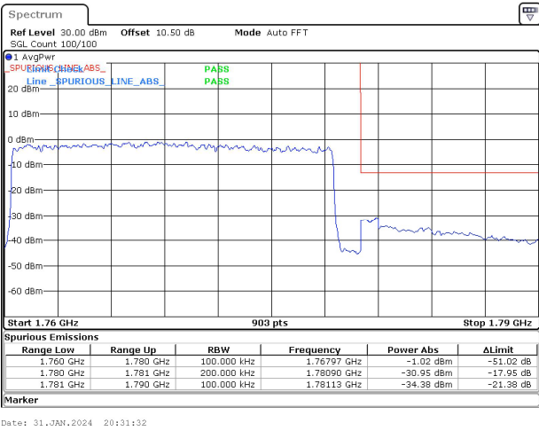
20MHz_15kHz_1770MHz_DFT-s-OFDM QPSK_RB100@0&-30.95 dBm
