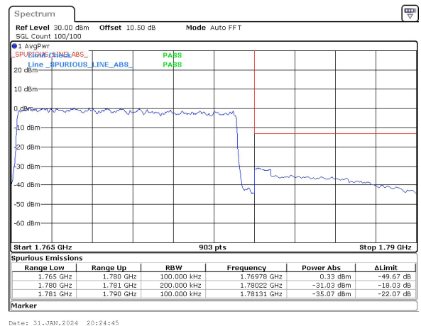
15MHz_15kHz_1772.5MHz_DFT-s-OFDM QPSK_RB75@0&amp;-31.03 dBm
