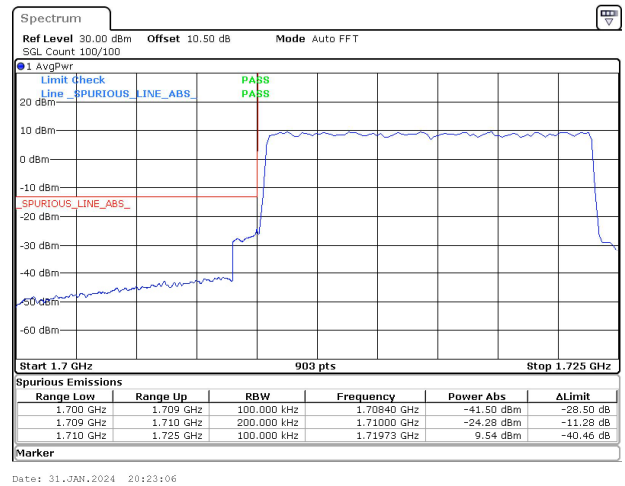
15MHz_15kHz_1717.5MHz_DFT-s-OFDM QPSK_RB75@0&amp;-24.28 dBm
