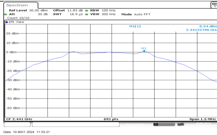
SRD 2.4G_Ant1_2441_0~Reference
