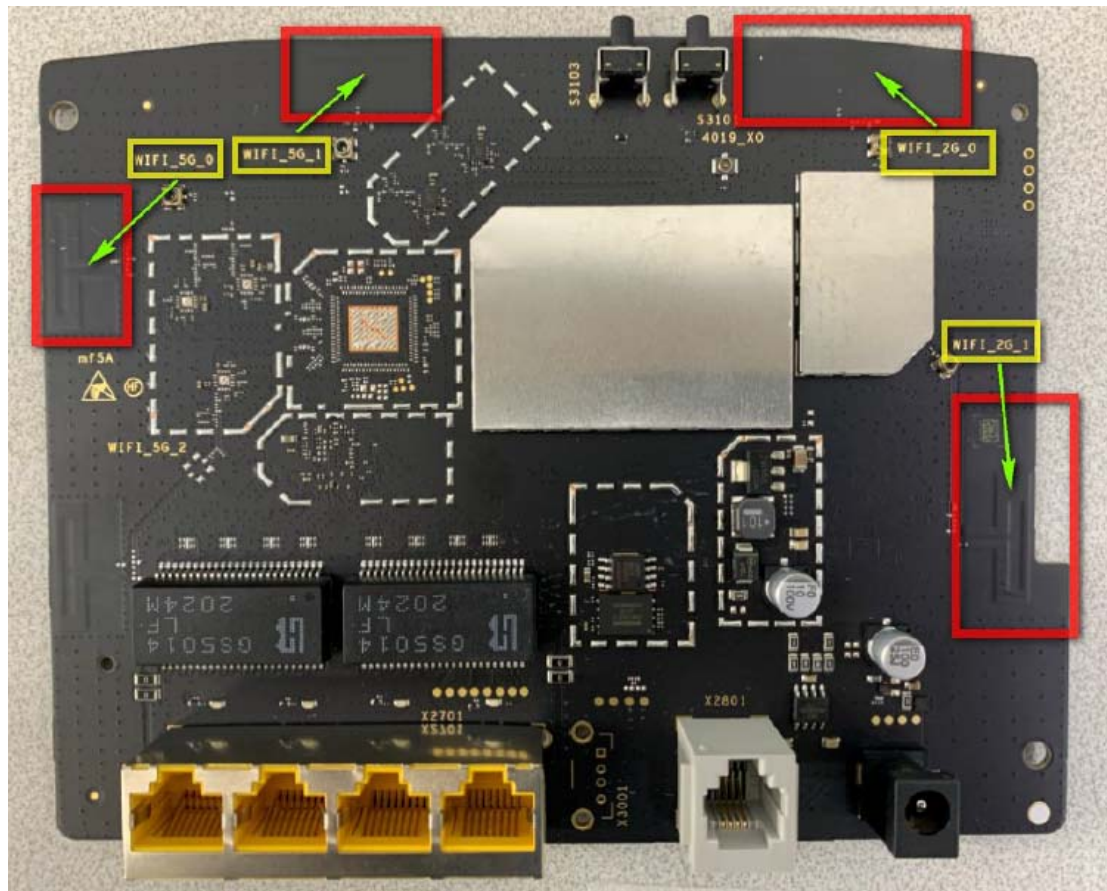
Antenna location
