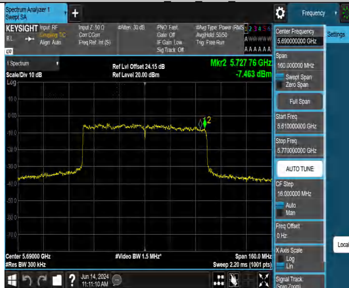
11AX80MIMO Ant4 5690 UNII-3
