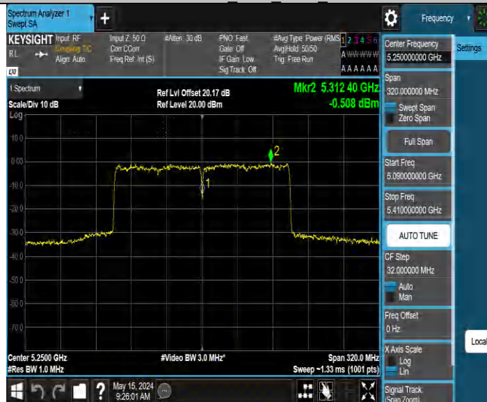
11AX160MIMO Ant4 5250 UNII-2A
