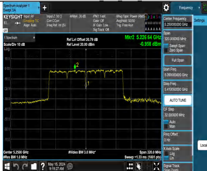
11AC160MIMO Ant4 5250 UNII-1
