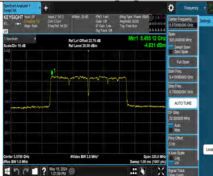
11AC160MIMO Ant2 5570
