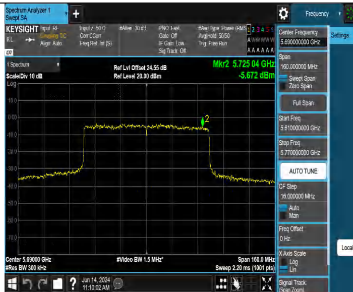
11AX80MIMO Ant2 5690 UNII-3
