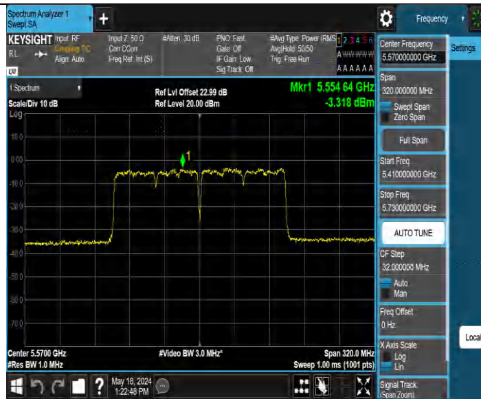
11AC160MIMO Ant3 5570
