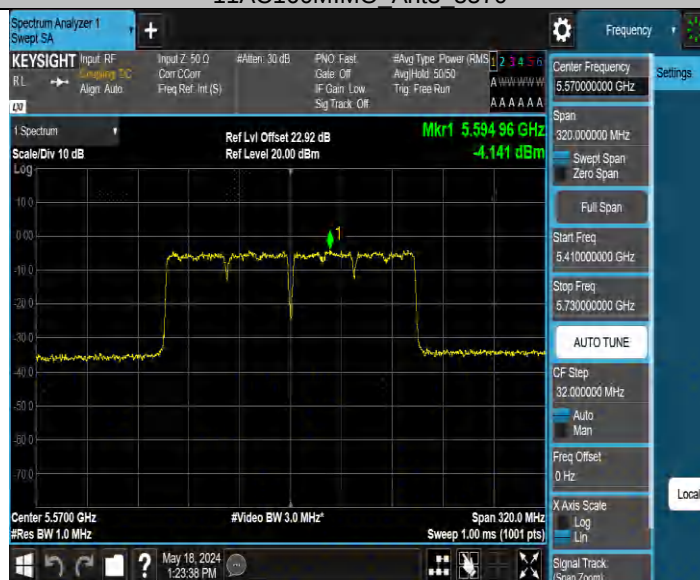
11AC160MIMO Ant4 5570
