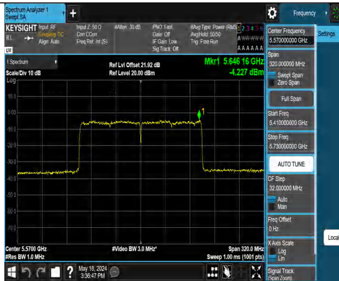
11AX160MIMO Ant4 5570
