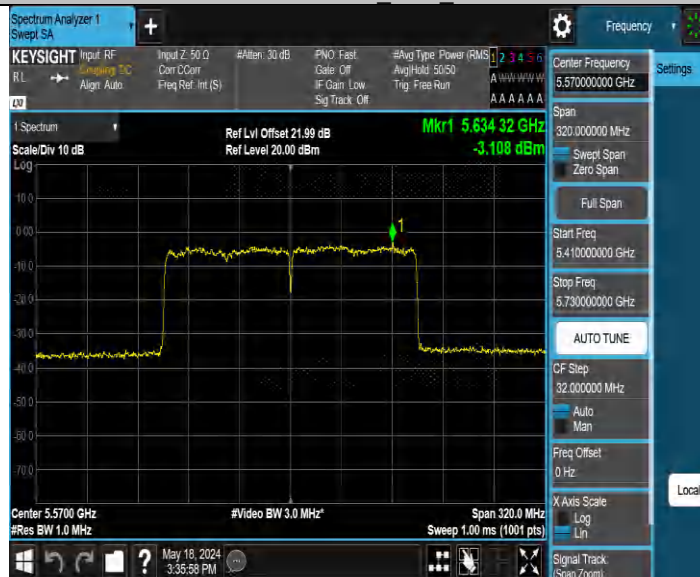
11AX160MIMO Ant3 5570
