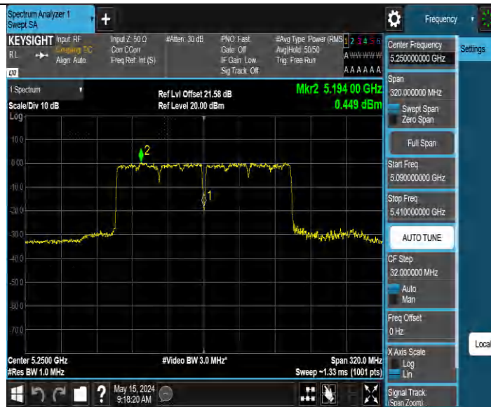
11AC160MIMO Ant2 5250 UNII-1
