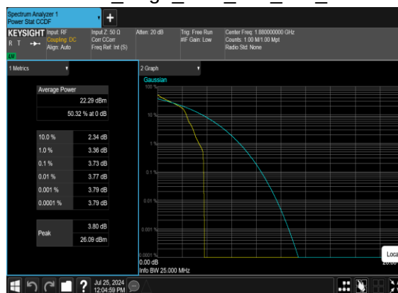
N2(20M)_DFT-s-OFDM_PI_2- BPSK_Edge_1RB_Left_Mid_CH
