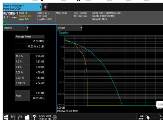
N2(20M)_DFT-s- OFDM_QPSK_Edge_1RB_Left_Mid_CH
