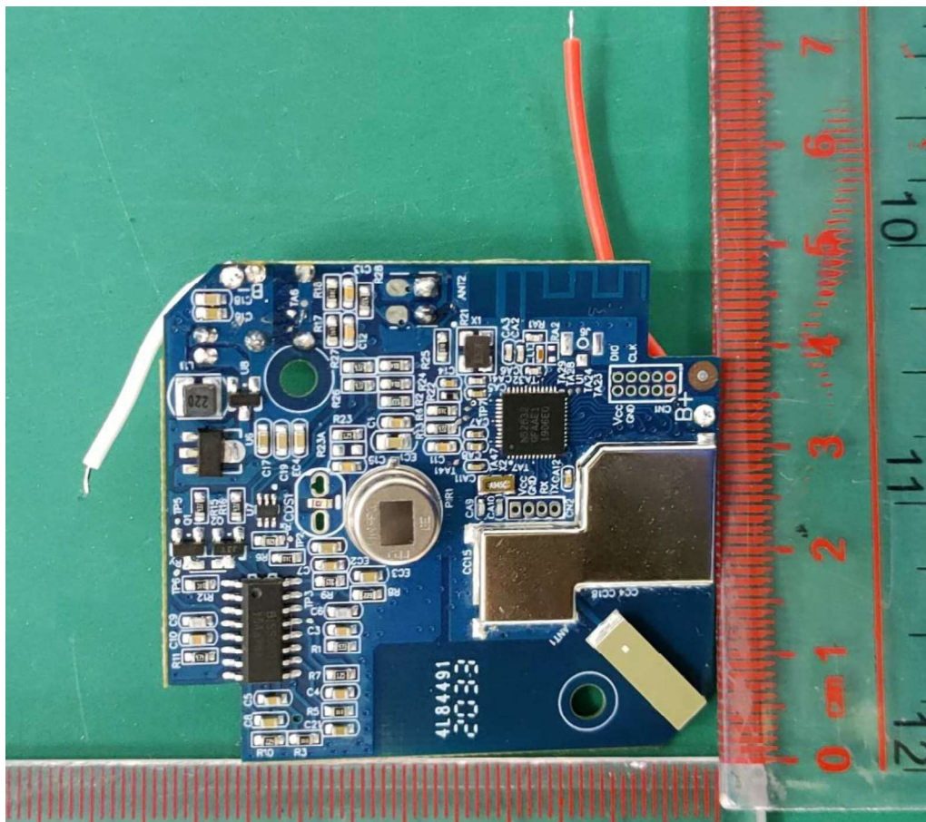
Photograph 4: PCB of the EUT
