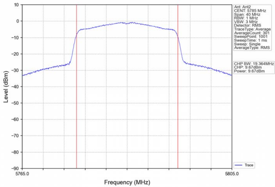
802.11ax(HEW20)_MCH_5785MHz_RU242_Left_Ant2_NTNV
