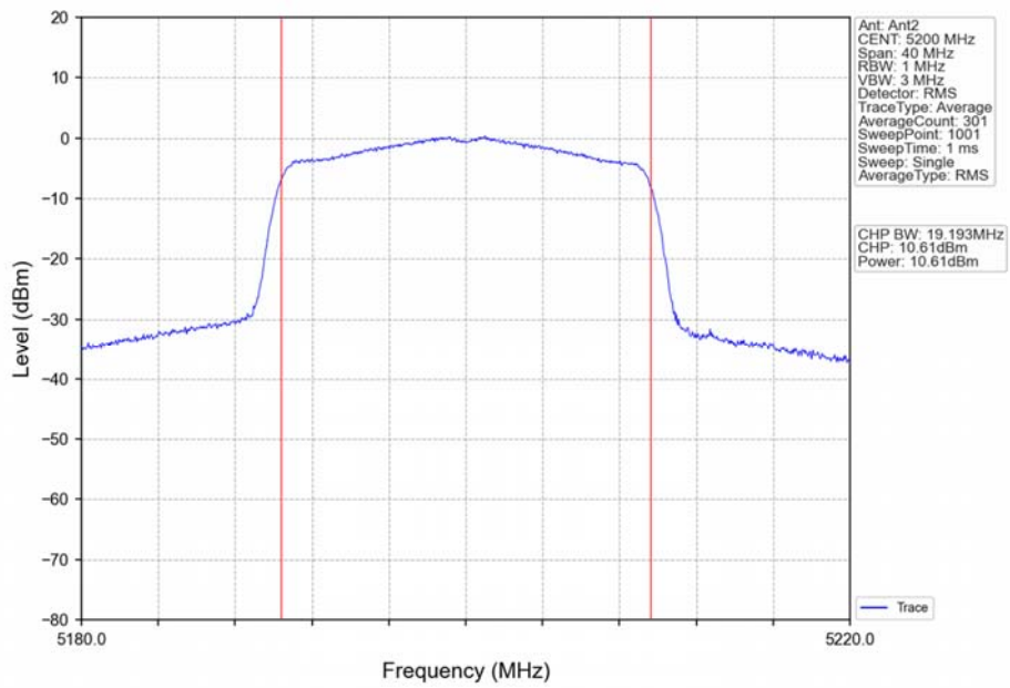
802.11ax(HEW20)_MCH_5200MHz_RU242_Left_Ant2_NTNV
