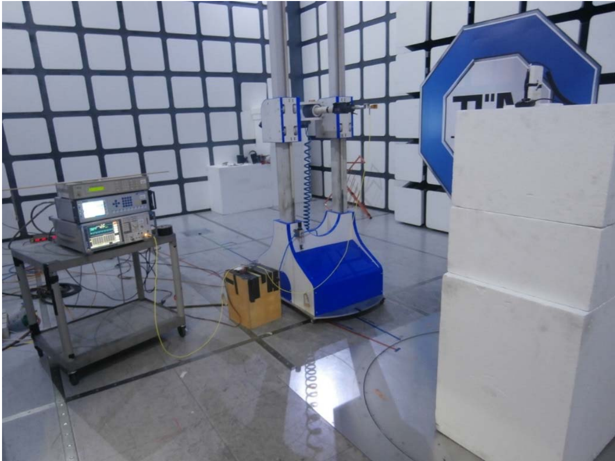
FCC Part 15.407 Radiated Emissions 18 GHz to 25 GHz
