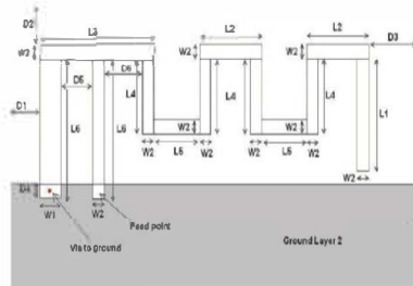
Figure 1: Antenna Dimensions
