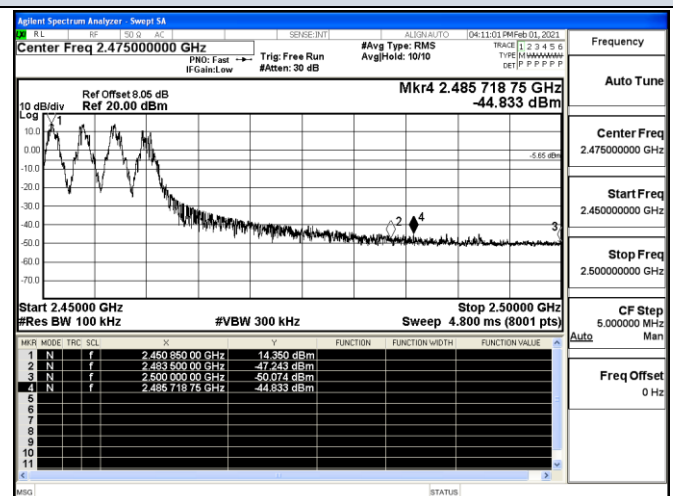
Channel 15 / 2460 MHz
