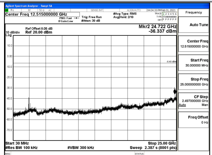
Channel 15 / 2460 MHz
