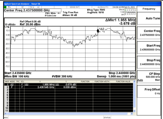
Channel 7 / 2436 MHz
