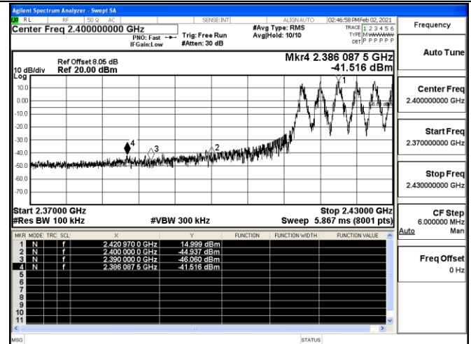
Channel 0 / 2415 MHz
