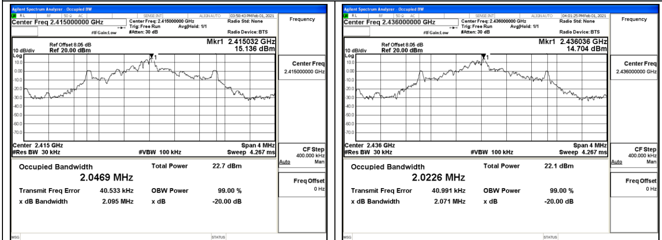
Channel 0/ 2415Hz
