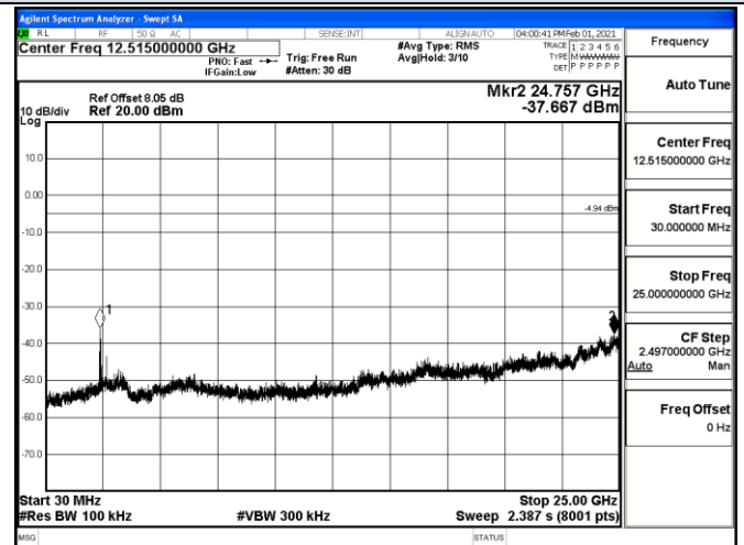
Channel 0 / 2415 MHz
